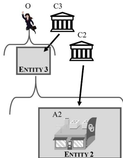
FIGURE 4. Structural Priority
