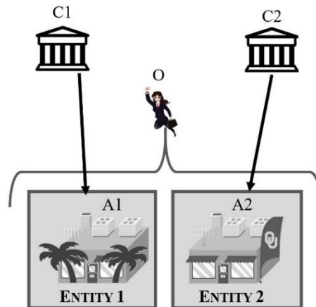
FIGURE 2. Entity Partitioning
