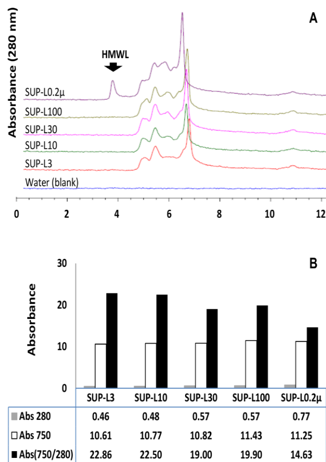
Figure 4. Characterization of size fractionated soluble lignin moieties from Eucalyptus . (A) Aqueous size exclusion chromatography profile of lignin samples containing water-soluble lignin moieties \leq 3 kDa (SUP-L3), \leq 10 kDa (SUP-L10), \leq 30 kDa (SUP-L30), \leq 100 kDa (SUP-L100) and \leq 0.2 \mu\text{m} (SUP-L0.2 \mu ). (B) Ferricyanide analysis of each substrate described in (A). Prussian blue produced from each reaction was estimated at 750 nm wavelength ( \text{Abs}_{750} ). The absorbance of each substrate was determined at 280 nm wavelength ( \text{Abs}_{280} ) prior to the analysis. Ferricyanide activity of each sample was normalized per unit substrate absorbance at 280 nm ( \text{Abs}_{750/280} ). HMWL = High molecular weight lignin moieties.
