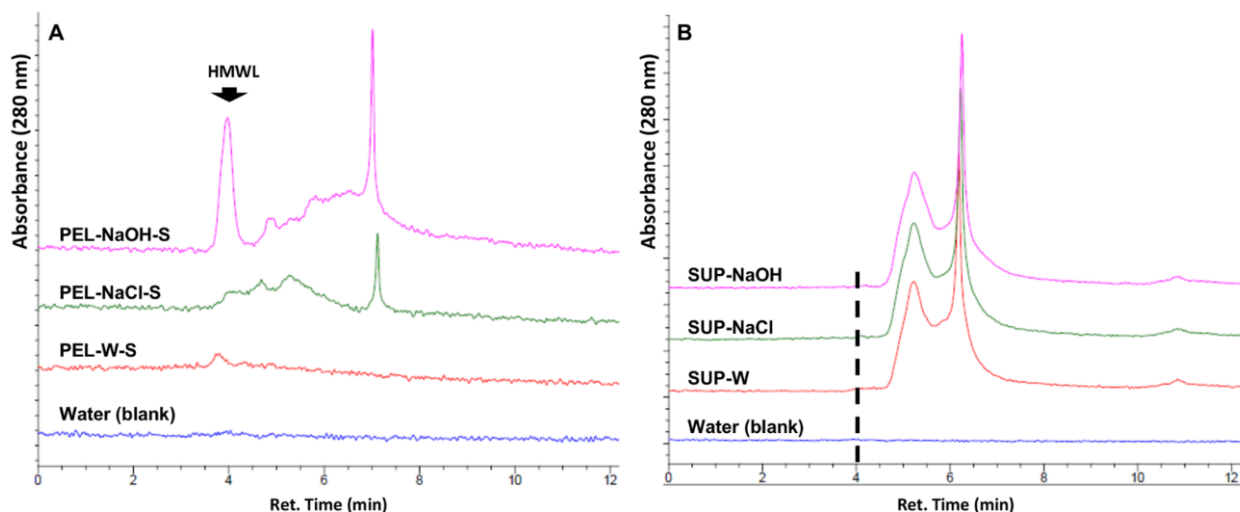
Figure 6. Size exclusion chromatography (SEC) analysis of alkaline solubilized sequestered lignin moieties from Eucalyptus . (A) SEC profile of 0.45 µm filtered supernatants of insoluble lignin aggregates (PEL) treated with DI-water (PEL-W-S), 0.01 M NaCl (PEL-NaCl-S) and 0.01 M NaOH (PEL-NaOH-S). Each PEL suspension was incubated at 37°C for 180 min. After incubation PEL-NaOH was neutralized with 0.01 M HCl. Sequestered soluble high molecular weight lignin (HMWL) moieties (Ret. Time = 3.5 – 4.5 min) were released from NaOH-treated aggregates. (B) SEC profile of the soluble lignin fractions (SUP) of the total lignin suspension (TLS) that was used for the preparation of the corresponding PEL fraction in (A). The broken line corresponded to the retention time of alkali solubilized high molecular weight lignin moieties released by NaOH treatment.
