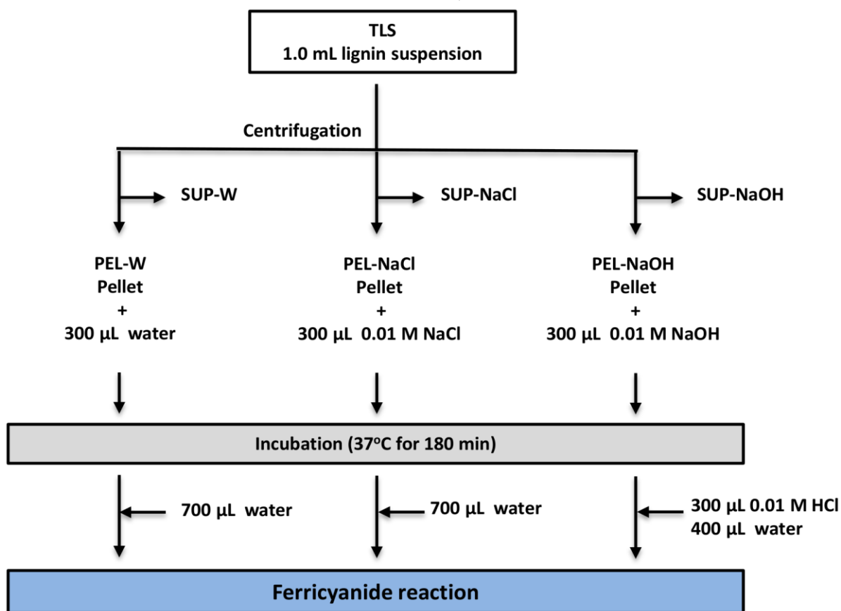
Figure 5. Schematic diagram of protocol for dissolution of insoluble lignin aggregates from Eucalyptus . Three 1.0 mL aliquots of aqueous total lignin suspension (TLS) were centrifuged to separate soluble lignin moieties (SUP) from insoluble aggregates (PEL). The SUP fractions were filtered through 0.45 \mu\text{m} membrane filter. The PEL extracts were washed three times by re-suspending in 1.0 mL of DI-water and centrifuging to remove residual soluble lignin moieties. The washed PEL extracts were re-suspended in 300 \mu\text{L} of DI-water (PEL-W), 300 \mu\text{L} of 0.01 M NaCl (PEL-NaCl) and 300 \mu\text{L} of 0.01 M NaOH (PEL-NaOH) respectively, and incubated in a water-bath at 37°C for 180 min with intermittent agitation. PEL-NaOH suspension was neutralized with 0.01 M HCl after incubation. The volume of each treated PEL suspensions were subsequent adjusted to 1.0 mL with DI-water. The soluble fraction of the treated PEL suspensions were also obtained from 0.5 mL aliquot of each sample and filtered through 0.45 \mu\text{m} membrane filter. The treated PEL extracts, the corresponding SUP (SUP-W, SUP-NaCl and SUP-NaOH) and the TLS were subjected to ferricyanide assay and size exclusion chromatography.
