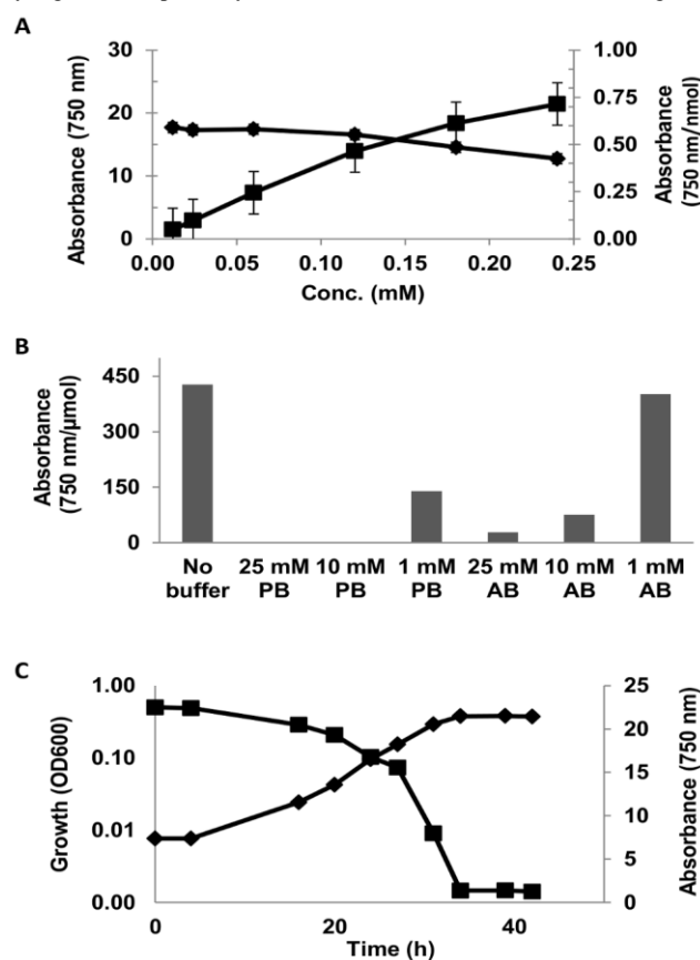
Figure 1. Ferricyanide assay characterization of syringic acid. (A) Plot of absorbance (750 nm) of ferricyanide reaction with different concentrations of syringic acid (activity) against normalized activity per nmol of substrate [Absorbance (750nm/ nmol)]. (B) Effect of 1, 10 and 25 mM phosphate (pH = 6.5) and acetate (pH = 5.5) buffers on ferricyanide reactivity of 0.05 mg/ml syringic acid and (C) Ferricyanide reactivity of residual substrate during growth of Syringobium sp. SYK-6 on 0.5 g/L syringic acid. OD_{600} = light scattering at 600 nm wavelength.
