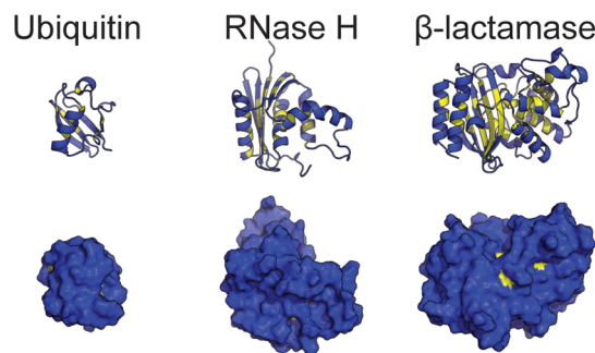
Figure 1. Structures of ubiquitin, RNase H, and \beta -lactamase in ribbon (top) and surface (bottom) representations. Surface residues are blue, and core residues are yellow.
