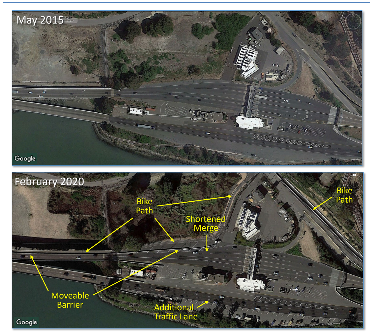
Figure 2-18: Modification of Richmond Approach
