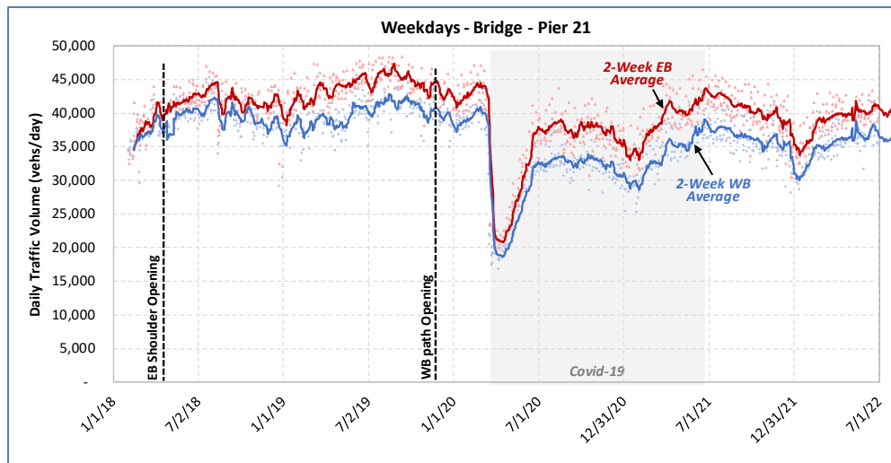
Figure 8-4: Traffic Volumes on Bridge – Weekdays, 2018-2022
