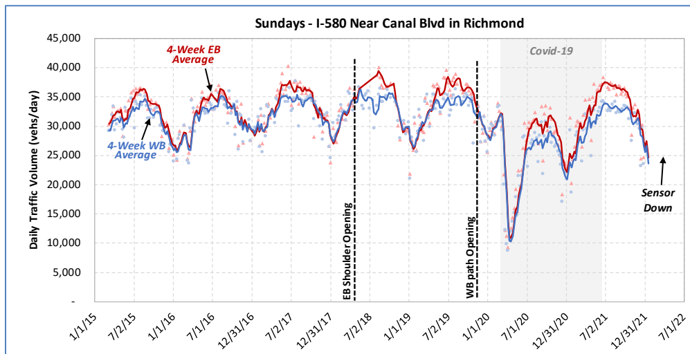
Figure 8-3: Traffic Volumes on I-580 near Canal Boulevard in Richmond – Sundays, 2015-2022
