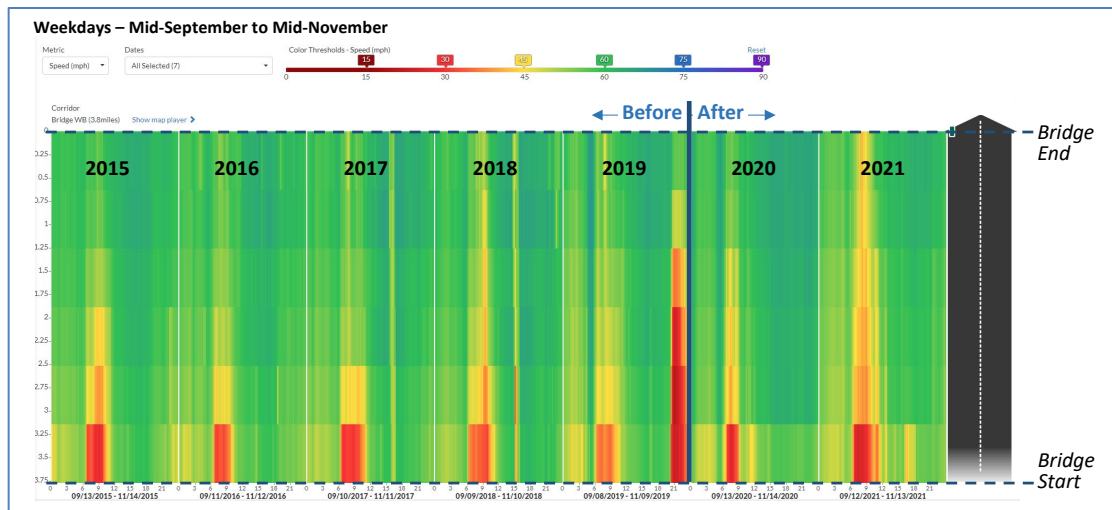
Figure 8-60: Speed Maps – I-580 West – Bridge – Weekdays, Fall 2015-2021
