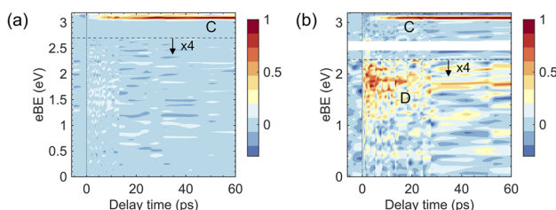
FIG. 6. Contour plots of TRPE spectra of I^-2TU photodetached by 3.18 eV with excitation energies of (a) 4.16 eV and (b) 4.73 eV. The signal intensities below 2.7 eV in (a) and 2.28 eV in (b) are magnified by a factor of 4.
