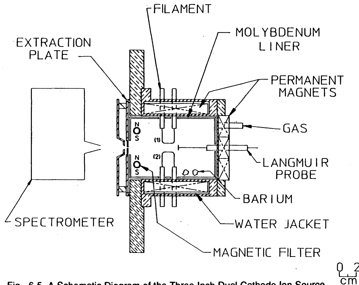
Fig. 6-5 A Schematic Diagram of the Three Inch Dual Cathode Ion Source
