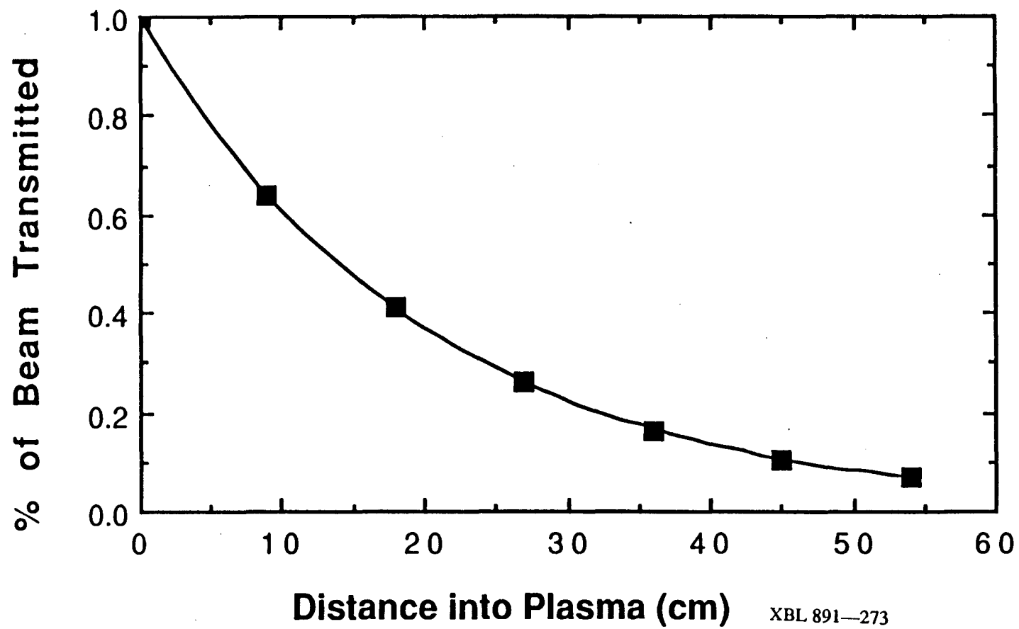
Fig. 4-1 Penetration of the TEXT Diagnostic Beam into the TEXT Plasma ( a=27 cm)
