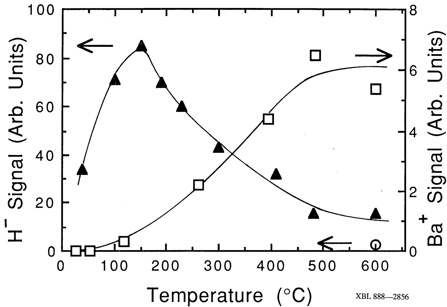
Fig. 6-4 A Graph of the H^- and Ba(+) Ion Signals as a Function of the Temperature of the Liner
