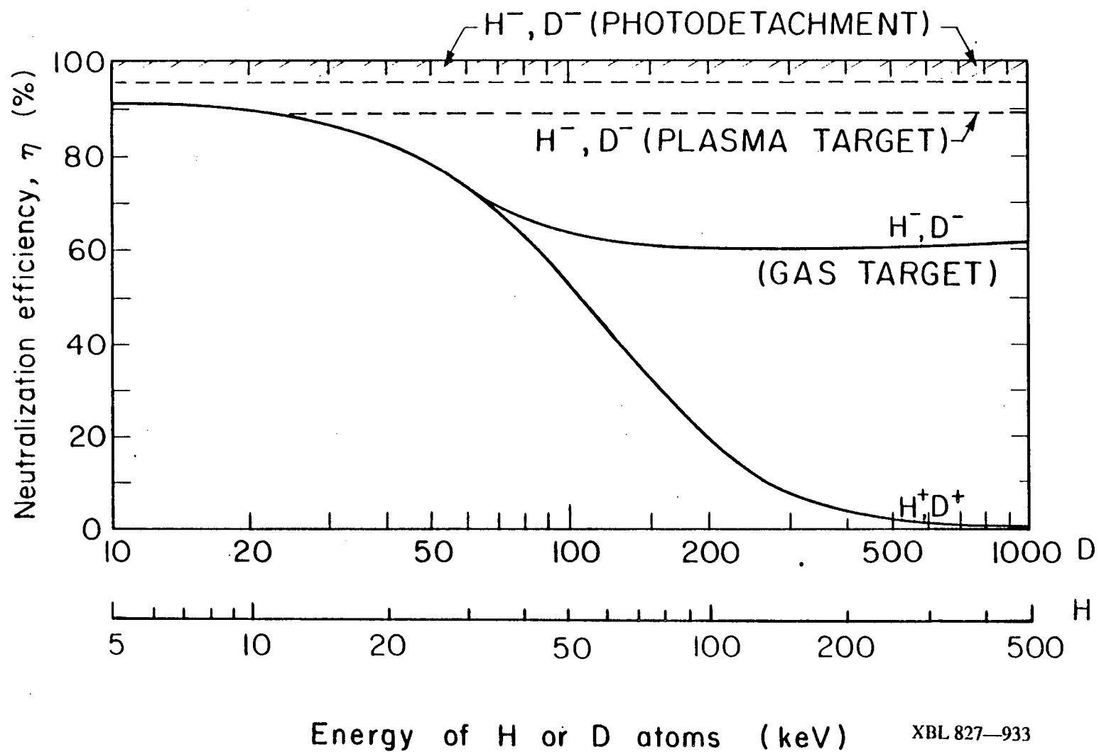
Fig. 1-2 Maximum Obtainable Neutral Fraction vs. Beam Energy
