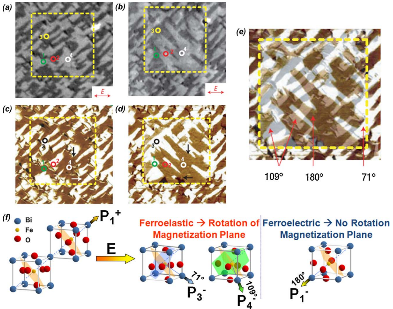
Fig. 28. Determination of strong magnetoelastic coupling in BiFeO 3 . Photomission electron microscopy (PEEM) images before (a) and after (b) electric field poling. The arrows show the X-ray polarization direction during the measurements. In-plane PFM images before (c) and after (d) electric field poling. The arrows show the direction of the in-plane component of ferroelectric polarization. Regions 1 and 2 (marked with green and red circles, respectively) correspond to 109° ferroelectric switching, whereas 3 (black and yellow circles) and 4 (white circles) correspond to 71° and 180° switching, respectively. In regions 1 and 2 the PEEM contrast reverses after electrical poling. (e) A superposition of in-plane PFM scans shown in c and d used to identify the different switching mechanisms that appear with different colors and are labeled in the figure. (Adapted from Ref. [381].) (f) Schematic illustration of coupling between ferroelectricity and antiferromagnetism in BiFeO 3 . Upon electrically switching BiFeO 3 by the appropriate ferroelastic switching events (i.e., 71° and 109° changes in polarization) a corresponding change in the nature of antiferromagnetism is observed. (Adapted from Ref. [285].) (For interpretation of the references to colour in this figure legend, the reader is referred to the web version of the article.)
