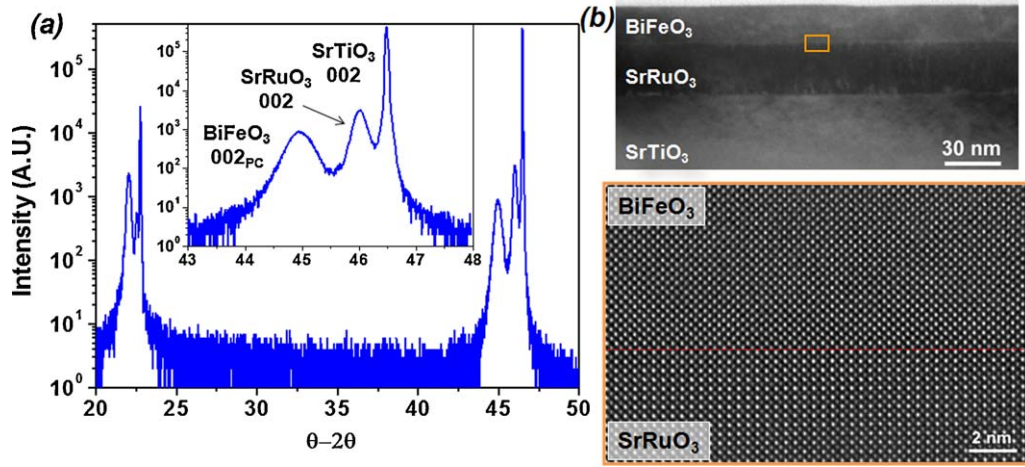
Fig. 25. Thin films of BiFeO 3 . (a) X-ray diffraction results from a fully epitaxial, single phase BFO/SRO/STO(0 0 1) heterostructure. (b) Low (top) and high (bottom) resolution transmission electron microscopy images of BFO/SRO/STO(0 0 1) heterostructure. (Adapted from Ref. [285].)
