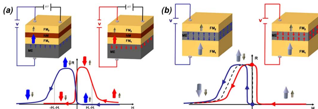
Fig. 32. Multiferroic-based magnetolectronics. (a) Schematic of the magnetoresistance curve of a GMR device involving a magnetoelectric, multiferroic film as a pinning layer. Half-hysteresis curves are shown, after saturation at positive field values. The change of polarity of the magnetoelectric, multiferroic layer upon application of an electric field changes the direction of the net magnetization of the pinning field. The pinned layer (FM1) switches first at large positive field (red), or second at large negative field (blue). The low field magnetic configuration is therefore either antiparallel (red) or parallel (blue), controlled by the magnetoelectric, multiferroic. (b) Schematic of the magnetoresistance curve of a TMR device involving a magnetoelectric, multiferroic film as a tunnel barrier. Half-hysteresis curves are shown, after saturation at positive field values. The arrows denote the magnetization directions, with the bottom layer FM1 being harder (or pinned) than the top one FM2. The dashed curve is the expected TMR behavior. The change of voltage polarity changes the direction of the net magnetization of the magnetoelectric, multiferroic layer, adding an exchange bias magnetic field to the resistance curve. The two colors indicate shifting of half-hysteresis curves towards positive or negative fields, depending on the polarity of the applied voltage. At zero magnetic field, the change of voltage polarity changes the resistance value of the device (dashed). (Adapted from Ref. [420].) (For interpretation of the references to colour in this figure legend, the reader is referred to the web version of the article.)
