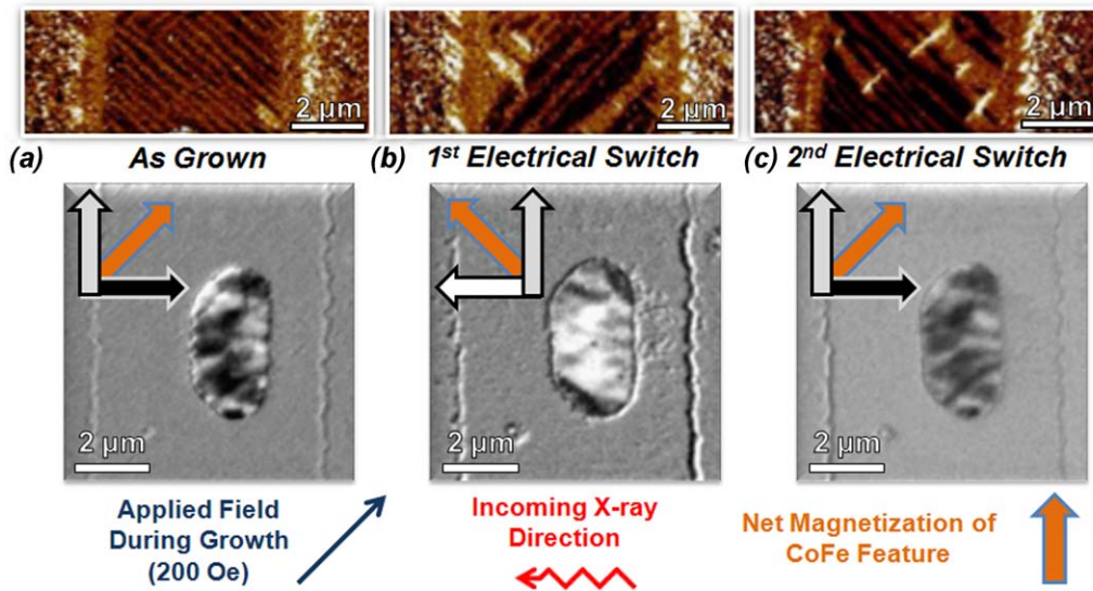
Fig. 38. Electric field control of ferromagnetic domain structures at room temperature. In-plane piezoresonance force microscopy images of ferroelectric domain structure (top) and corresponding photoemission electron microscopy image of ferromagnetic domain structure (bottom) of Co 0.9 Fe 0.1 features on BiFeO 3 as a function of applied electric field in the (a) as-grown state, (b) after application of an electric field, and (c) following application of the opposite electric field. This represents the first demonstration of reversible electric field control of ferromagnetic domain structures at room temperature. (Adapted from Ref. [441].)
