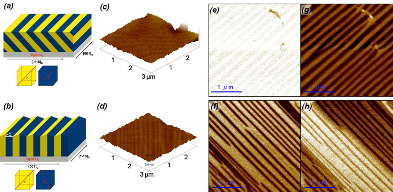
Fig. 16. Ordered arrays of ferroelectric domains and domain walls. (a) and (b) Schematics of equilibrium structure of an ordered array of 71^\circ and 109^\circ domain walls, respectively. (c) and (d) Surface topography as measured by AFM of 71^\circ and 109^\circ domain walls samples, respectively. Out-of-plane (e) and (f) as well as in-plane (g) and (h) PFM images for samples possessing ordered arrays of 71^\circ and 109^\circ domain walls. (Adapted from Ref. [135].)
