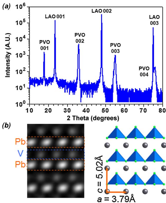
Fig. 30. Other multiferroics – \text{PbVO}_3 . (a) X-ray diffraction of a fully epitaxial \text{PbVO}_3/\text{LaAlO}_3 (0 0 1) thin film. (b) High resolution, cross-sectional transmission electron microscopy image of the \text{PbVO}_3 structure along with a schematic illustration of the large c/a lattice parameter distortion in this super tetragonal phase. (Adapted from Ref. [393].)
