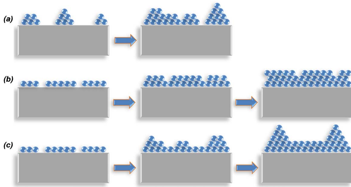
Fig. 3. Illustrations of the basic growth modes including (a) Volmer–Weber (island), (b) Frank–Van der Merwe (layer-by-layer), and (c) Stranski–Krastranov growth.
