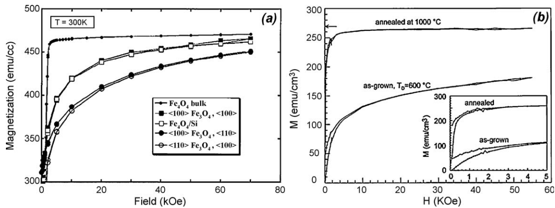
Fig. 19. Magnetism in spinel thin films. (a) Magnetization measured in the film plane for Fe 3 O 4 films grown on Si (1 0 0) and MgO (1 0 0) and (1 1 0). The crystallographic direction along which the field is applied is indicated beside each film in the figure. The magnetization axis is offset to facilitate observation of the high field data. (Adapted from Ref. [186].) (b) Magnetization of as-grown and post-annealed NiFe 2 O 4 thin films demonstrates the lengths to which one must go to achieve bulk-like properties in spinel films. (Adapted from Ref. [199].)
