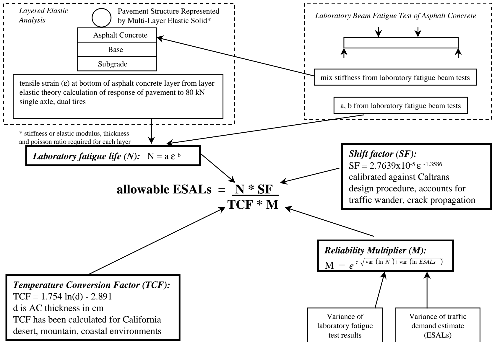
Figure 24. Fatigue Analysis Procedure.
