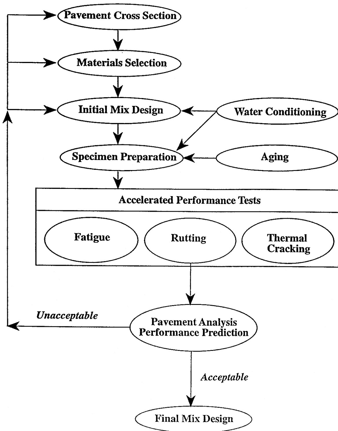
Figure 3. Schematic of Mix Design and Analysis Framework.
