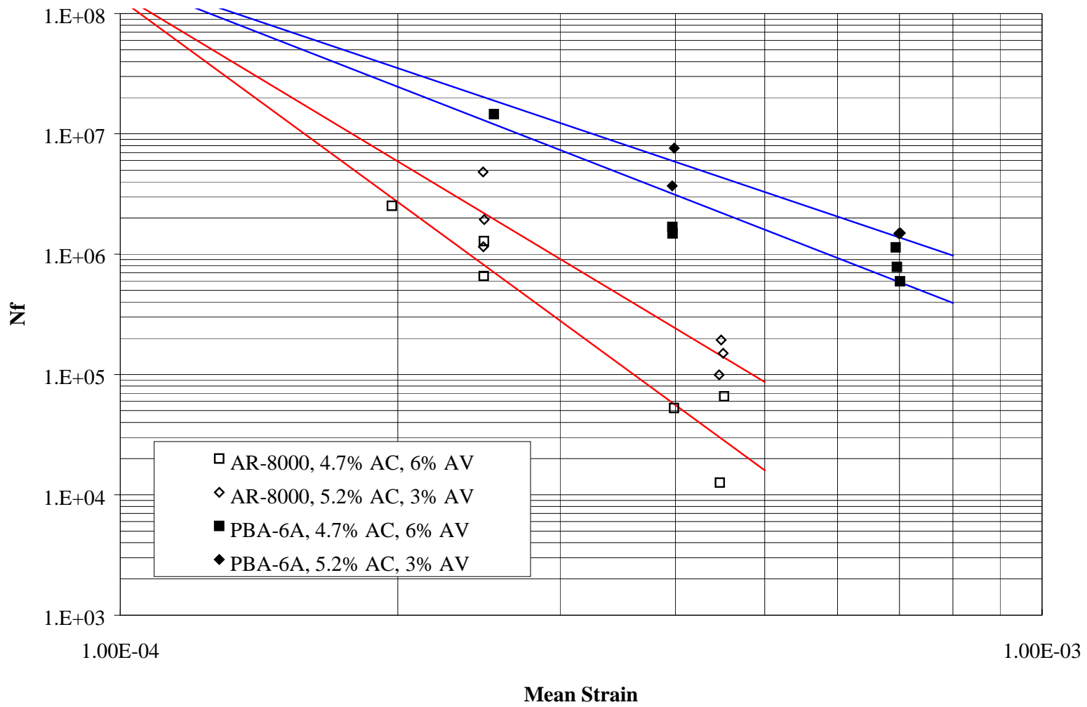
Figure 22. Results of Controlled Strain Fatigue Tests at 20°C, 10 Hertz Frequency.
