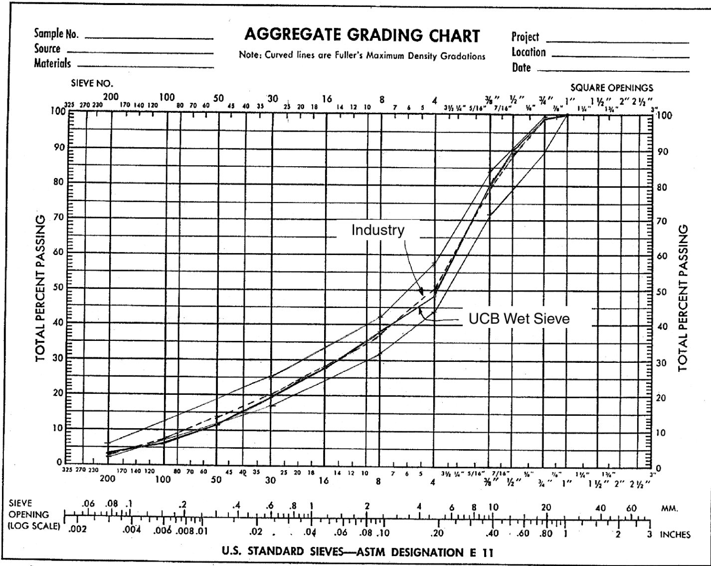
Figure 9. Comparison of UCB and Industry Gradations, Hot Bin Aggregates.
