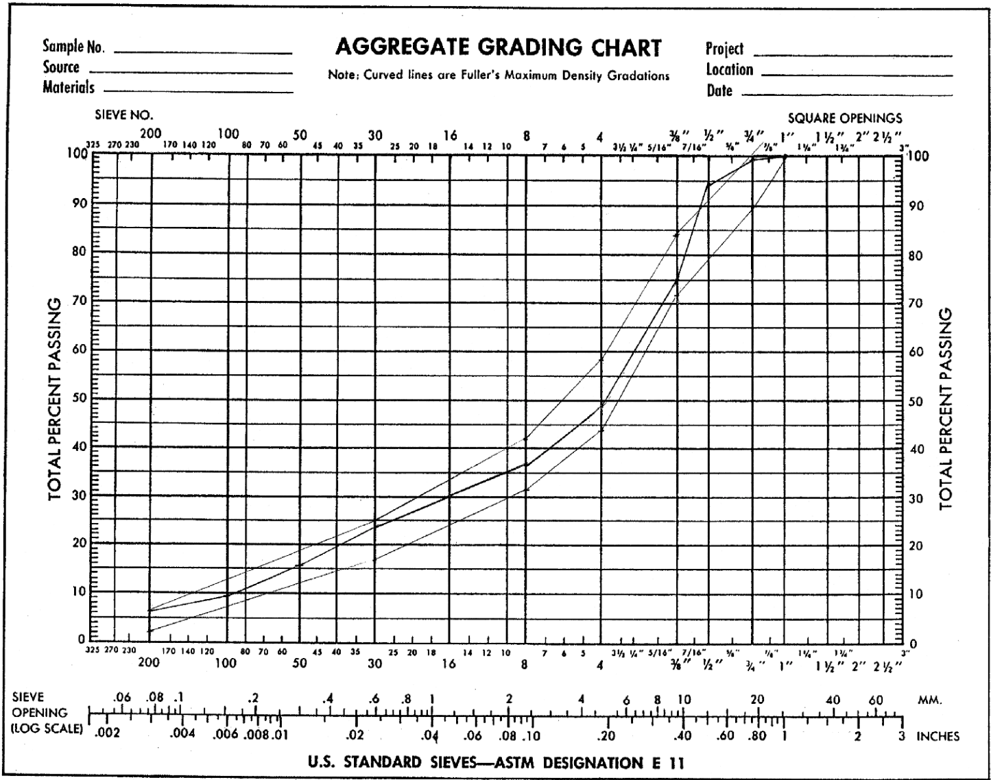
Figure 11. Aggregate Gradation with Crushed Cold Feed and Sands (16 Percent).
