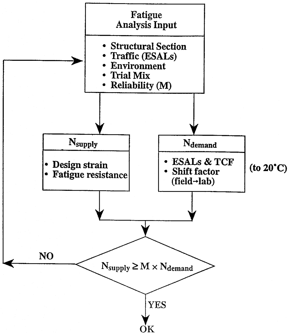
Figure 5. Fatigue System.
