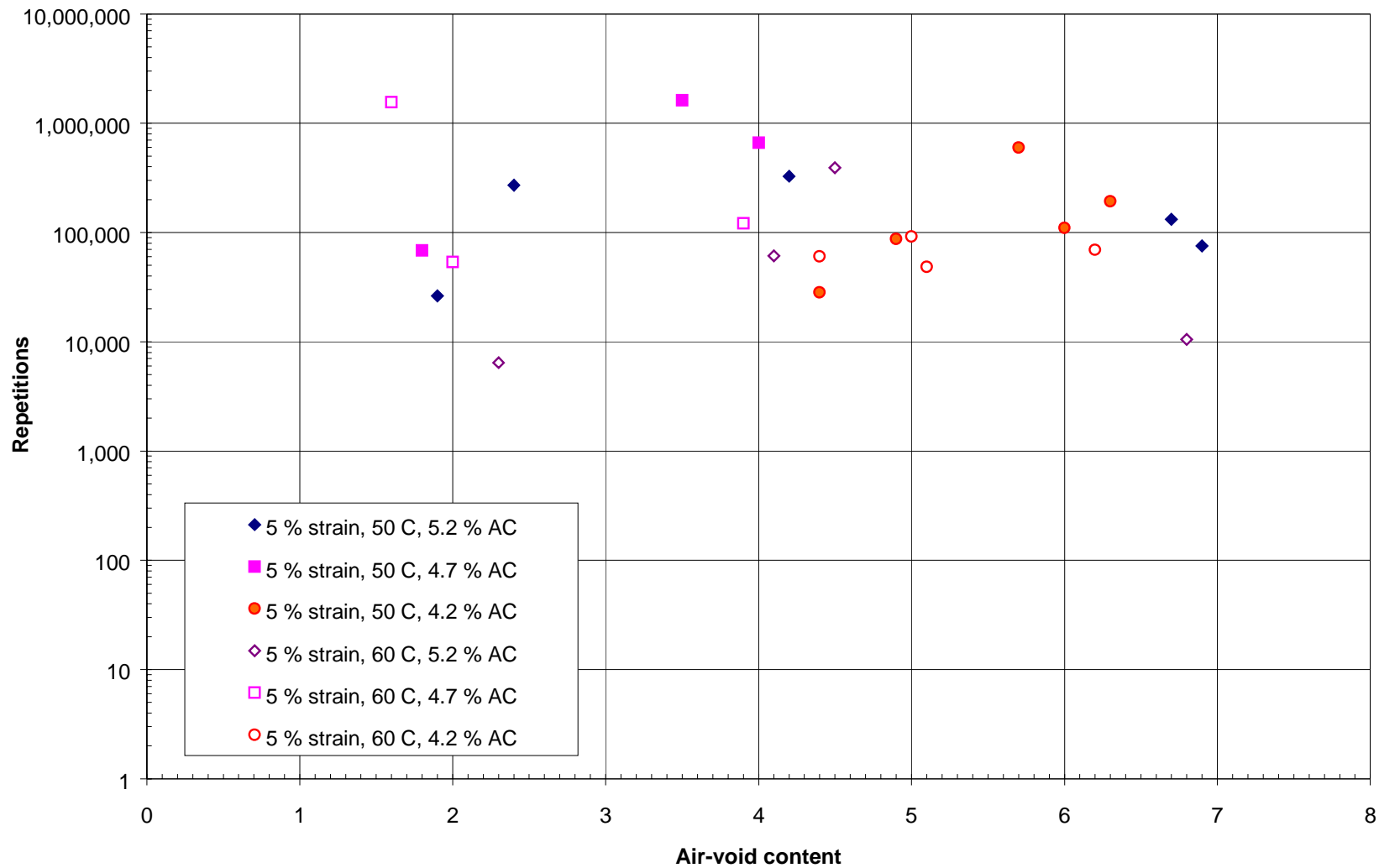
Figure 20. Relationship between Number of Repetitions to 5 Percent Permanent Shear Strain and Air-Void Content, Mixes with PBA-6A Binder.
