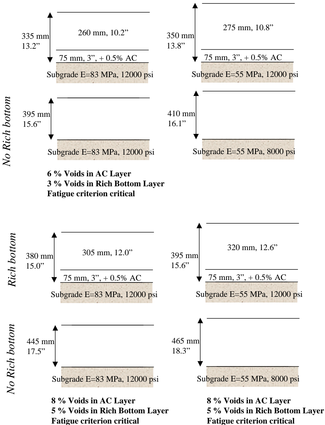
Figure 27a. Structural Sections for Valley Asphalt with Increasing Air-Void Contents.
