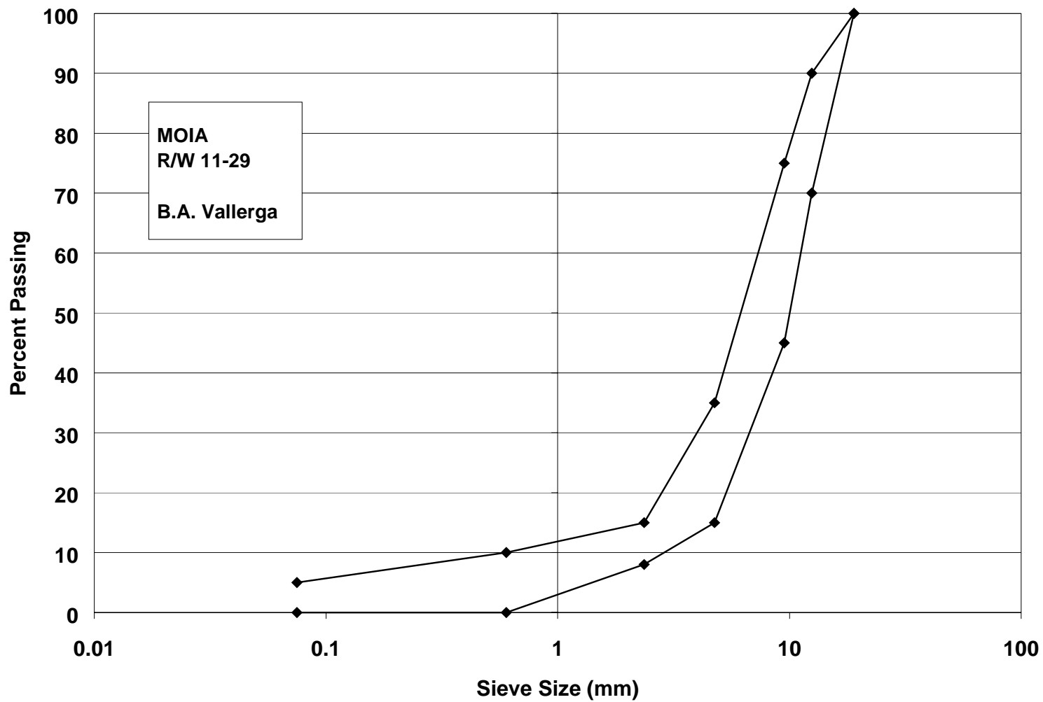
Figure 28. Open-Graded Aggregate Gradation (Porous Friction Course).
