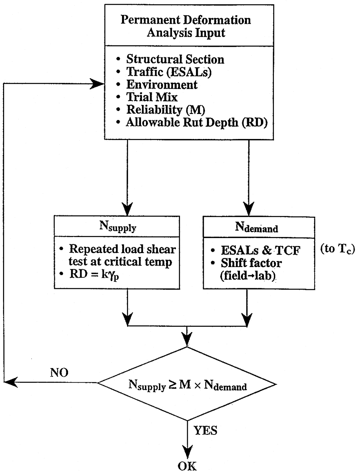
Figure 4. Permanent Deformation System.
