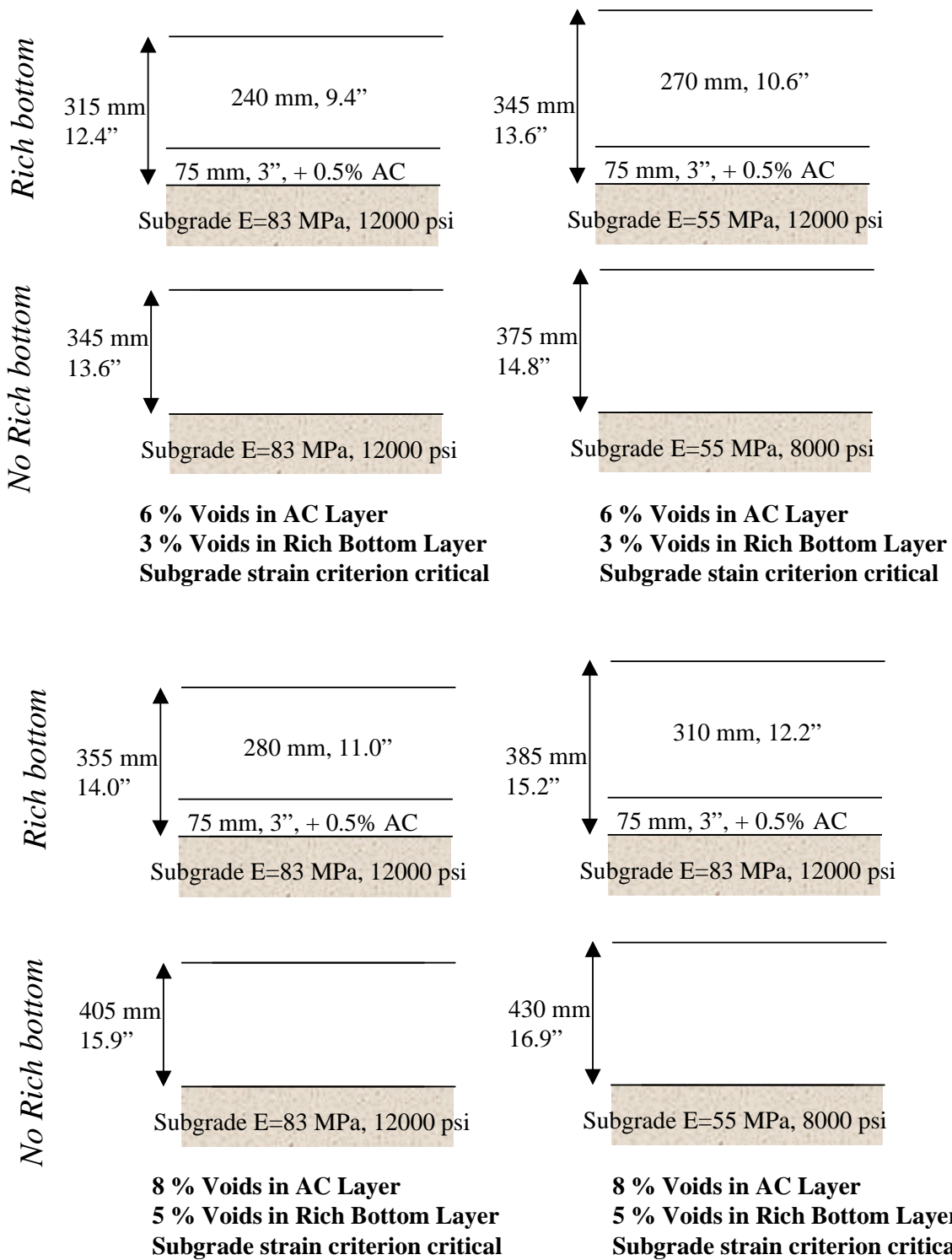
Figure 27b. Structural Sections for Coastal Asphalt with Increasing Air-Void Contents.
