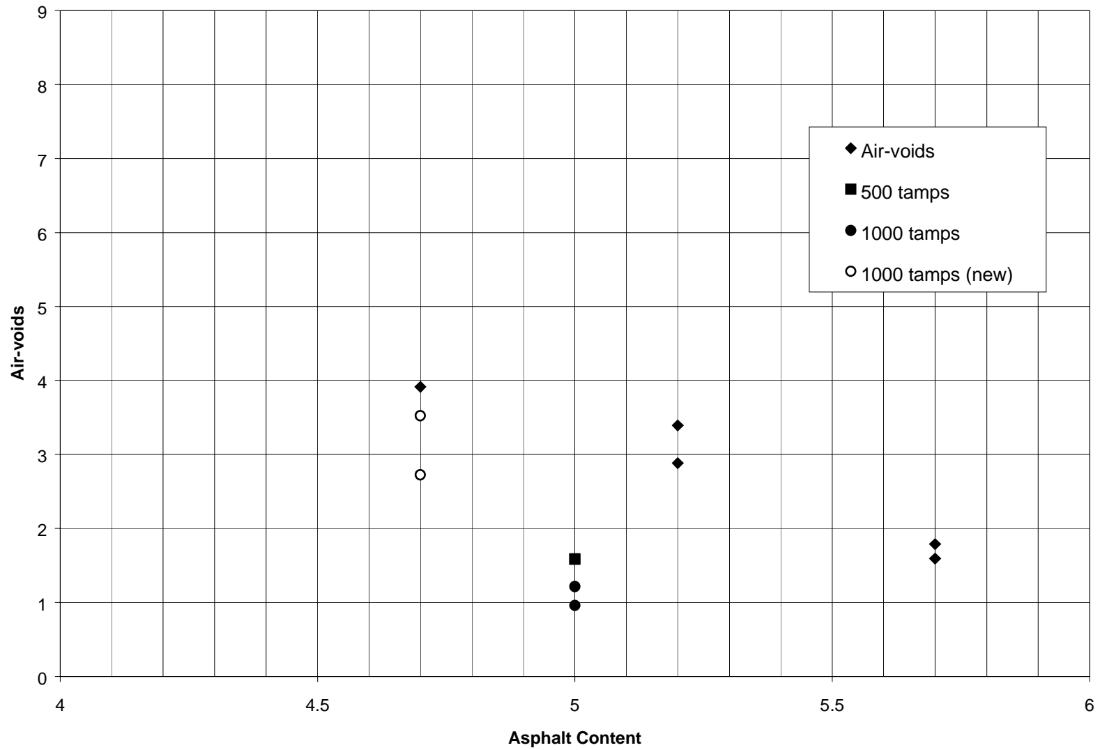
Figure 16. Air-Void Content versus Asphalt Content, PBA-6A Binder.
