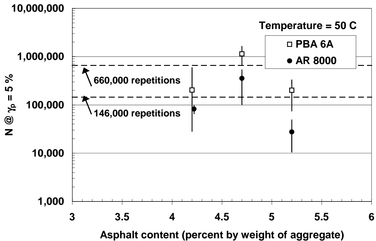
Figure 23. Repetitions to 5 Percent Permanent Shear Strain, N_{supply} , Versus Binder Content; Tests at 50°C.
