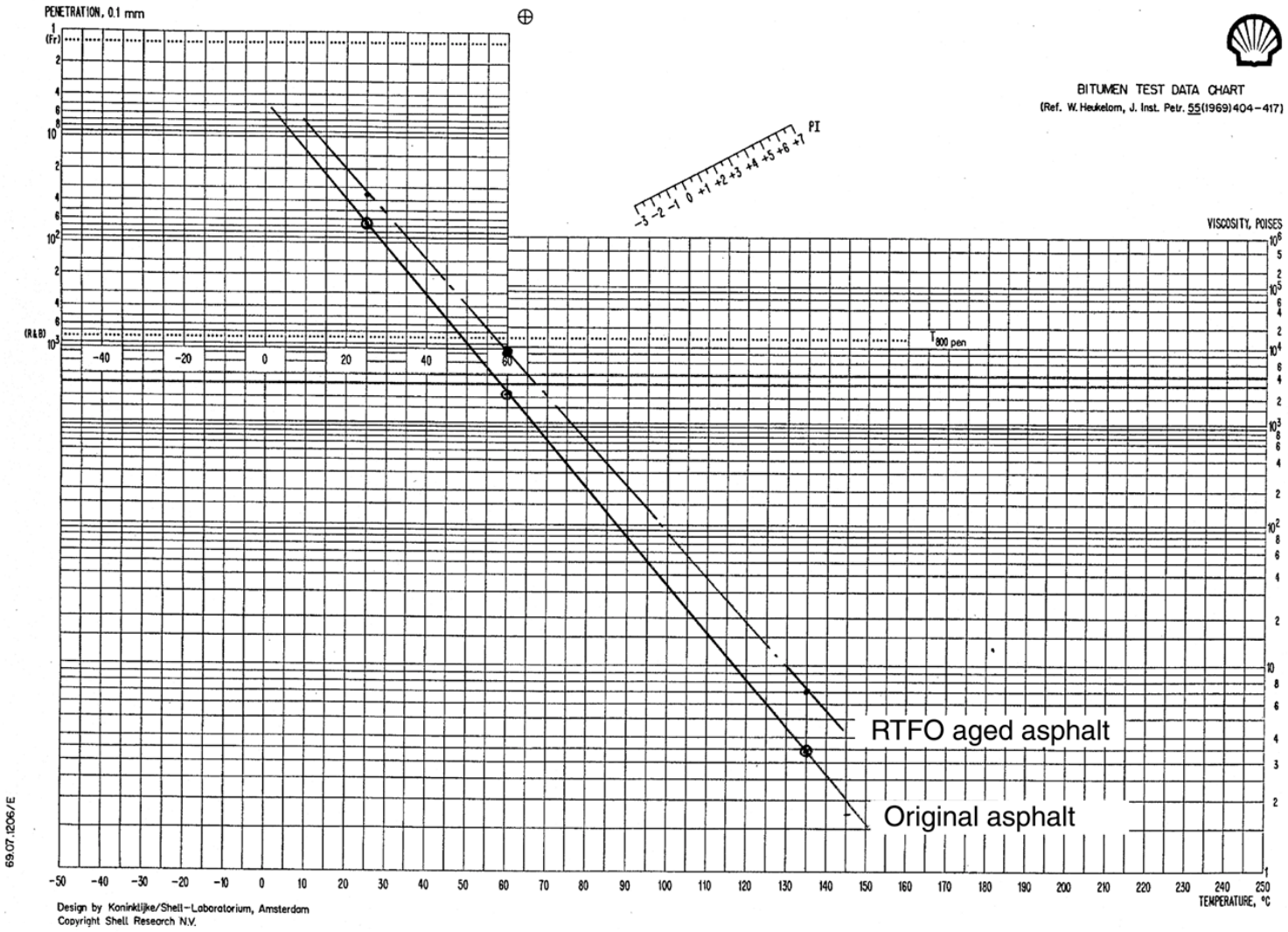
Figure 6. Bitumen Test Data Chart (AR-8000)
