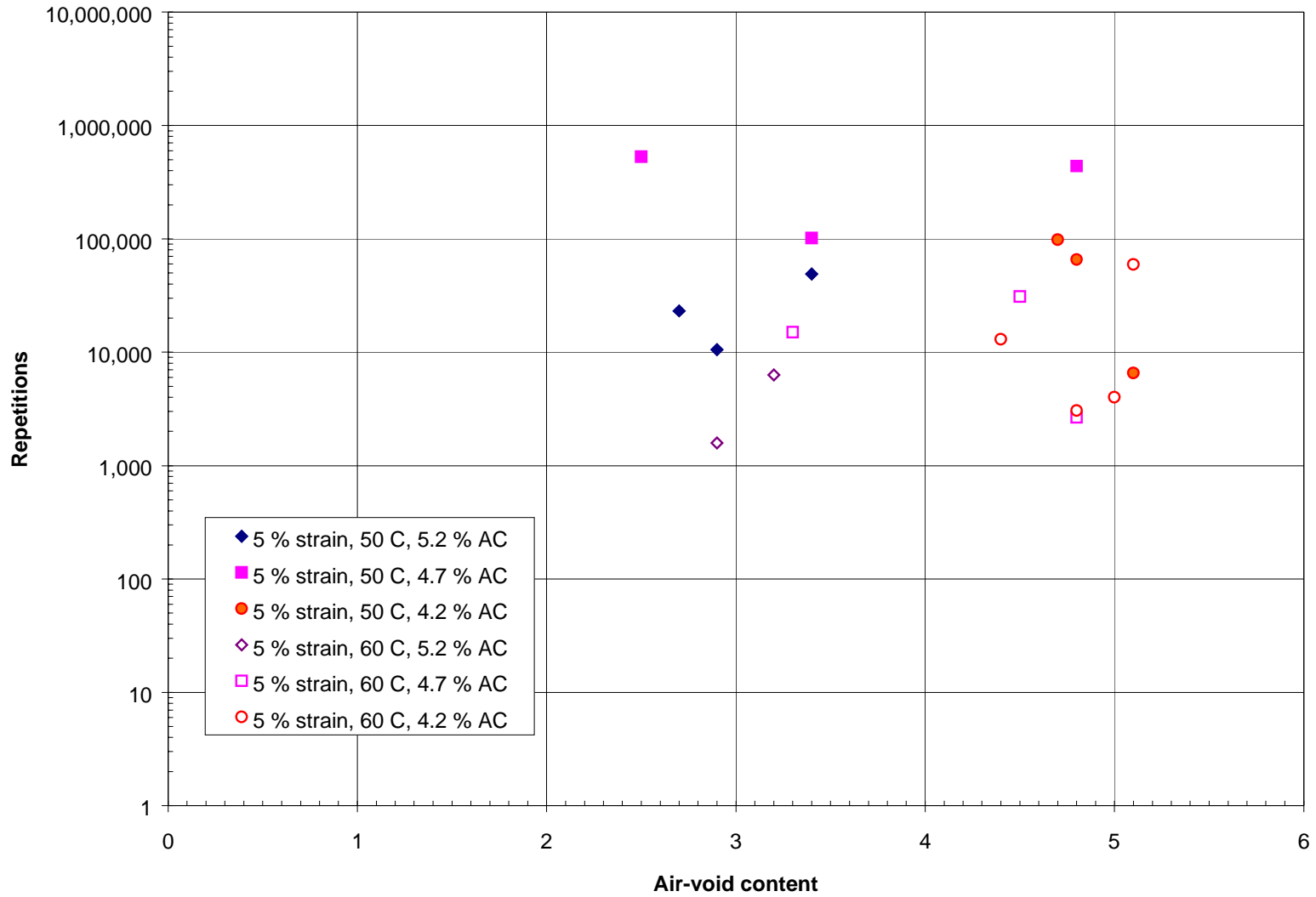
Figure 19. Relationship between Number of Repetitions to 5 Percent Permanent Shear Strain and Air-Void Content, Mixes with AR-8000 Binder.
