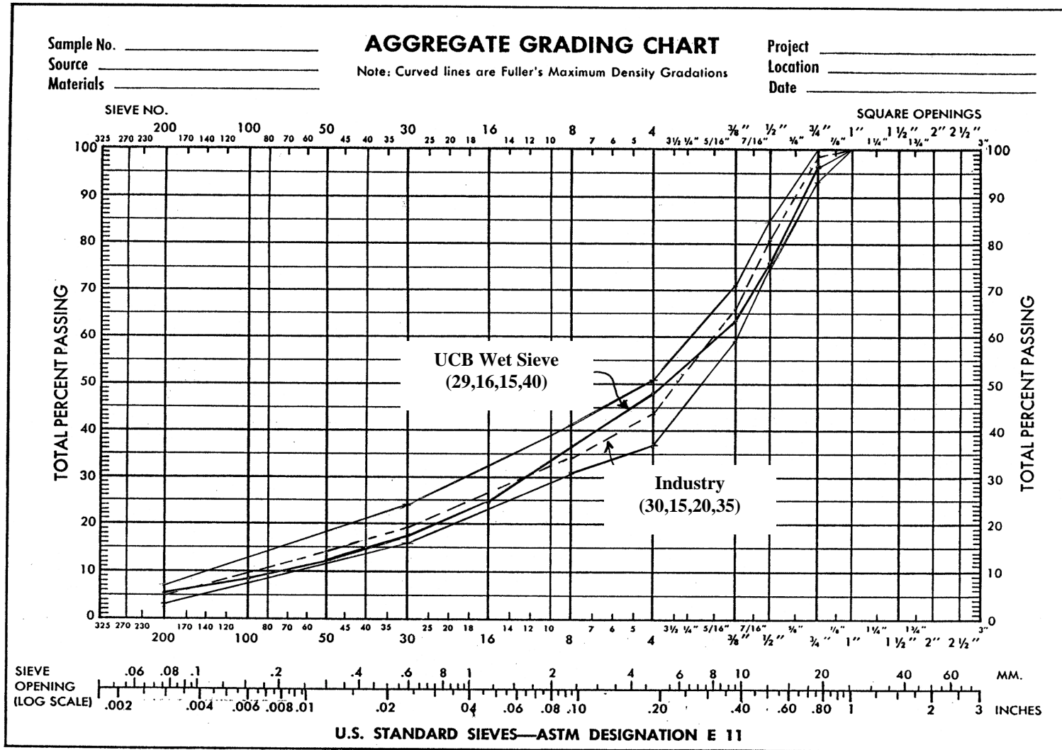
Figure 7. Comparison of UCB Wet Sieve and Industry Gradation.
