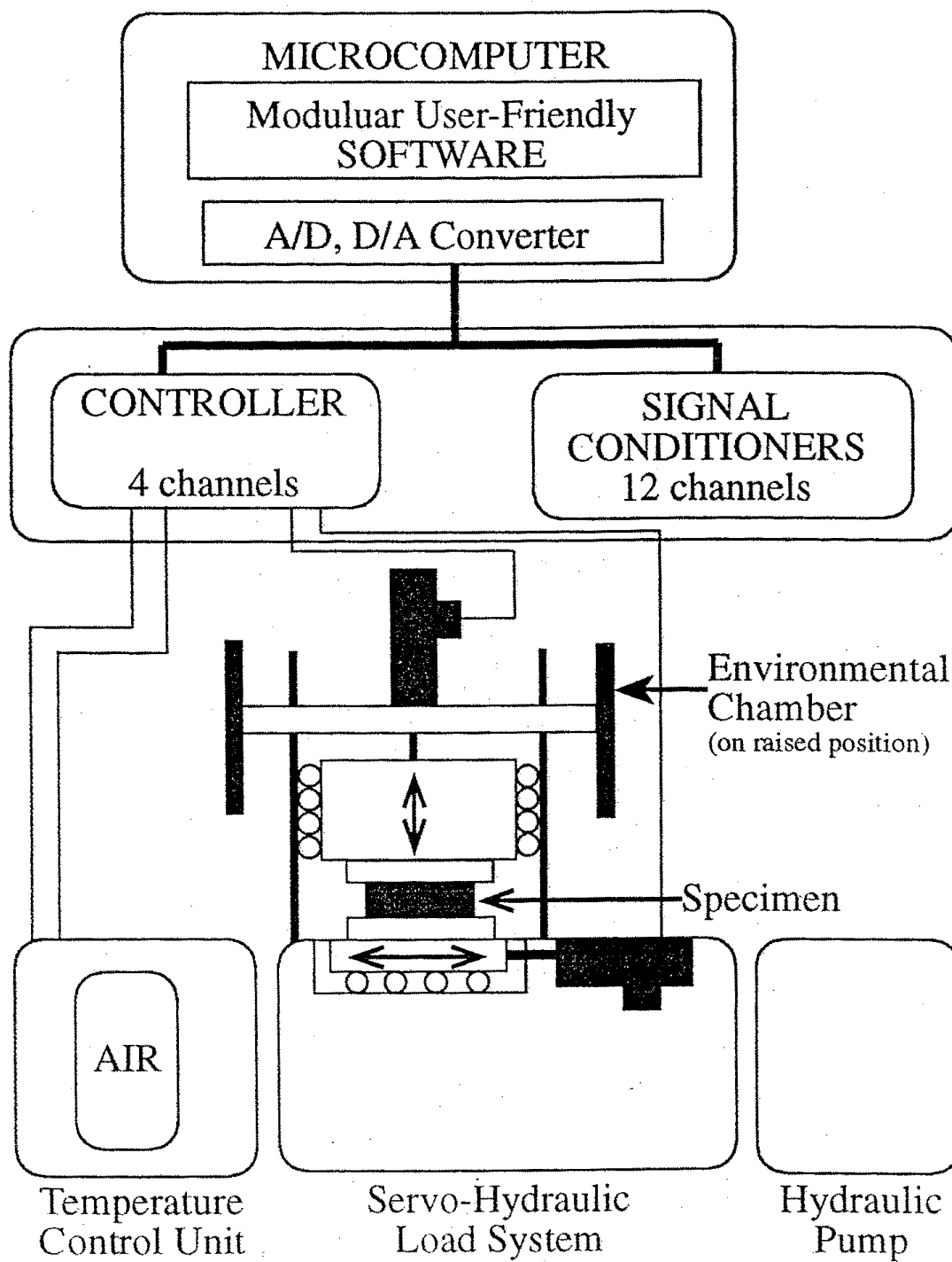
Figure 17. Schematic of Simple Shear Test.
