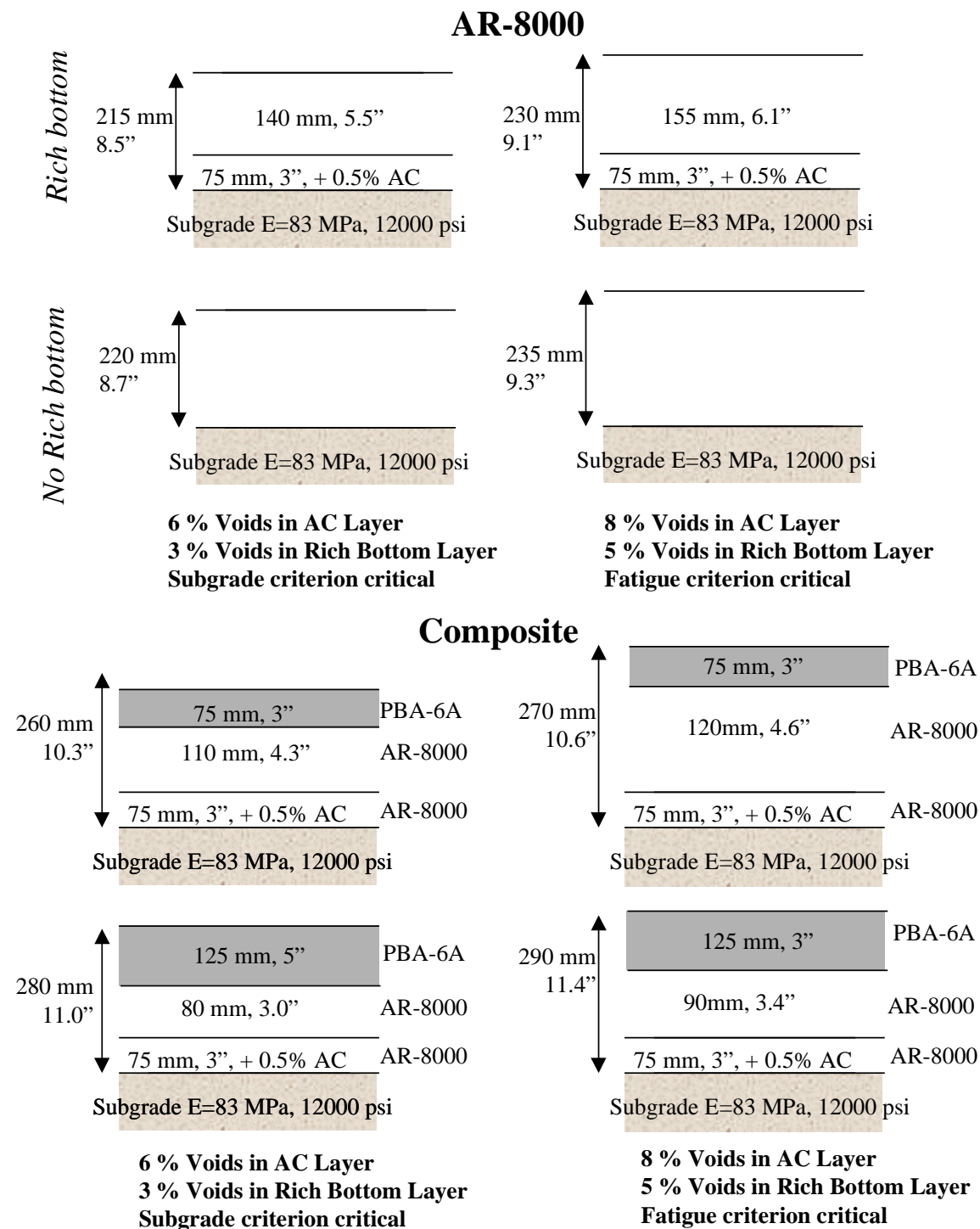
Figure 26. Structural Sections for AR-8000 and Composite Pavements with Increase in Air-Void Contents.
