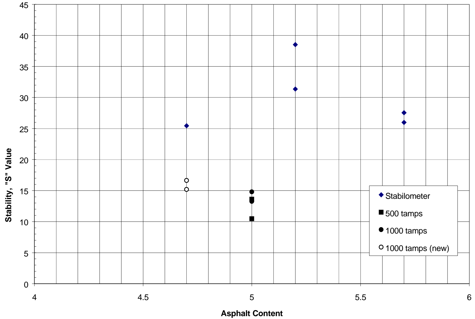
Figure 15. Stabilometer Data versus Asphalt Content, PBA-6A Binder.
