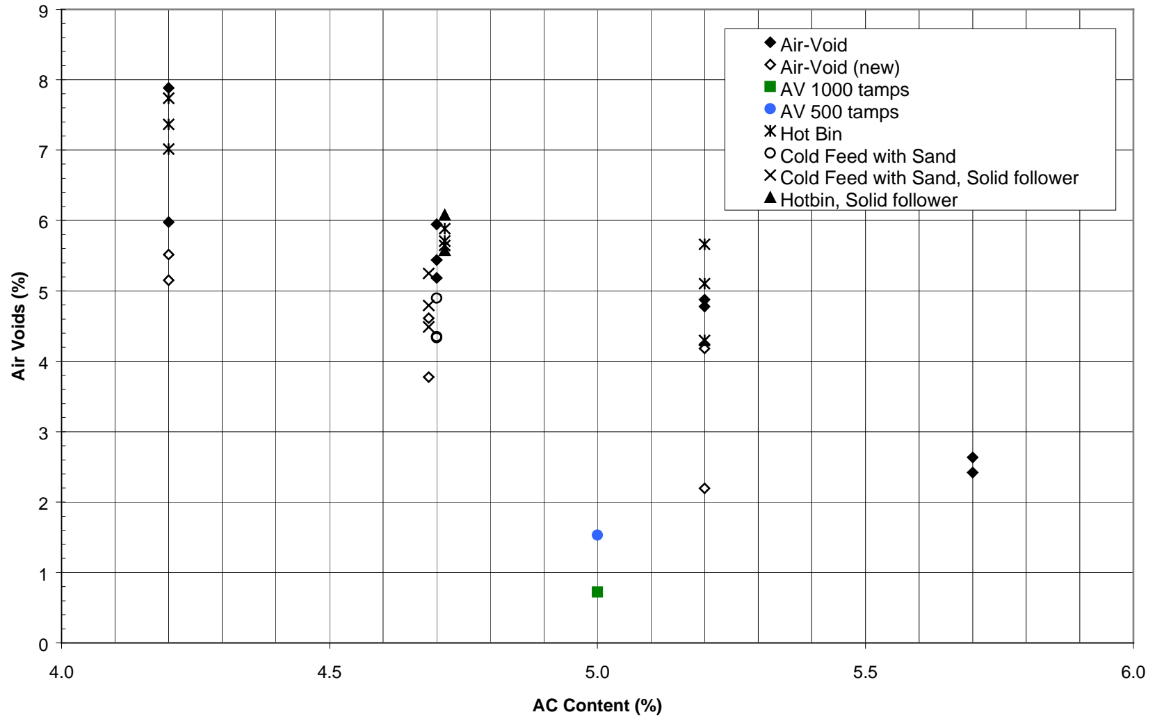
Figure 14. Air-Void Content versus Asphalt Content, Conventional AR-8000.
