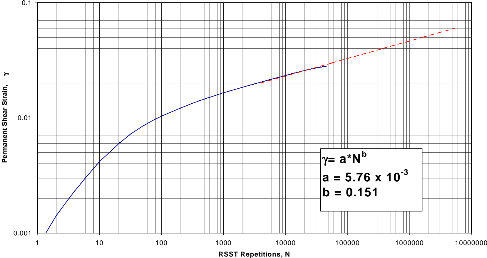
Figure 18. Permanent Shear Strain versus Stress Repetitions in RSST-CH at 50°C; PBA-6A Mix, 4.7 Percent Binder Content.
