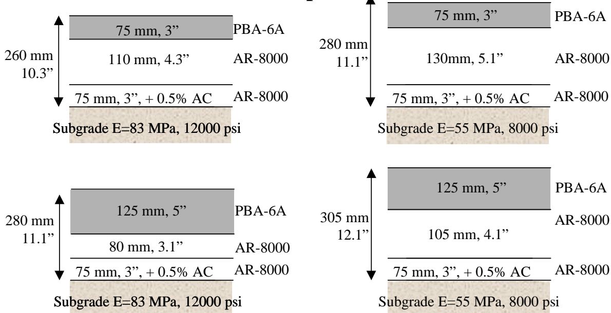
Figure 25. Structural Sections for AR-8000 and Composite Pavements (6 Percent Voids in AC Layer and 3 Percent in Rich Bottom Layer).
