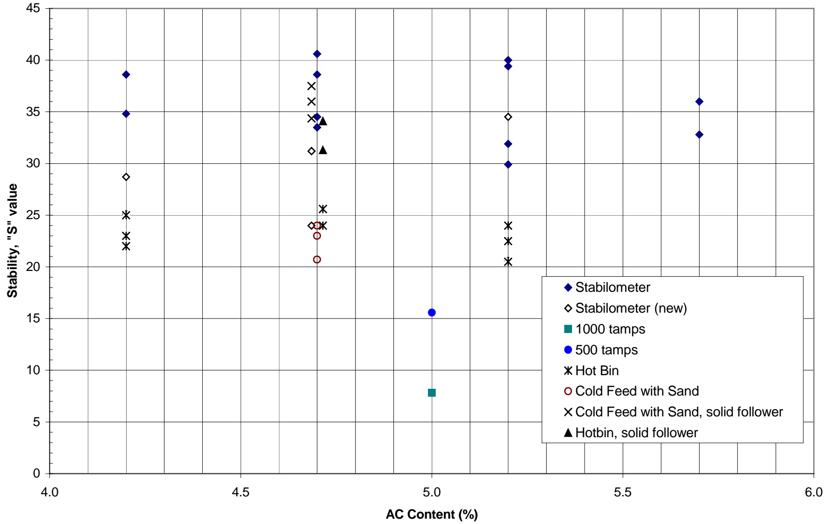
Figure 13. Stabilometer Data Versus Asphalt Content, Conventional AR-8000.
