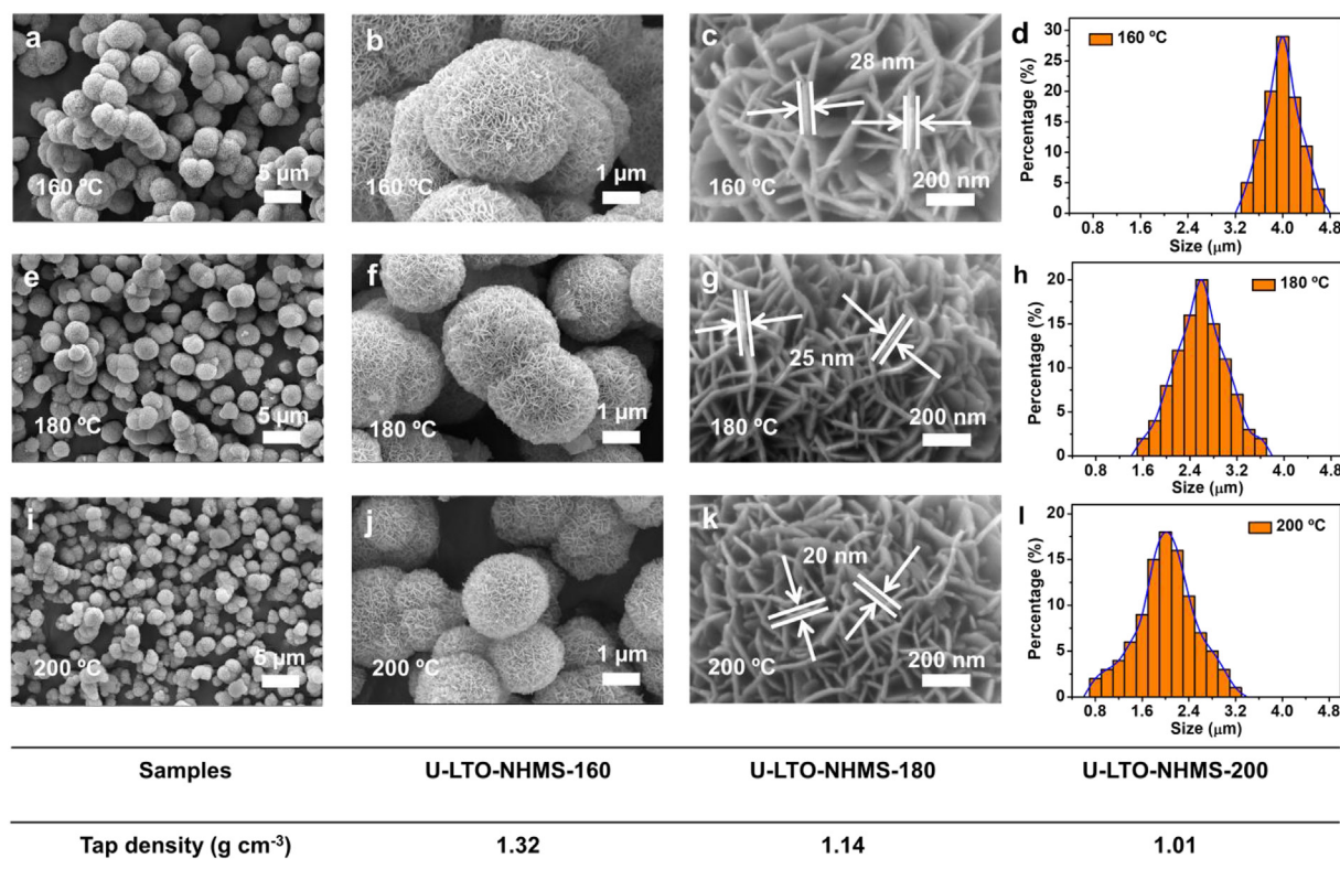
Fig. 1. SEM images and size distribution plot of U-LTO-NHMS-160 (a, b, c, d), U-LTO-NHMS-180 (e, f, g, h), and U-LTO-NHMS-200 (i, j, k, l); the Table in the bottom is the summary of tap density of three samples.
