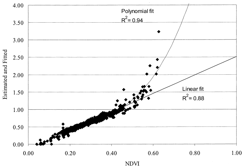
Figure 2. LAI-NDVI relationships [Eq. (2) in the text and a linear fit] used in this study.
