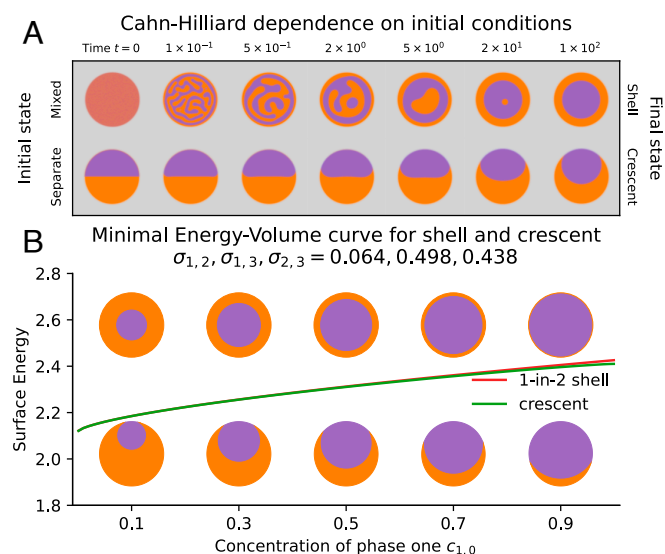
Fig. 3. (A) Evolution of ternary Cahn–Hilliard model from different initial conditions (mixed vs separate). For equal concentration ratio c_1 : c_2 = 0.5 , mixed initial conditions lead to shells, while initially separated drops form minimal-energy crescents. (B) Energy–volume curve for the shell (red) and crescent (green) configurations of figure (A) with surface tensions of Fig. 2C.
