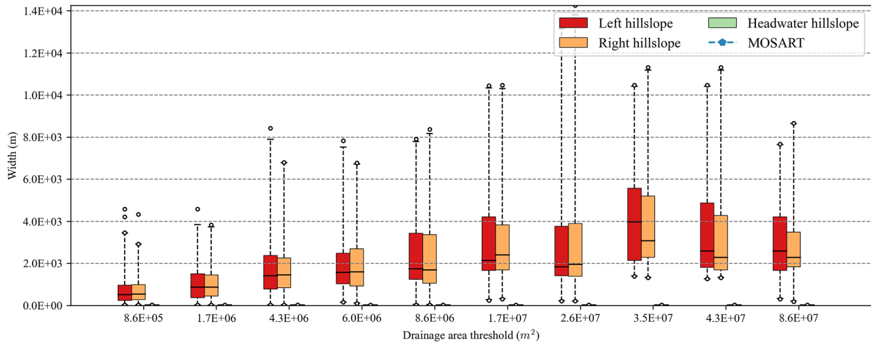
Figure B2. Boxplot comparisons of HexWatershed-modeled hillslope width from Cases 1 to 10 (Table 2). The x axis represents different drainage area thresholds. Each box group includes left, right, and headwater hillslope. The MOSART elevation-profile-based width is out of the range.
