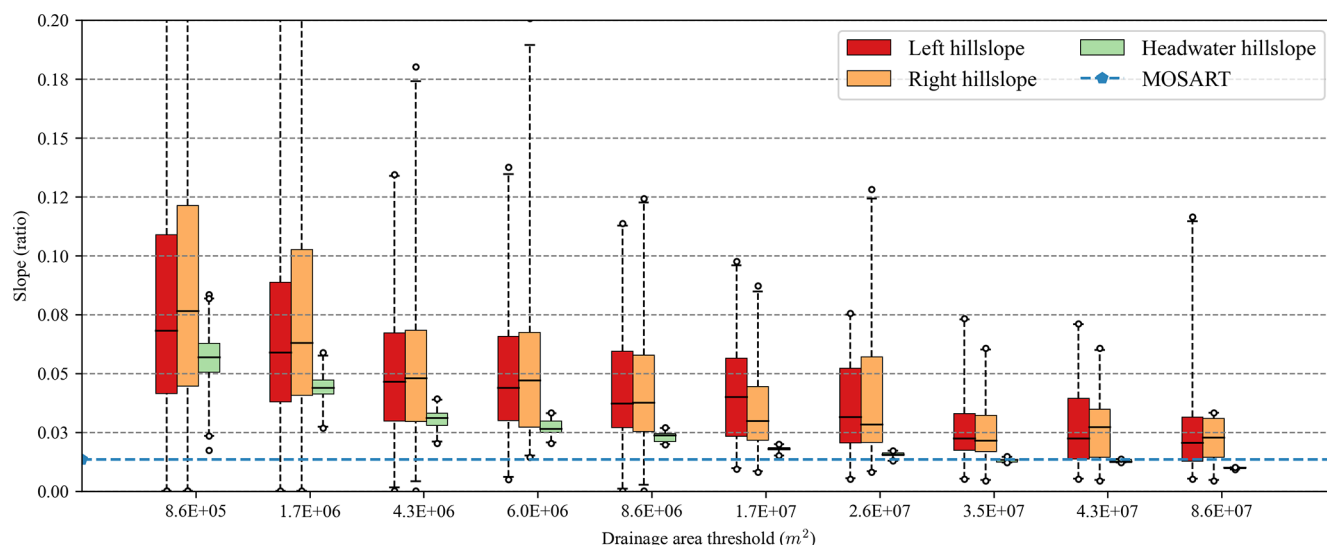
Figure 7. Boxplot comparisons of HexWatershed-modeled hillslope slopes from Cases 1 to 10 (Table 2). The x axis represents different drainage area thresholds. Each box group includes left, right, and headwater hillslope. The dashed blue line is the MOSART elevation-profile-based slope.
