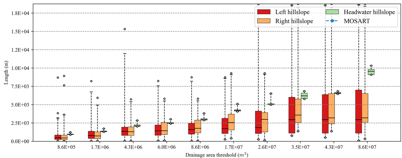
Figure 6. Boxplot comparisons of HexWatershed-modeled hillslope length from Cases 1 to 10 (Table 2). The x axis represents different drainage area thresholds. Each box group includes left, right, and headwater hillslope. The MOSART elevation-profile-based length is out of the range.
