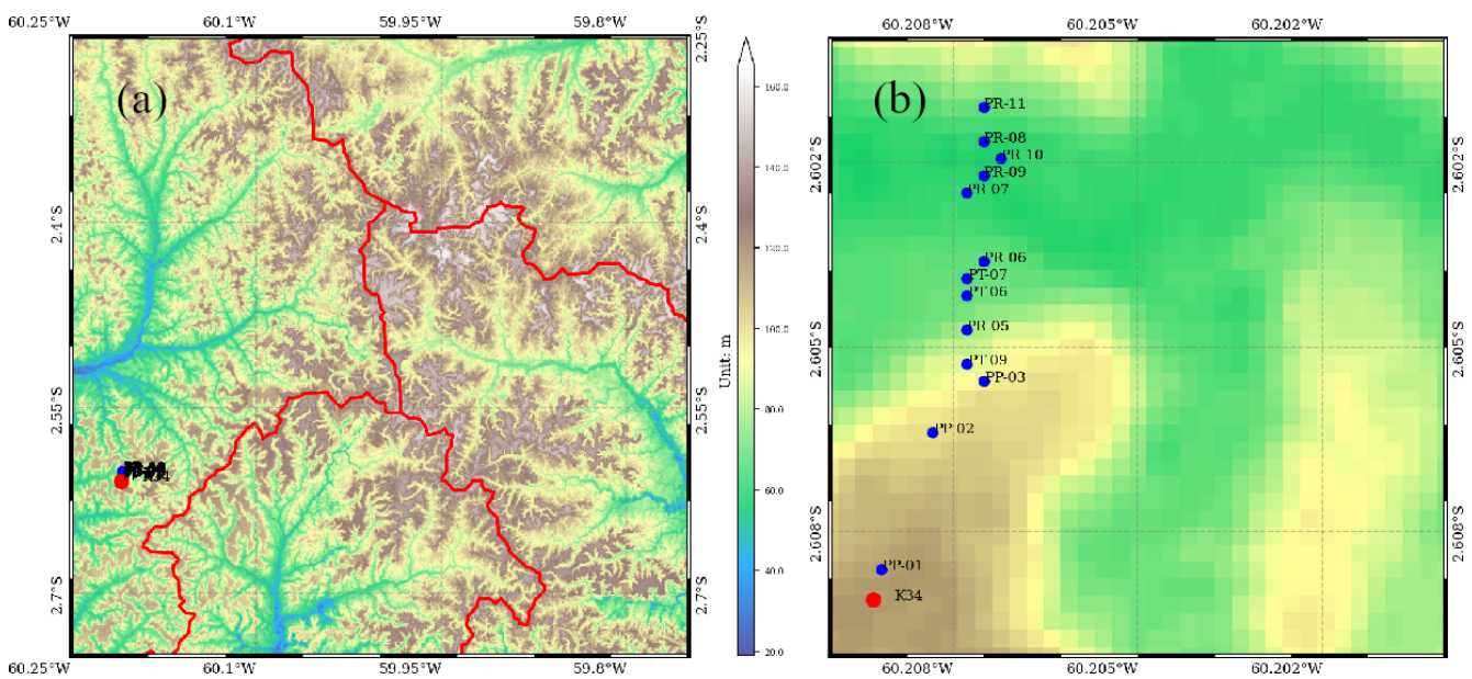
Figure 4. Surface elevation of the study area (unit: m) and locations of in situ measurement sites. Panel (a) is the 30 m resolution surface elevation of the 0.5^{\circ} \times 0.5^{\circ} ELM grid cell. The red lines are watershed boundaries. Panel (b) is a zoomed-in view of the hillslope transect.
