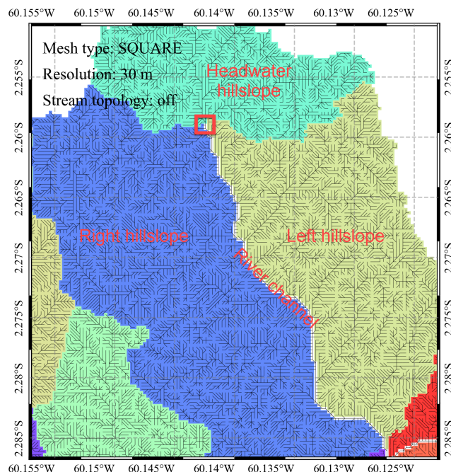
Figure 2. Illustration of the hillslope definition. The colored polygon features are the delineated hillslopes. The white-colored poly-line segment in the middle is a delineated river channel by HexWatershed. The black lines from cell to cell are the flow direction field. The river channel is linked to three hillslopes. All the cells entering from the left/right side (upstream facing downstream) of the river channel are grouped as left/right hillslopes. All the cells entering the river channel through the first river channel cell (highlighted in red rectangle) are grouped as the headwater hillslope. The results are produced using the HexWatershed model with 30 m DEM. Map visualization is supported by the PyEarth Python package (Elson et al., 2023; Liao, 2022b).
