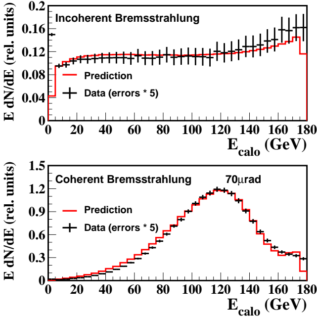
FIG. 13: Power spectrum for incoherent (top) and for coherent bremsstrahlung (bottom) as a function of the total energy E_{calo} detected in the calorimeter. Vertical axis: Power (rel. units). The statistical errors on the data are enhanced by a factor of five to increase visibility.
