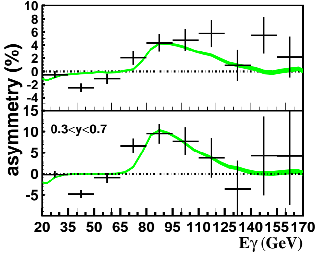
FIG. 16: Asymmetry to determine the \eta_3 component of the CB photon polarization with the Ge analyzer. Measurements without ( TOP ) and with ( BOTTOM ) the quasi-symmetrical pair selection at roll angles 0 + \pi are compared to those at roll angles \pi/2 + 3\pi/2 .
