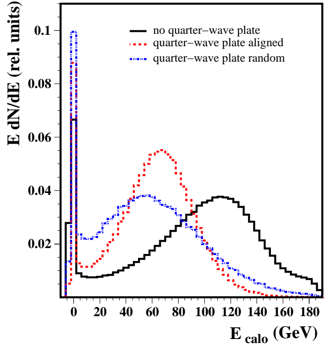
FIG. 18: Power spectrum of the photon beam measured in the calorimeter. Without the quarter wave plate crystal the predicted CB spectrum is observed (solid line). With the aligned quarter wave plate inserted the spectrum shifts to lower energies (dashed line). And with the quarter wave plate in random orientation we see more spread in the shifted spectrum.
