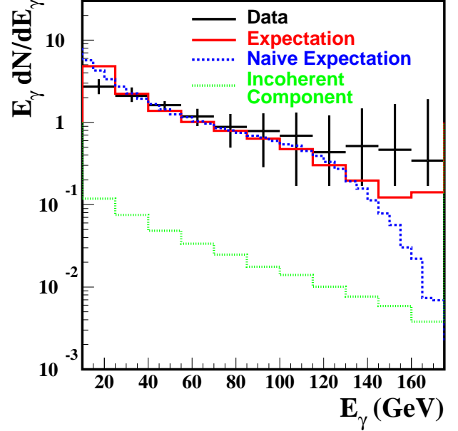
FIG. 23: Photon power yield, E_\gamma dN/dE_\gamma , as a function of the energy E_\gamma of individual photons radiated by an electron beam of 178 GeV in the SOS-aligned 1.5 cm Si crystal. The black crosses are the measurements with the pair spectrometer, the vertical lines represent the errors including the uncertainty in the acceptance of the spectrometer. The (red solid) histogram represent the Monte Carlo prediction for our experimental conditions. The (green dotted) represent the small contribution due to incoherent interactions. For completeness, we also show the theoretical predictions if the experimental effects are ignored (blue dashed).
