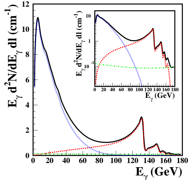
FIG. 3: Photon power yield, E_\gamma d^2 N / dE_\gamma dl , per unit of thickness for a thin silicon crystal in the SOS orientation. The solid curve represents the total of the contributions from ICB (green dash-dotted), PC (blue dotted) and SOS (red dashed) radiation. The insert is a logarithmic representation and shows the flat incoherent contribution and the enhancement with a factor of about 20 for SOS radiation at 129 GeV.
