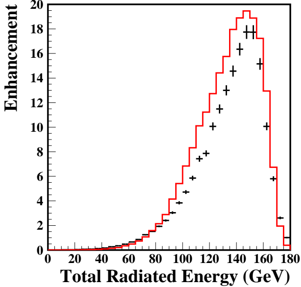
FIG. 24: Enhancement of the intensity with respect to the Bethe-Heitler (ICB) prediction for randomly oriented polycrystalline Si as a function of the total radiated energy E_{tot} in the SOS-aligned Si crystal by 178 GeV electrons. The black crosses are the measurements and the red histogram represent the Monte Carlo prediction.
