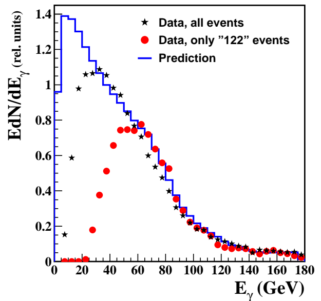
FIG. 12: Monte Carlo predictions for the single photon spectrum, compared with data using all events (stars) and only '122 type' events (circles).
