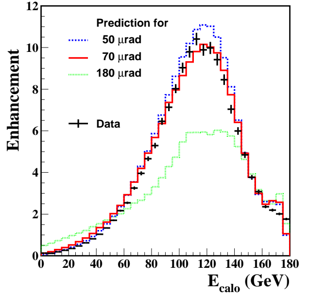
FIG. 14: Enhancement of CB radiation data compared to Monte Carlo predictions. Note the sensitivity of the cross section to small changes in the angular setting of the crystal.
