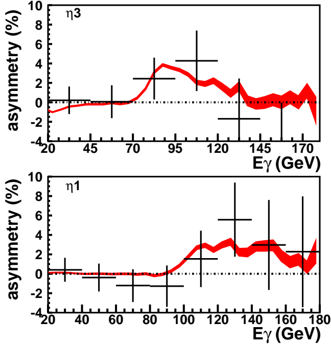
FIG. 22: Asymmetry measured with the Ge analyzer (top) and the pair spectrometer (bottom). The data sample with a fully reconstructed single e^+e^- pair is ten times smaller than the total data sample with at least one pair passing all the data quality cuts and with a 2MIPs cut (see section IV-A) in S11.
