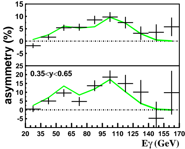
FIG. 17: Asymmetry measurements without ( TOP ) and with ( BOTTOM ) the quasi-symmetrical pair selection to determine \eta_3 component of the photon polarization with the diamond analyzer (Cf. Table II).
