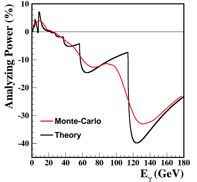
FIG. 26: Analyzing power R with the aligned diamond crystal as a function of the photon energy E_\gamma (black curve) for an ideal photon beam without angular divergence and (red curve) for the Monte Carlo simulation of photons with the beam conditions in the actual experiment.
