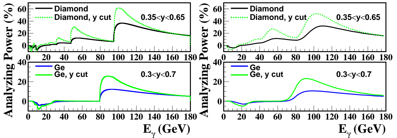
FIG. 5: Analyzing power of different single crystals, for an ideal e^- beam without any angular divergences (left) and for the actual e^- beam conditions (right).
