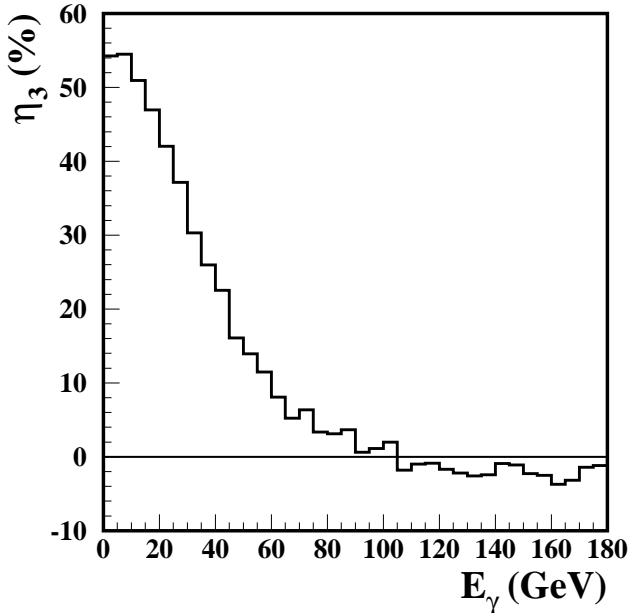
FIG. 25: Expected linear polarization as a function of the energy E_\gamma of the photons produced in the SOS-aligned Si crystal by 178 GeV electrons.
