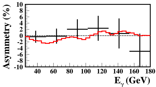
FIG. 27: Asymmetry of the e^+e^- pair production in the aligned diamond crystal as a function of the photon energy E_\gamma which is measured to determine the P_1 component of the photon polarization in the SOS-aligned Si crystal by 178 GeV electrons. The black crosses are the measurements and the red histogram represent the Monte Carlo prediction.
