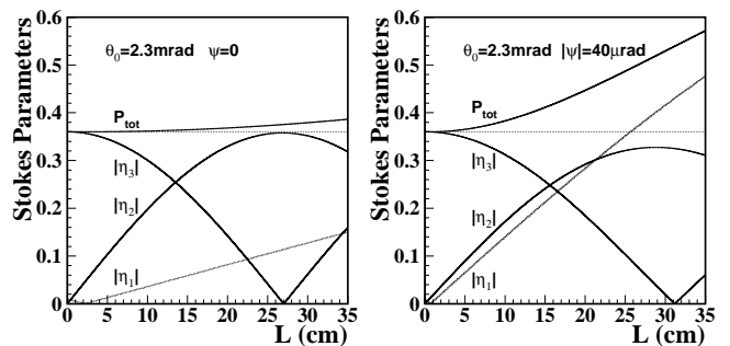
FIG. 8: Absolute values of the Stokes parameters and the total degree of polarization for a Si crystal as a function of its thickness L , for E_\gamma=100 GeV linearly polarized photons. The left hand figure and the right hand figure are calculated using initial values for the Stokes parameters described in the text. For these conditions, the crystal also acts as polarizer generating a \eta_1 component.
