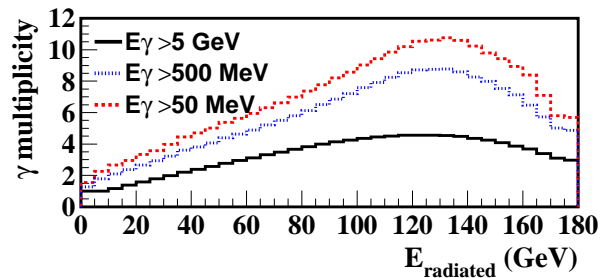
FIG. 1: Monte Carlo prediction for photon multiplicity vs total radiated energy using different photon energy cut-off values.
