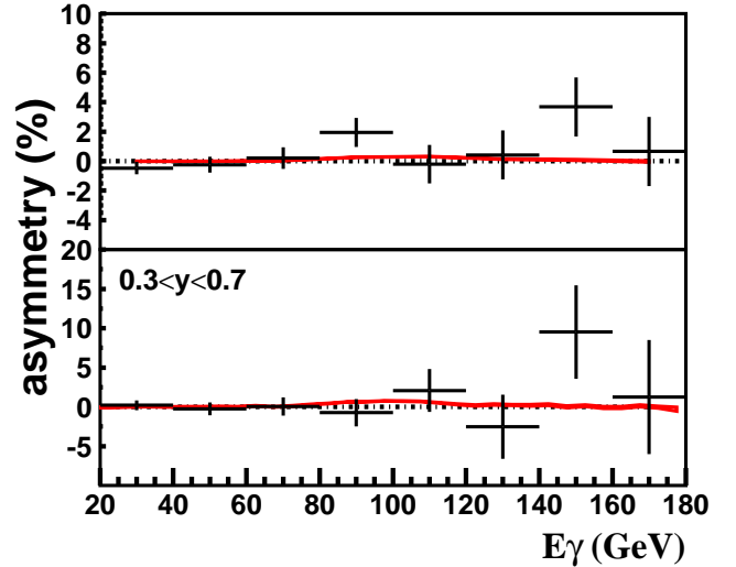
FIG. 15: Asymmetry to determine \eta_1 component of the photon polarization with the Ge analyzer. The data at roll angles \pi/4 + 5\pi/4 are compared to 3\pi/4 + 7\pi/4 without (top) and with (bottom) the quasi-symmetrical pair selection.
