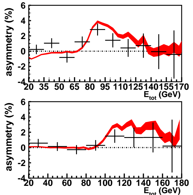
FIG. 21: Asymmetry measured with the calorimeter. The results reflects the changes in \eta_3 (top) and generation of \eta_1 (bottom) due to the presence of the quarter wave crystal .
