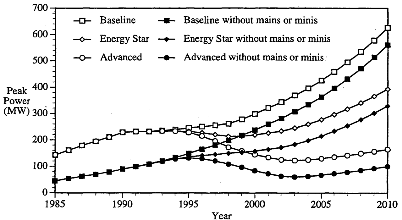
Figure 6.15. Winter Peak Power Demand by Scenario.
