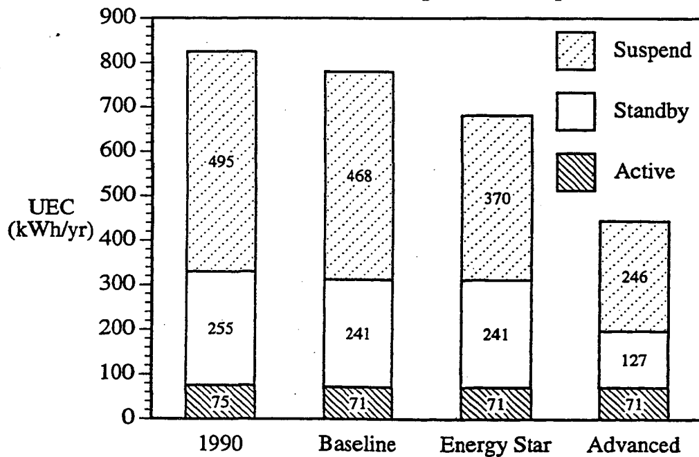
Figure 6.5. Baseline (1990 and 2000), Energy Star, and Advanced Scenario Unit Energy Consumption for Copiers.
