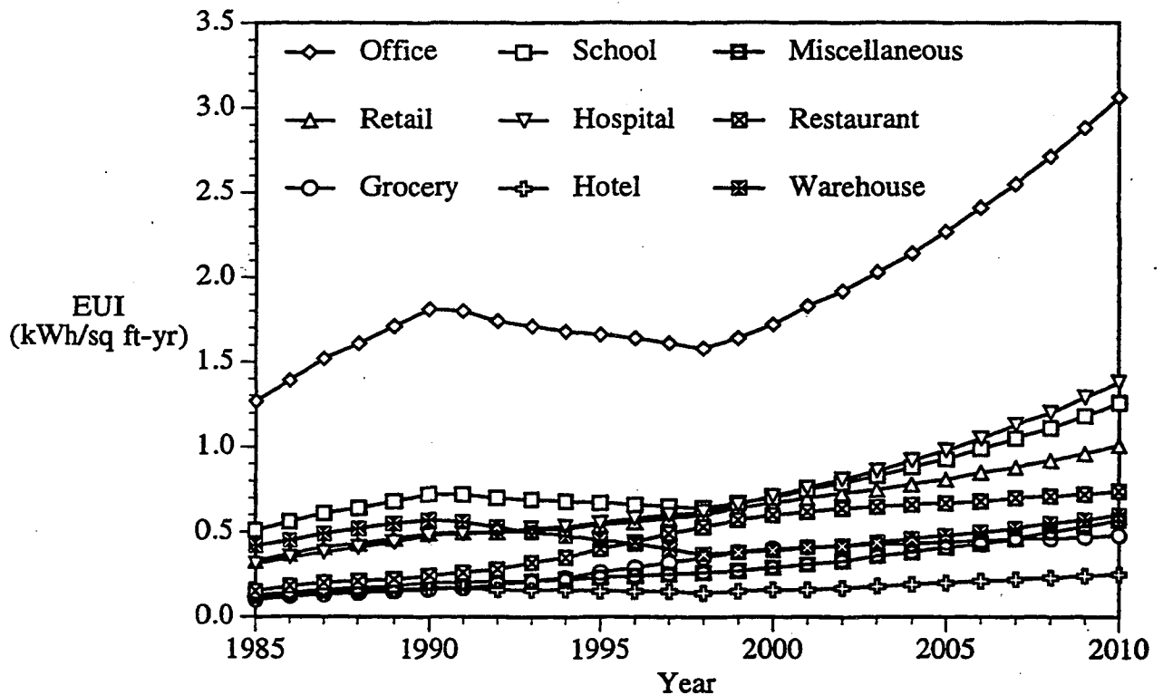
Figure 6.9. Baseline Scenario: Energy-Use Intensity by Building Type.
