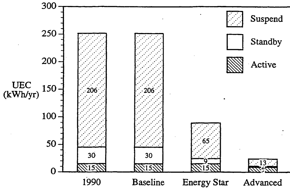
Figure 6.4. Baseline (1990 and 2000), Energy Star, and Advanced Scenario Unit Energy Consumption for Printers.
