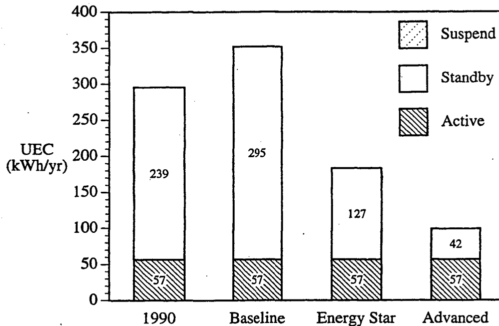
Figure 6.6. Baseline (1990 and 2000), Energy Star, and Advanced Scenario Unit Energy Consumption for Fax Machines.
