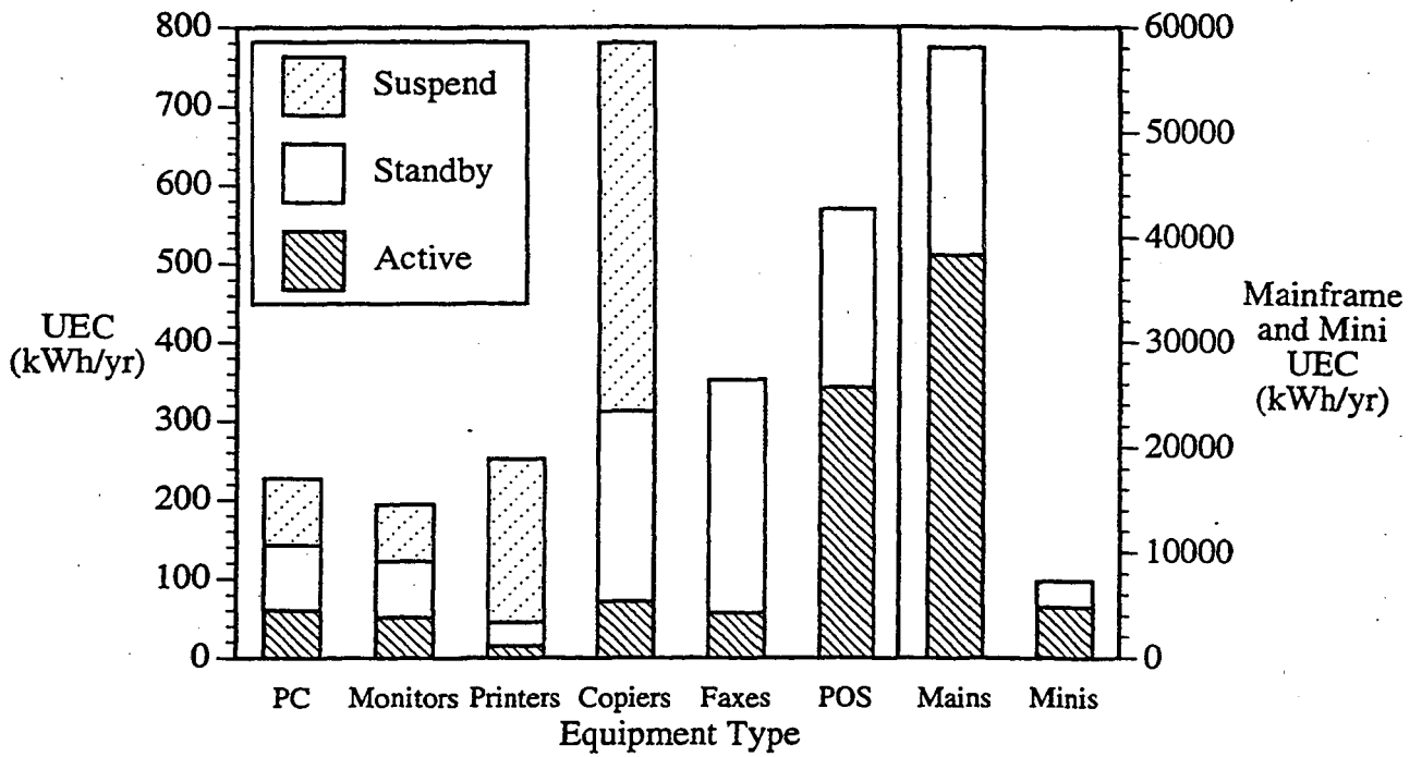
Figure 6.1. Baseline Scenario Unit Energy Consumption (Year 2000).
