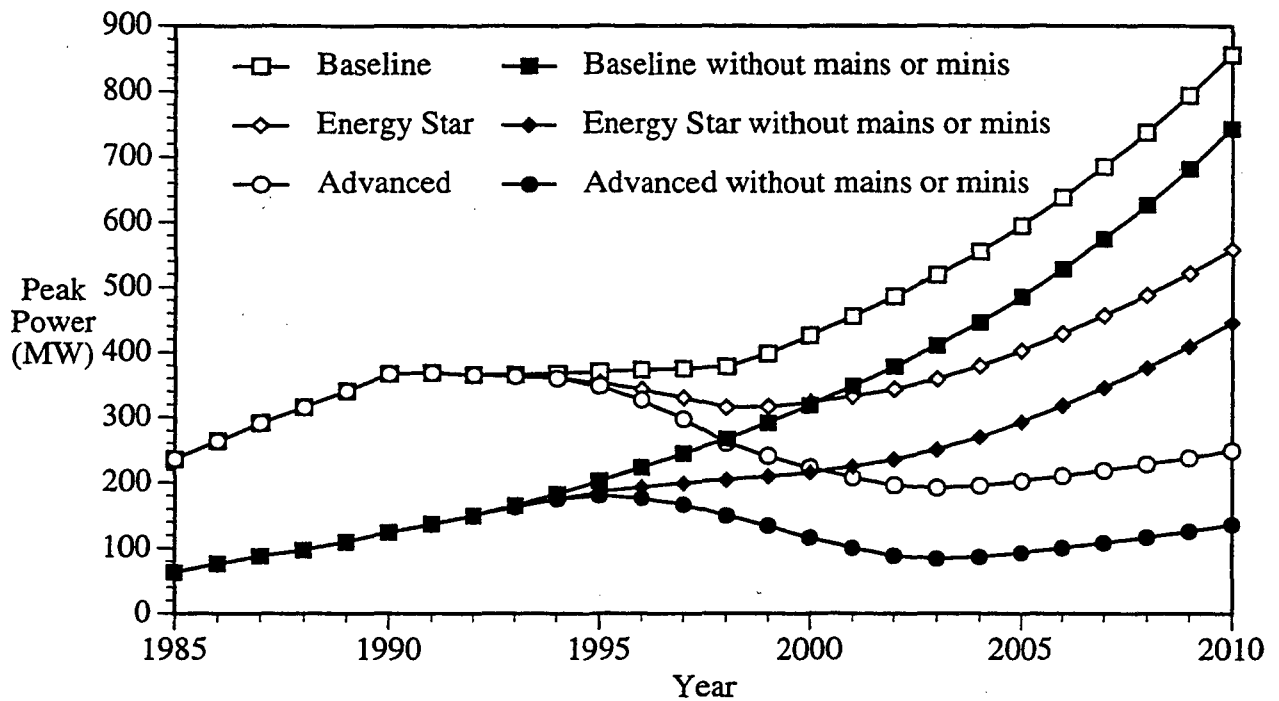
Figure 6.14. Summer Peak Power Demand by Scenario.
