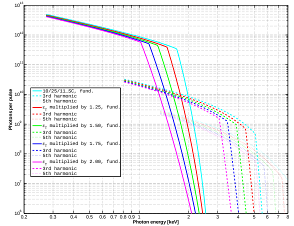
Figure 2: The performance of a design point is plotted together with several other design points obtained by increasing the emittance by varying amounts.
