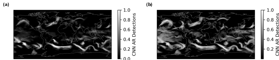
Figure 6. CNN-based AR detections with and without perceptual loss. CNN AR detections in 0.25^\circ ERA-I at the same time as Figs. 1–4 (a) with a perceptual loss function and (b) with a pixel-wise cross-entropy loss function.
