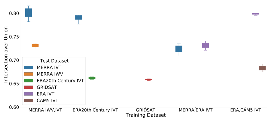
Figure 8. Performance of ARCNNs on different climate datasets and input fields. Five ARCNNs are trained on different datasets and input fields, as shown on the x axis. Their performance is measured by IoU (with 0 being the worst and 1 being the best) on different test datasets. The IoU scores are the average of the IoU for the foreground class (AR) and background class (not AR). On each test dataset, the input field is multiplied by a factor ranging from 0.9 to 1.1 in increments of 0.02, and the IoU score is calculated. For the resulting 11 IoU scores, the box shows the lower and upper quartile, and the whiskers show the minimum and maximum of the IoU scores. All IoU scores are on test set years of 1984, 1997, 2003, 2010, and 2015.
