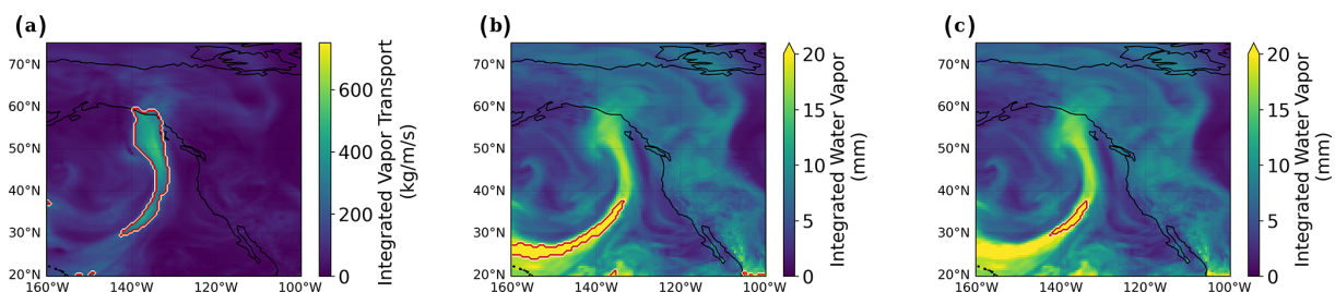
Figure A1. Further info on the textbook algorithm. In panel (a), the IVT is at the same time as in Fig. 2. The dashed red contour shows the region above 250 \text{ kg m}^{-1} \text{ s}^{-1} . Panel (b) shows IWV. The dashed red contour denotes the region above 20 mm. Panel (c) shows IWV, and the dashed red line denotes the region above both 250 \text{ kg m}^{-1} \text{ s}^{-1} and 20 mm.
