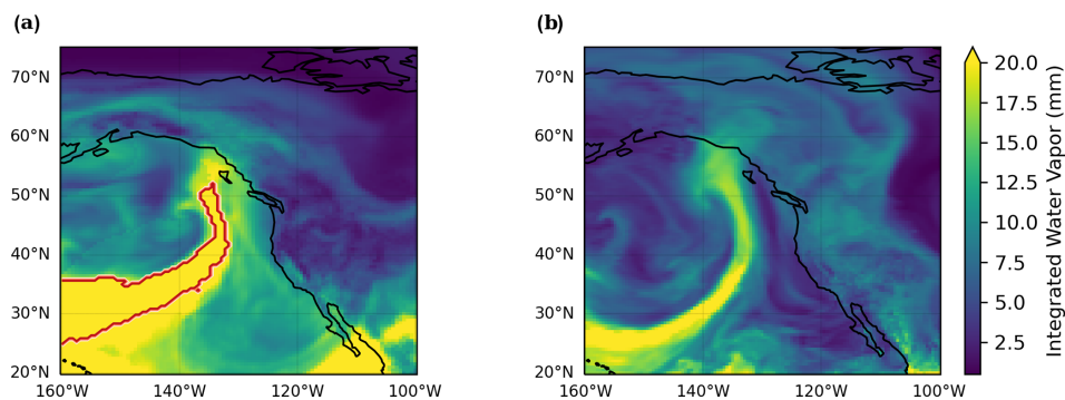
Figure 2. AR detections in MERRA-2 and ECMWF-IFS-HR from a threshold-based detection algorithm. (a) The detection algorithm from the Atmospheric Rivers textbook (Ralph et al., 2020) identifies an atmospheric river (AR) in MERRA-2 reanalysis (Gelaro et al., 2017). The AR contour is shown in red. (b) The same threshold algorithm does not identify an atmospheric river with a similar structure in ECMWF-IFS-HR (Roberts et al., 2018), a free-running, high-resolution climate model.
