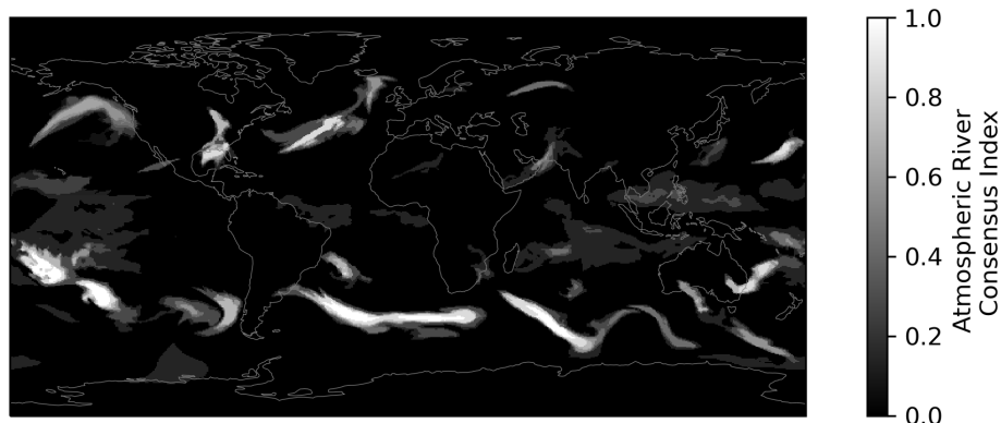
Figure 3. Example of the atmospheric river consensus index (ARCI). ARCI (black and white shading) refers to the proportion of 14 AR detection algorithms that identify an AR. ARCI ranges from 0 (none of the AR detection algorithms identified an AR) to 1 (all algorithms identified an AR). ARCI is at the same time step as Fig. 1.
