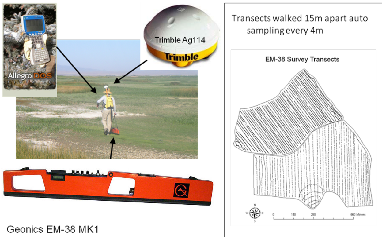
Figure 6.2. Mapping wetland soils using the Geonics EM-38 Mrk 1 and Mrk II instruments, Trimble GPS and Allegro logging unit.
