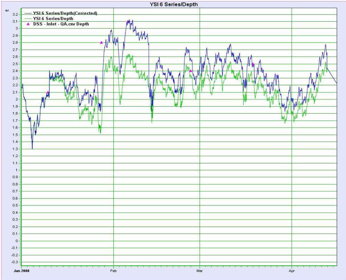
Figure 3.9. Aquarius allows the raw data to be plotted with the corrected data after QA analysis. The software also allows the data manipulations to be annotated and associated with the data trace. Plot is for YSI sensor depth at the Ducky Strike South pond.
