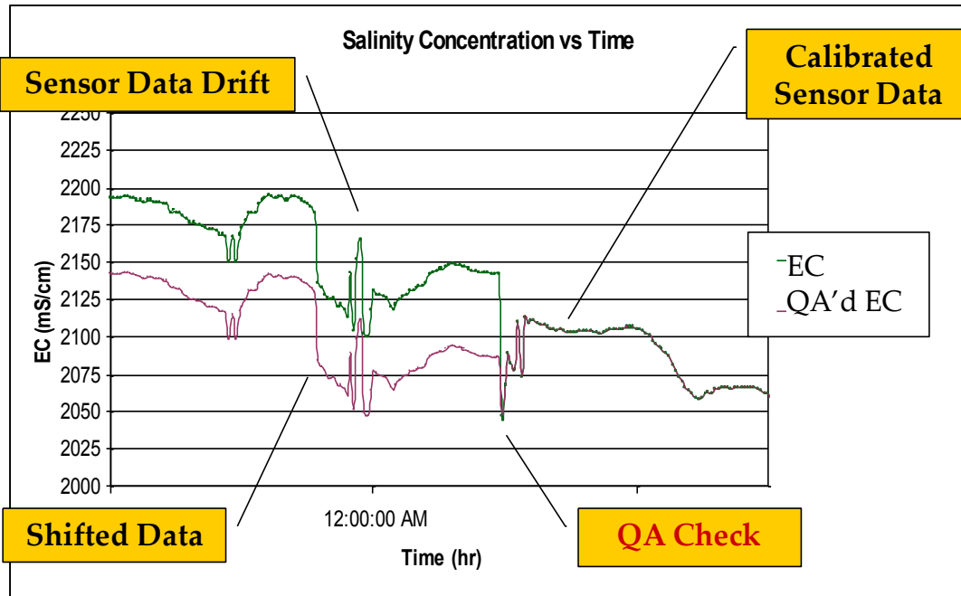
Figure 4.1. Example of adjustments made to YSI Sonde EC data to correct for sensor drift and match monitoring site QA data.
