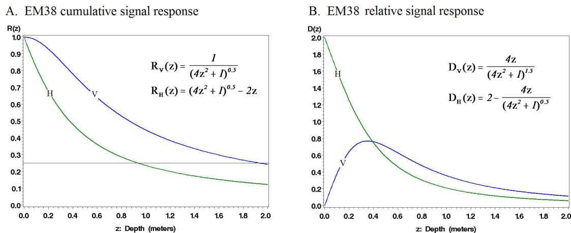
Figure 6.1. EM38 (a) cumulative and (b) relative signal responses where H is horizontal orientation and V is vertical orientation (McNeill 1980).
