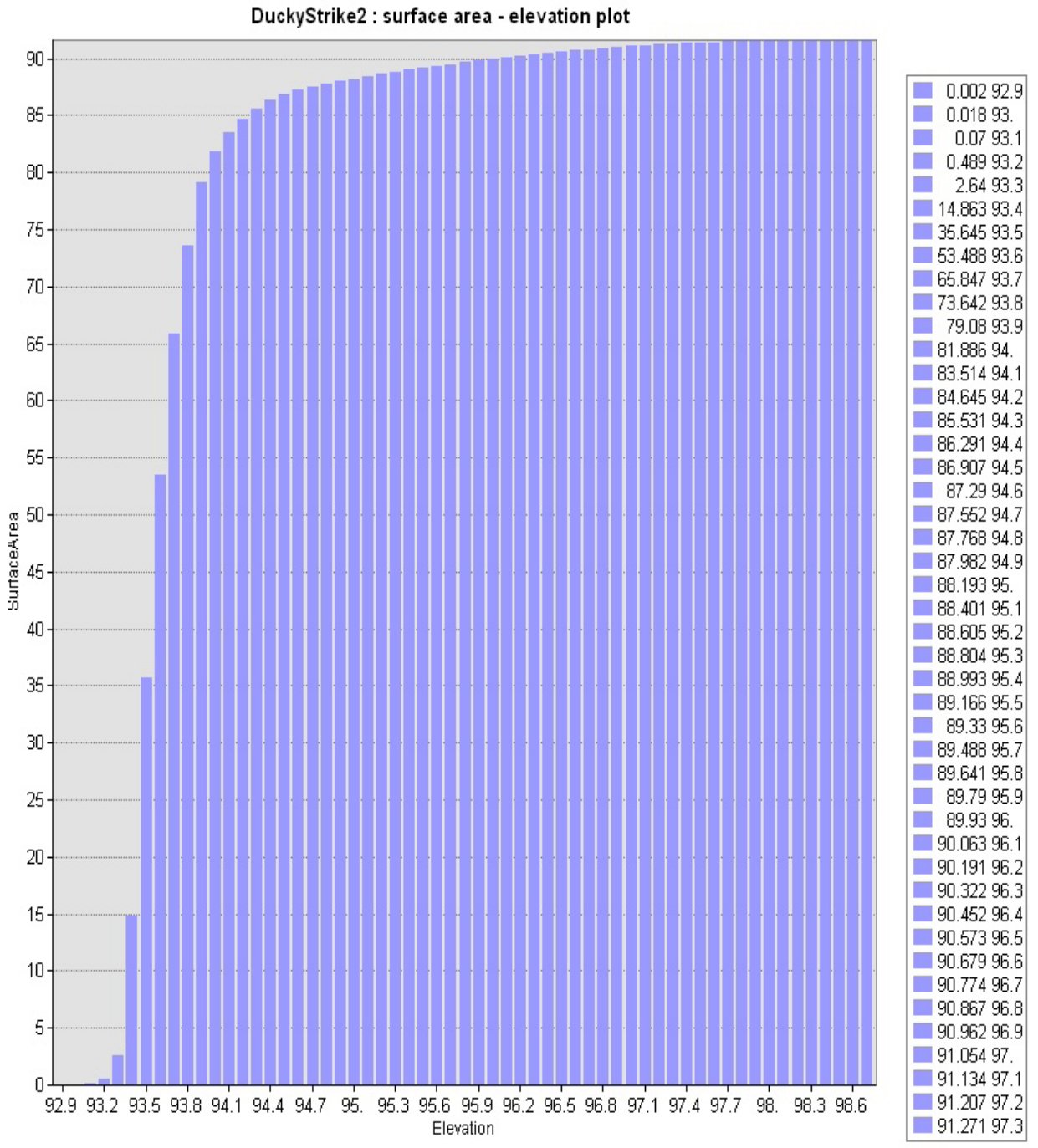
Figure 3.11. Surface-area –elevation plot for Ducky Strike Duck Club (South pond ) obtained from a motorized GPS survey during 2007 .
