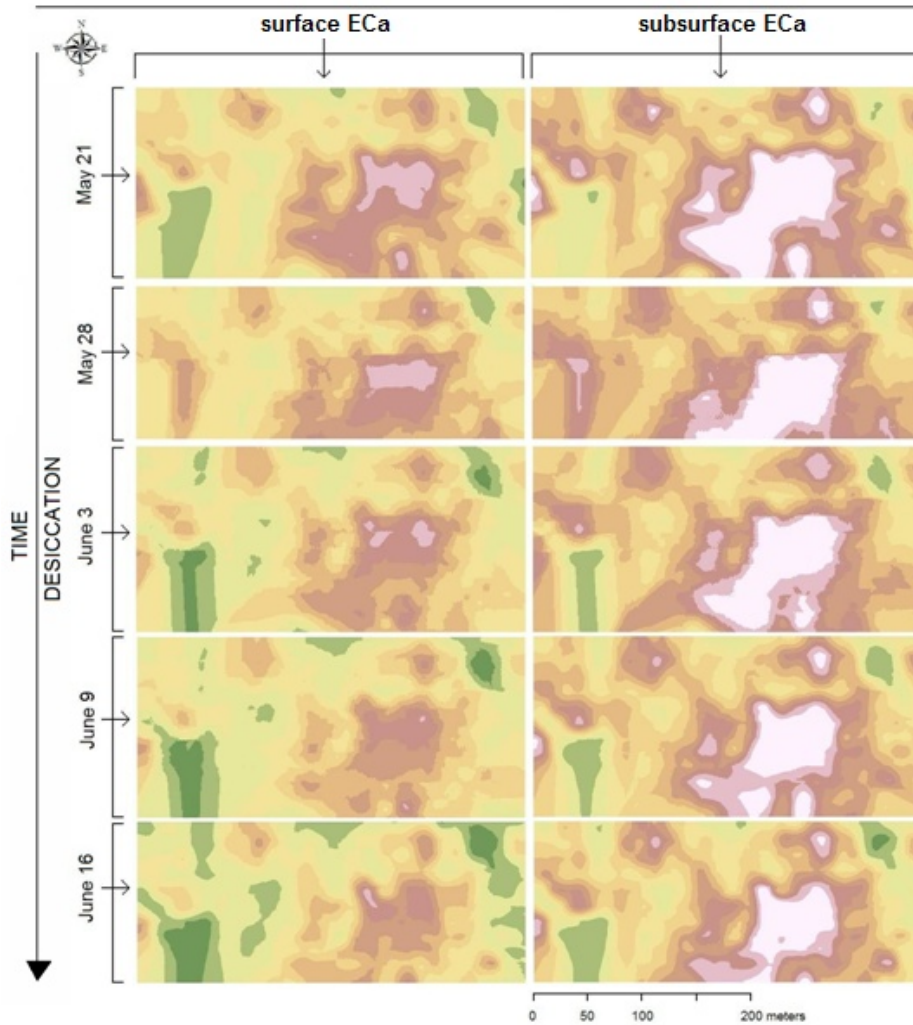
Figure 6.8 Temporal Study at MS 3b in 2008 demonstrating the effects of soil desiccation on EM-38 signal response. Weekly Surveys conducted from May 21, 2008 thru June 16, 2008 following exact transects for each survey. Surface ECa (left column) represent the EM-38 Horizontal signal, subsurface ECa (right column) represents the EM-38 Vertical signal.
