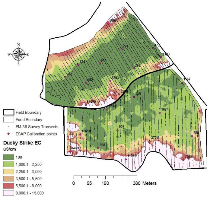
Figure 6.13. Ducky Strike North and South, 2008 calibrated EC1:2 maps of surface bulk soil salinity, 0 – 30 cm.
