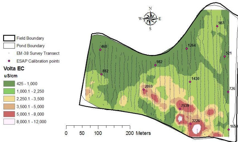
Figure 6.19. Volta 4d calibrated EC1:2 maps of surface bulk soil salinity, 0 – 30 cm.
