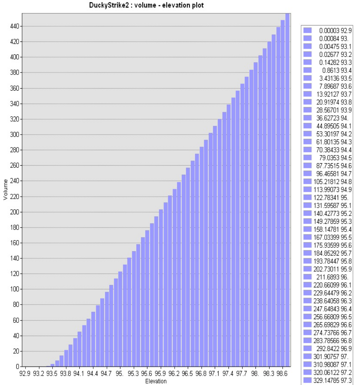
Figure 3.13. Volume – elevation plot for Ducky Strike Duck Club (South pond) obtained from a motorized GPS survey during 2007.
