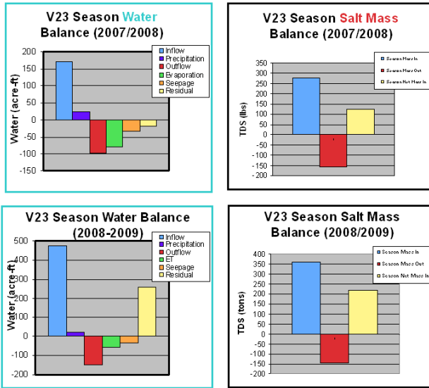
Figure 4.13. Water and salt balance for the Volta 23 wetland.
