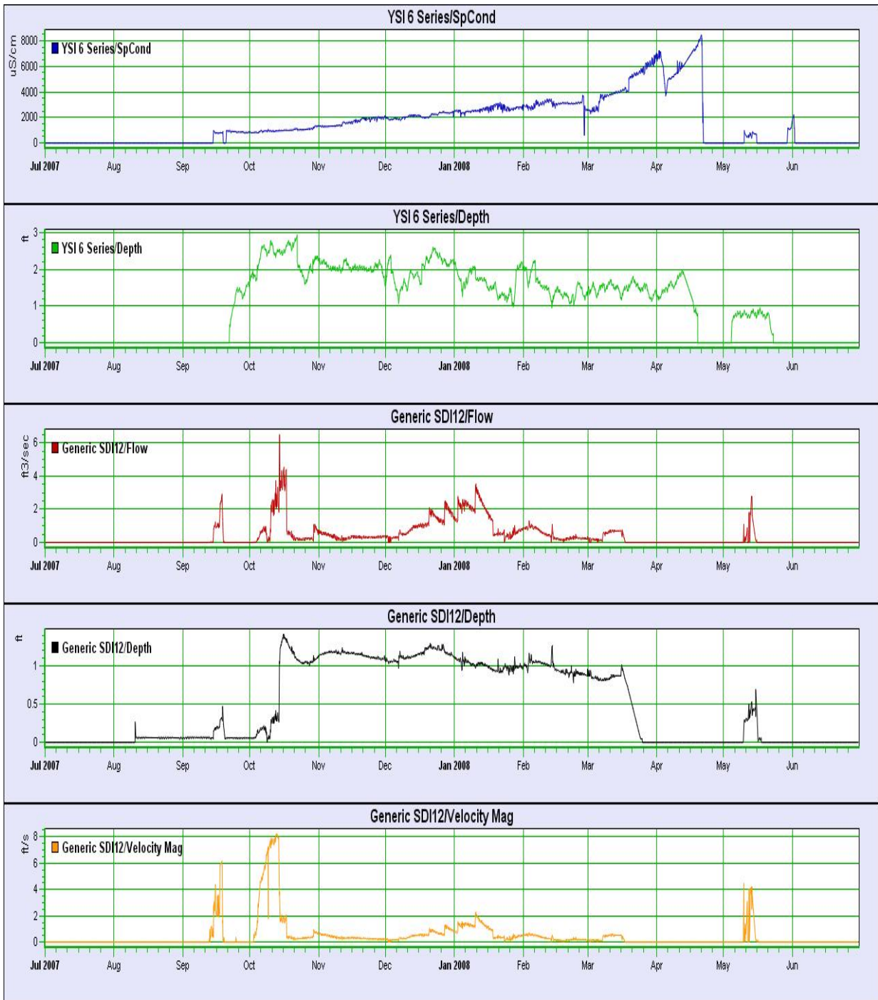
Figure 3.8. Example of the Aquarius data plots used in the data review sessions involving Grassland Water District, Berkeley National Laboratory and California Department of Fish and Game employees. Having multiple sensor values shown on a single plot helps to troubleshoot sensor problems.
