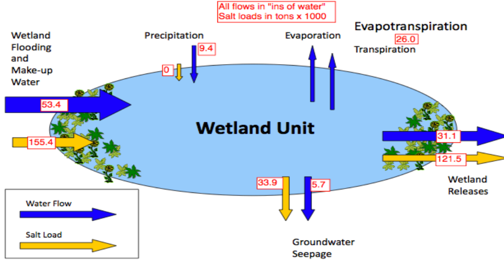
Figure 4.3 Graphical schematic of conceptual water and salinity mass balance (budget).
