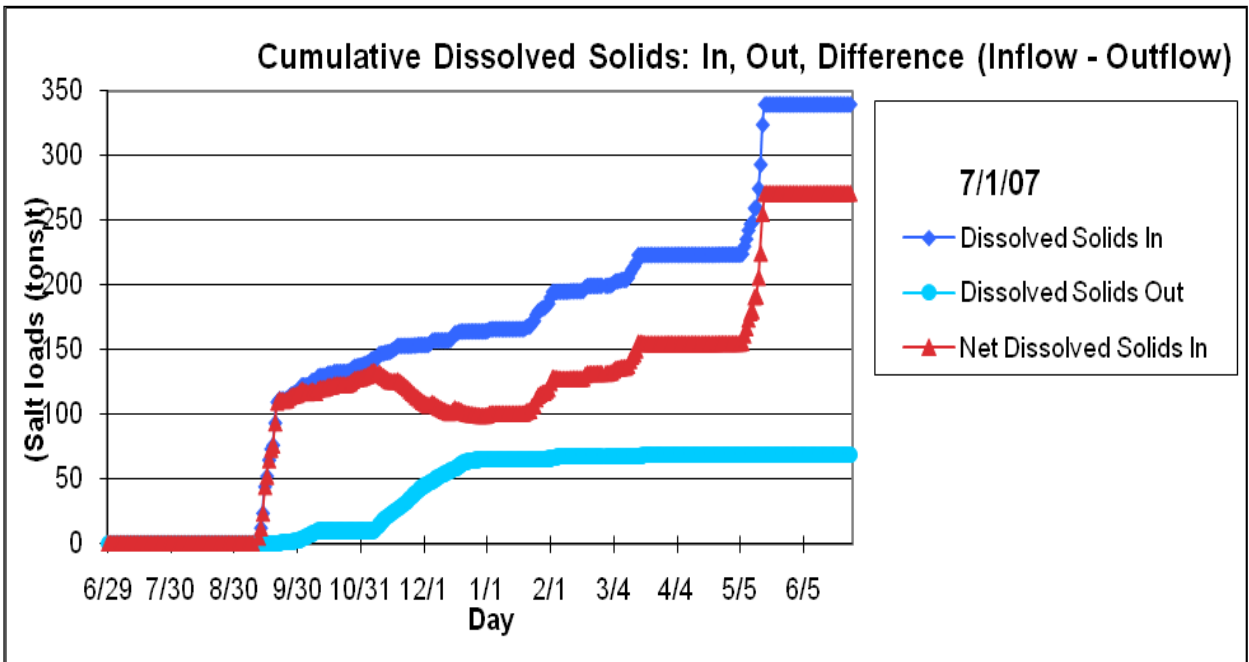
Figure 4.6. Spreadsheet model output showing cumulative flow and salt loading into and out of individual ponds over the 2006/2007 season. The outflow data was compromised at several of the pond sites owing to lack of consistent record keeping by ditch tenders. This problem was resolved by the installation of acoustic flow sensors at the inflow sites during 2007/2008 and 2008/2009 wetland flooded seasons.
