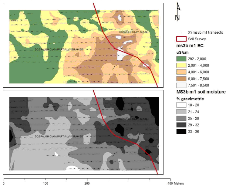
Figure 6.9. Mud Slough 3b May 21, 2008 calibrated EC 1:2 map (top) and calibrated soil moisture map (bottom) visually illustrating the relationship between soil moisture and bulk soil EC.
