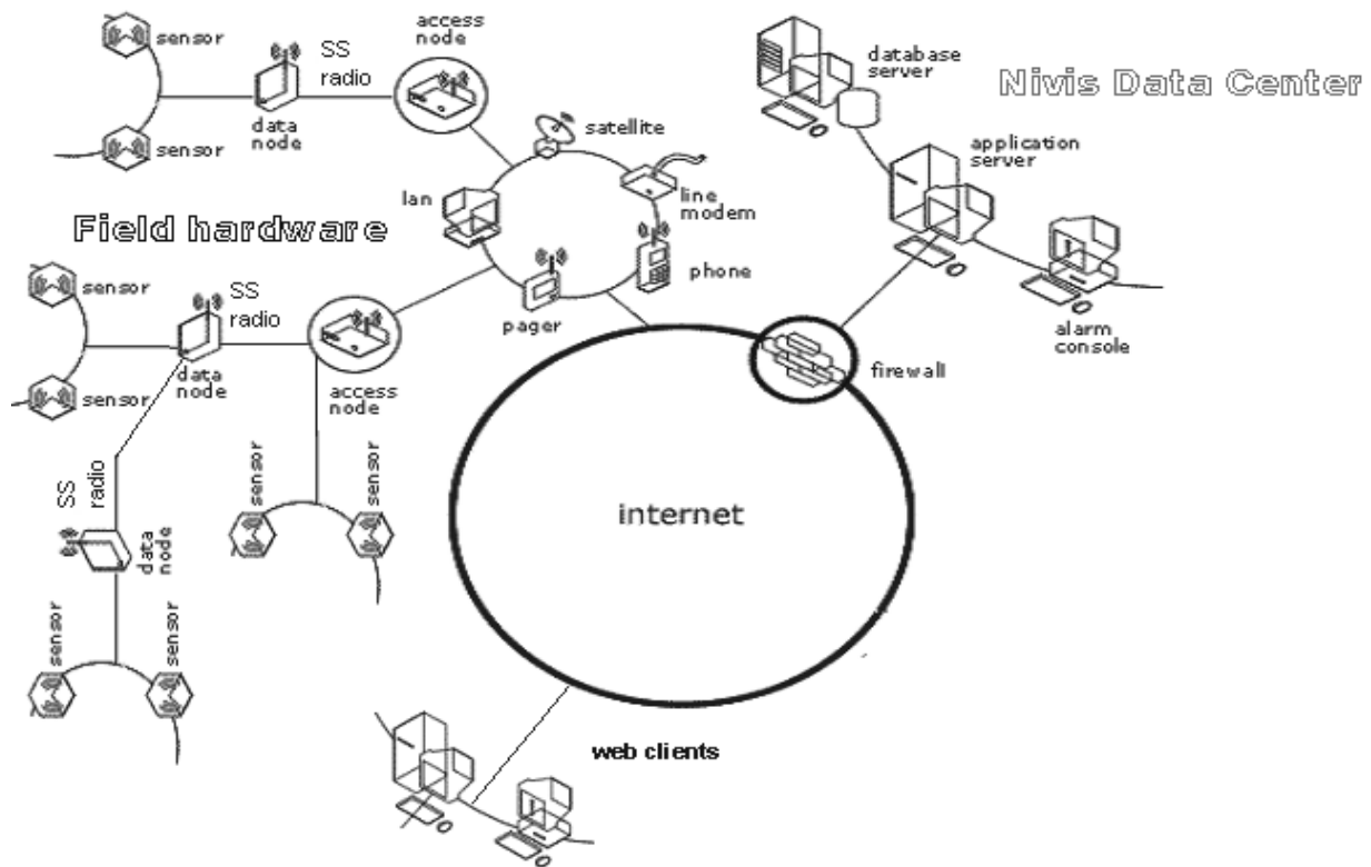
Figure 3.1 Sensor network architecture using YSI-EcoNet. Sensors are connected to dataloggers at either data node (RF telemetry) or Access Node (CDMA telemetry) sites. All data is reported to the NIVIS data server which polls each station at 15 minute intervals. The NIVIS server allows users to customize graphical data output from the monitoring stations.
