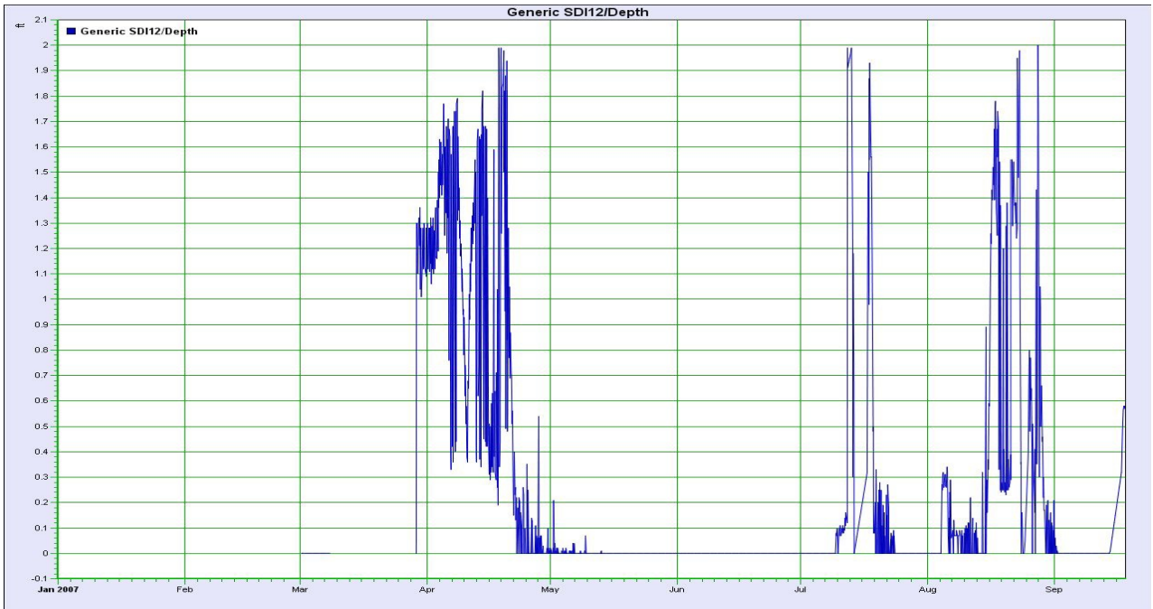
Figure 3.6. YSI sensor time series depth readings at Ducky Strike South. Smoothing algorithms in Aquarius were applied to reduce some of the noise in the data. YSI sondes are unvented and can be affected by changes in atmospheric pressure. Barometric data for the watershed used to make corrections to the YSI stage data to account for weather related shifts in barometric pressure.
