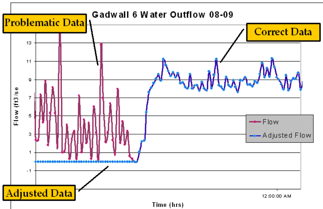
Figure 4.2. Example of adjustments made to MACE flow data to correct for sensor noise and match monitoring site QA data.
