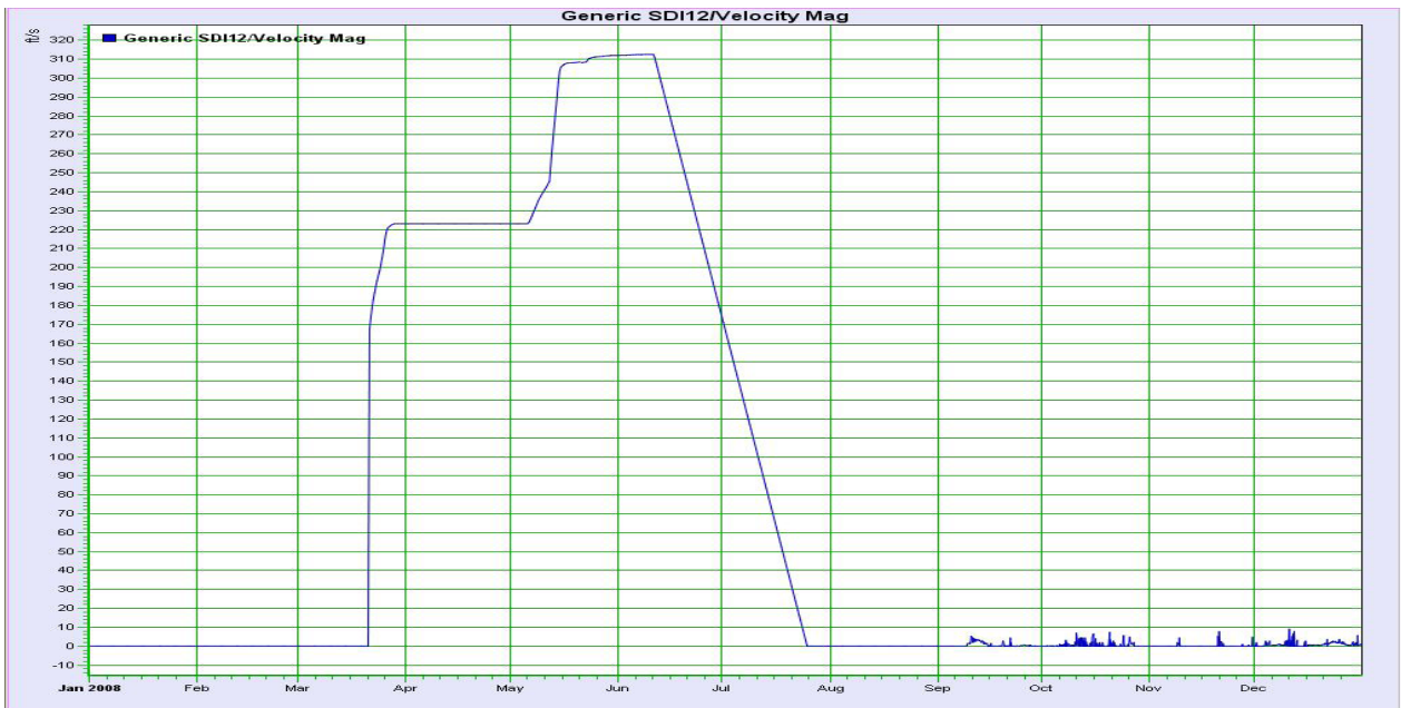
Figure 3.7. MACE velocity data for 2008 after spring drawdown in late March. High velocity data is an artifact of high temperatures combined with the loss of water head above the acoustic sensor. In early September the introduction of flow produces velocity values between 0 and 10 ft/sec.
