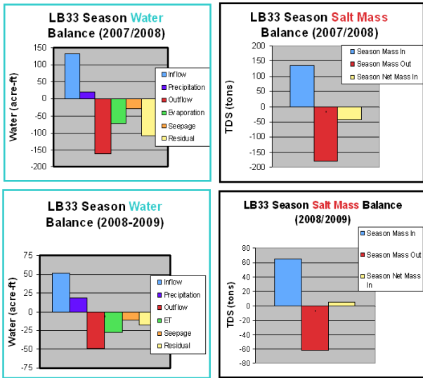
Figure 4.11. Water and salt balance for the Los Baños 33 wetland.
