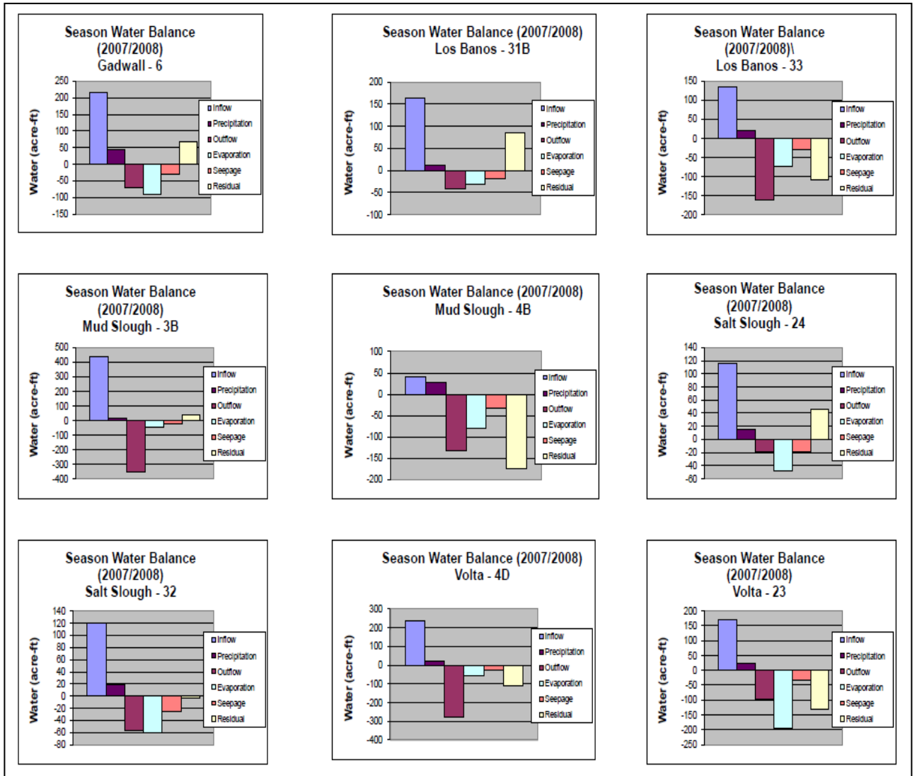
Figure 4.7. Summary water balances for all sites for the 2007/2008 flood-up season. Complete hydrologic balances were not possible at all twelve sites owing to sensor failure at certain pond sites which compromised the completeness of the hydrology and salinity mass balances.
