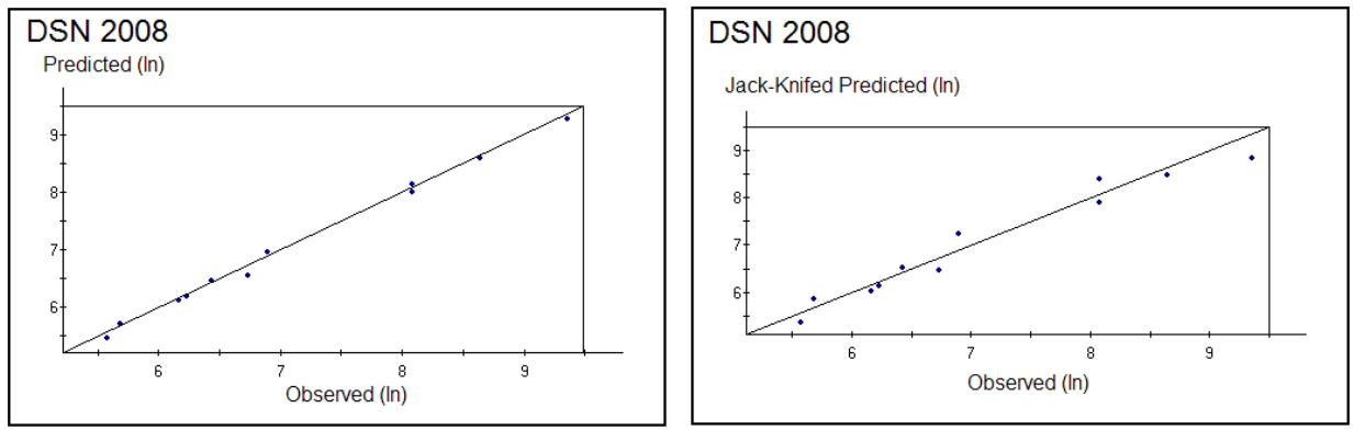
Figure 6.12. Ducky Strike North – model results comparing observed data to model predictions.
