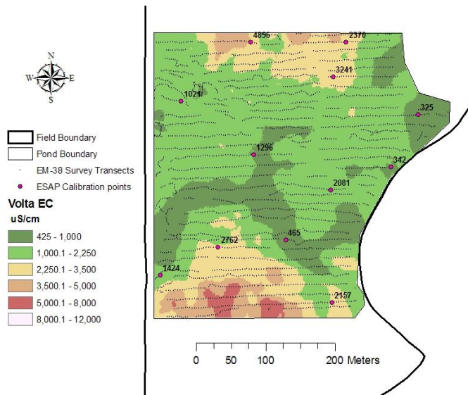
Figure 6.18. Volta 23 calibrated EC1:2 maps of surface bulk soil salinity, 0 – 30 cm.
