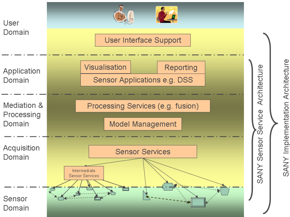
Figure 3.3. Conceptual model of the functional domains of a sensor network (Uslander, 2007)
