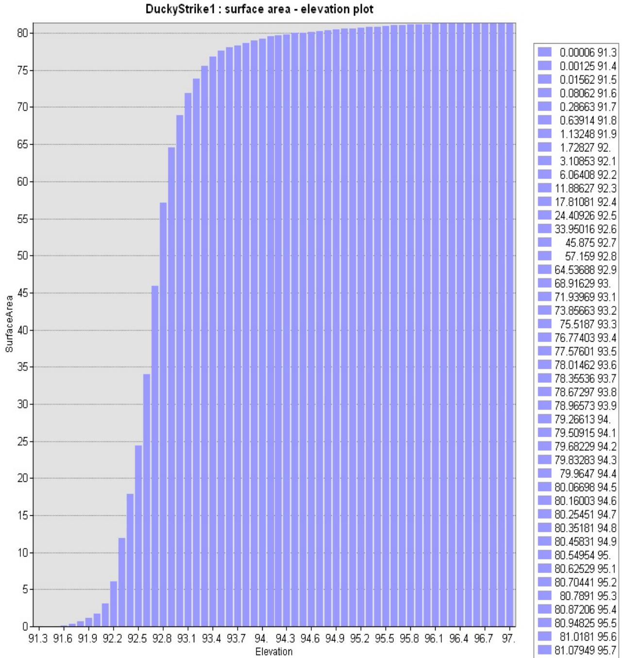
Figure 3.10. Surface-area –elevation plot for Ducky Strike Duck Club (North pond) obtained from a motorized GPS survey during 2007 .
