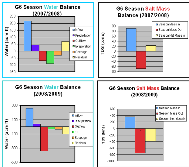
Figure 4.9. Water and salt balance for the Gadwall 6 wetland.
