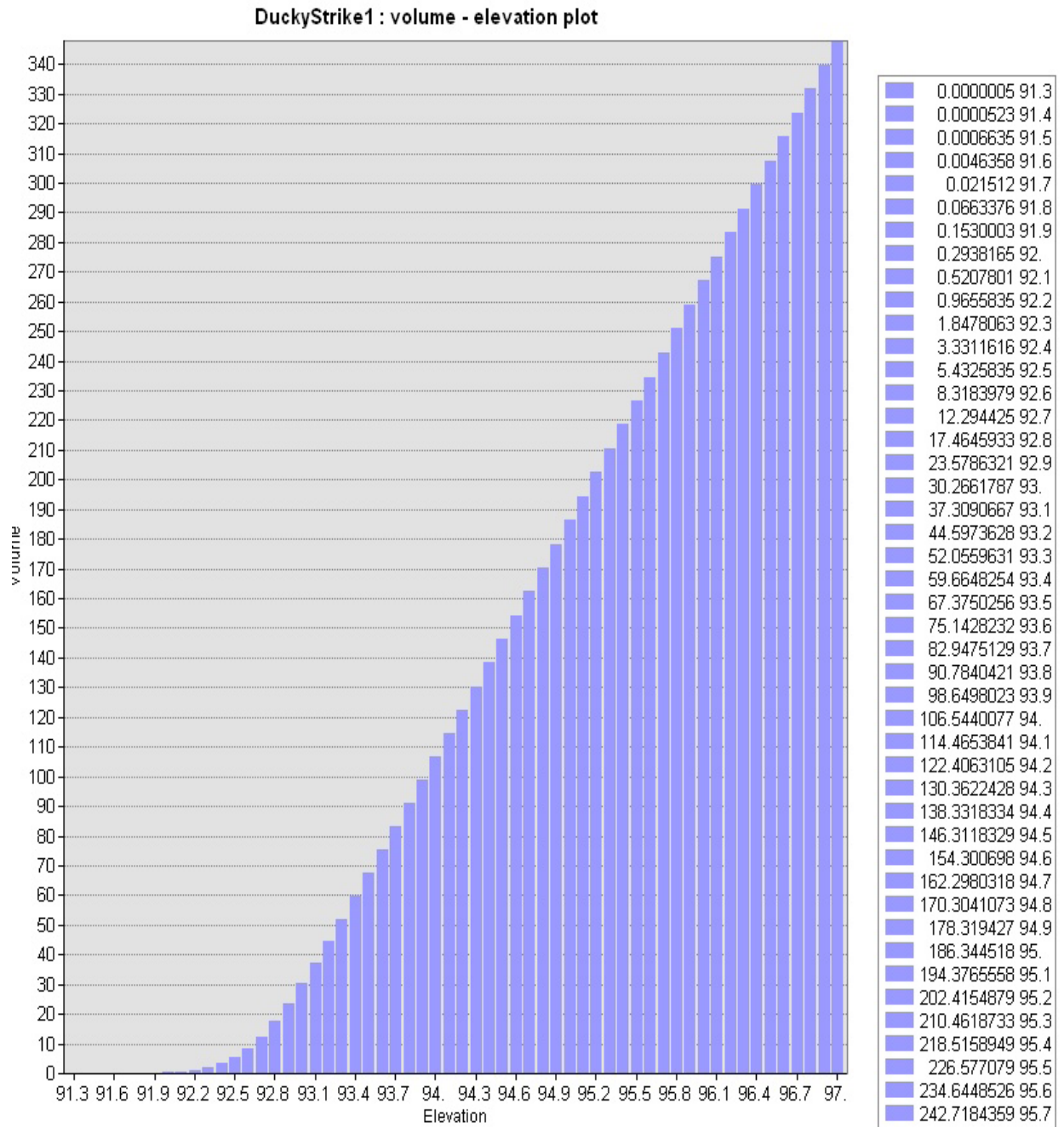
Figure 3.12. Volume – elevation plot for Ducky Strike Duck Club (North pond) obtained from a motorized GPS survey during 2007 .
