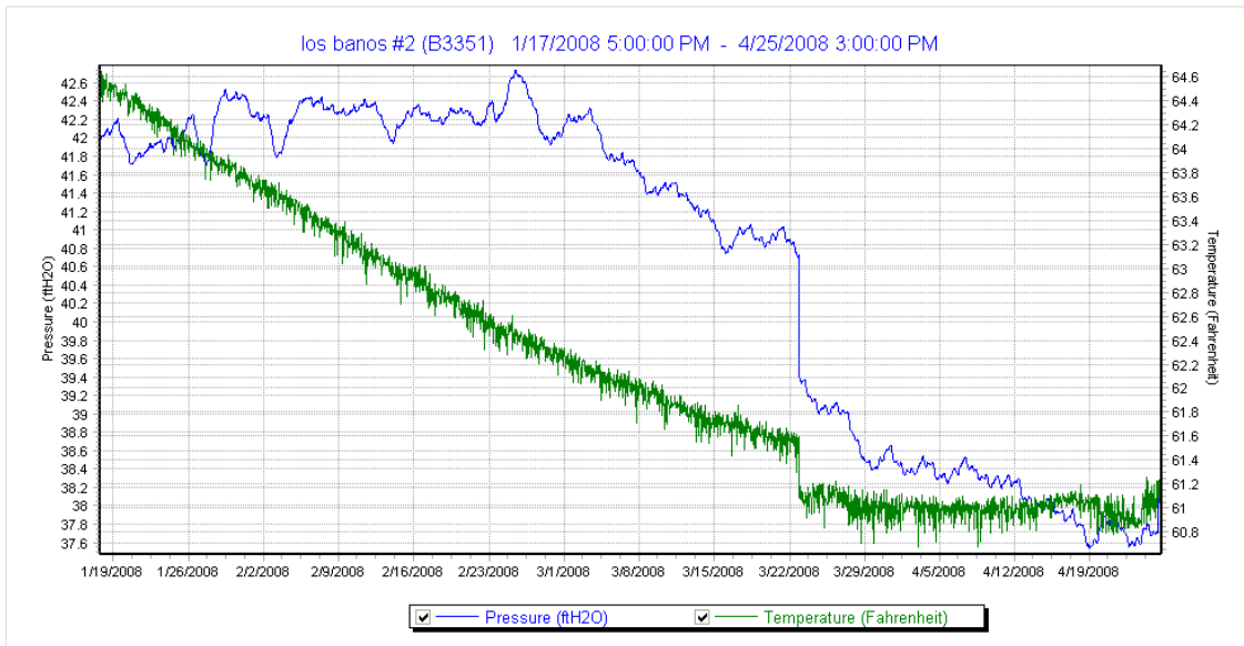
Figure 4.5. Groundwater elevations (not corrected for barometric pressure) within the Los Banos Wildlife Management Area. Well elevations drop rapidly immediately after ponded water is drained and then decline gradually over the remainder of the summer until fall flood-up.
