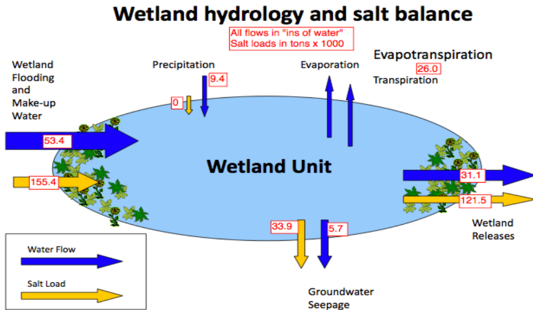
Figure 1.4 Conceptual salt balance model for Grassland Water District using year 2000 data and Level II water supply (Quinn, 2004).
