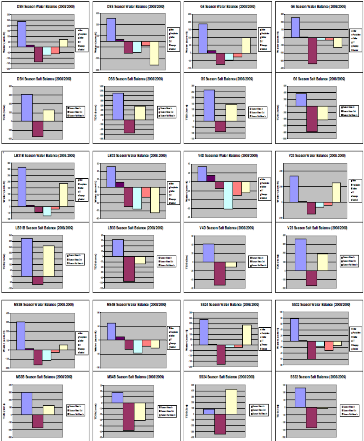
Figure 1.6 Summary water and salt balances for all sites for the 2008/2009 flood-up season. By 2007/2008 the majority of the sensor problems had been solved and the water and salt balances were completed for all sites.
