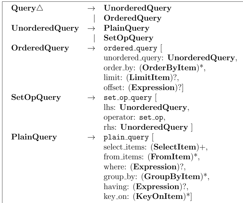
Figure 4.3: AST (queries)
