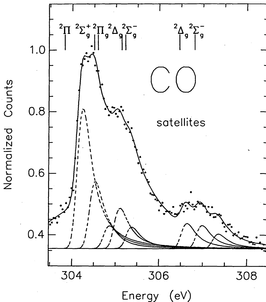
FIGURE 2.6 ZKE spectrum of the satellite region of CO: The solid line is a fit to the data points. The individual peaks are shown with the dashed lines. The calculated energies of Angonoa et. al. 11 are shown at the top of spectrum. These energies are calibrated to the experimental high incident photon energy results of Gelius. 8 As in figure 2.4, these energies correspond to the peak thresholds not the maxima, because of PCI.
