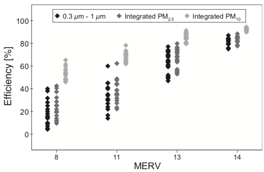
Figure 8: PM 2.5 Removal Efficiency of Various MERV8 and MERV13 Air Filters
