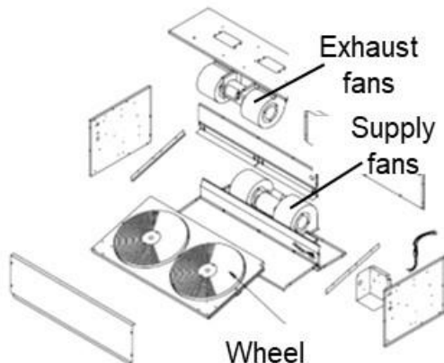
Figure E-2: ERV components
