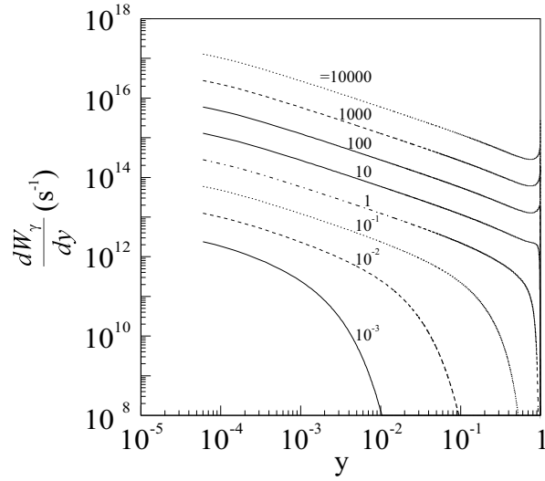
FIG. 1. Sokolov-Ternov spectrum. The energy of the electron beam is 2.5 TeV. From bottom to top, \Upsilon parameters are 10^{-3} , 10^{-2} , 10^{-1} , 1 , 10 , 100 , 1000 , 10000 , respectively.
