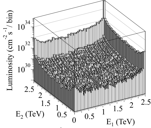
FIG. 10. The e^+e^- luminosity distribution of a 5 TeV e^+e^- linear collider with \Upsilon = 631 . The vertical axis is d^2L_{e^+e^-}/dE_1dE_2 in units of \text{cm}^{-2}\text{s}^{-1}/\text{bin} . The bin size is 50 GeV \times 50 GeV.
