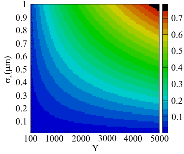
FIG. 3. Relative energy loss distribution as a function of \Upsilon and \sigma_z . The energy of the electron beam is 2.5 TeV.
