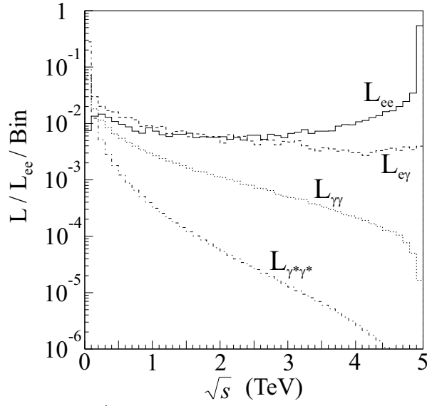
FIG. 9. Luminosity distribution of a 5 TeV e^+e^- linear collider with \Upsilon = 631 . The vertical axis is normalized by the total luminosity of the e^+e^- collisions. The bin size is 100 GeV.
