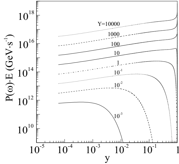
FIG. 2. Sokolov-Ternov power spectrum. The energy of the electron beam is 2.5 TeV. From bottom to top, \Upsilon parameters are 10^{-3} , 10^{-2} , 10^{-1} , 1 , 10 , 100 , 1000 , 10000 , respectively.
