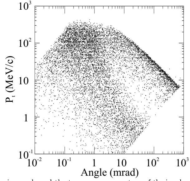
FIG. 8. Scatter plot of the scattering angle and the transverse momentum of the incoherent pairs. The one dot exhibits one real particle.
