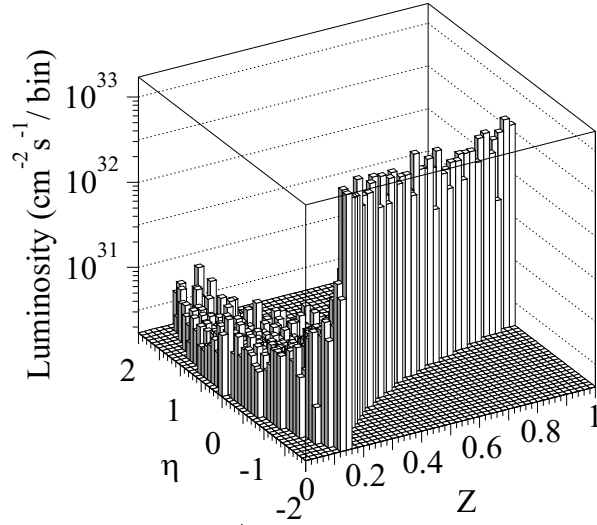
FIG. 13. The e\gamma luminosity distribution of a 5 TeV e^+e^- linear collider with \Upsilon = 631 . The vertical axis is d^2L_{e\gamma}/dzd\eta in units of \text{cm}^{-2}\text{s}^{-1}/\text{bin} . The bin size \Delta z \times \Delta\eta is 0.02 \times 0.1 .
