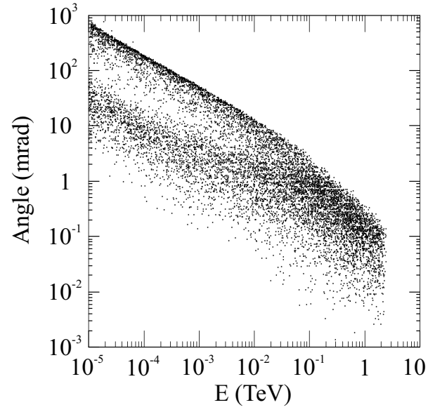
FIG. 7. Scatter plot of the energy and the scattering angle of the incoherent pairs. The one dot exhibits one real particle.
