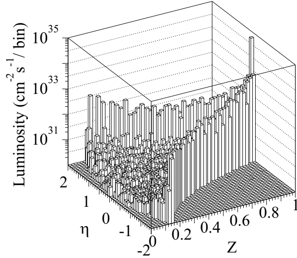
FIG. 11. The e^+e^- luminosity distribution of a 5 TeV e^+e^- linear collider with \Upsilon = 631 . The vertical axis is d^2 L_{e^+e^-}/dzd\eta in units of \text{cm}^{-2}\text{s}^{-1}/\text{bin} . The bin size \Delta z \times \Delta \eta is 0.02 \times 0.1 .
