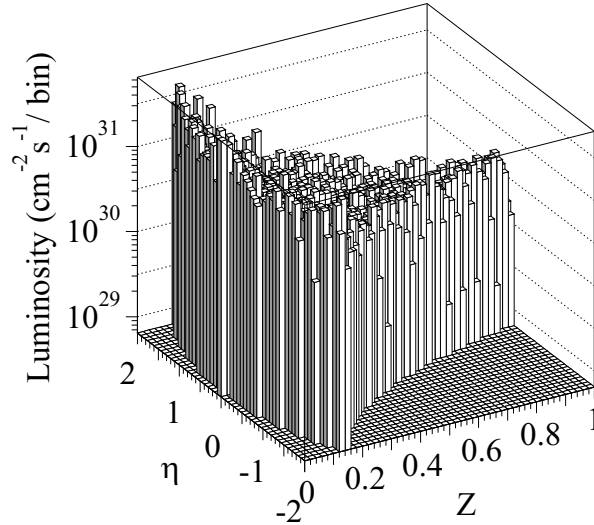
FIG. 15. The \gamma\gamma luminosity distribution of a 5 TeV e^+e^- linear collider with \Upsilon = 631 . The vertical axis is d^2L_{\gamma\gamma}/dzd\eta in units of \text{cm}^{-2}\text{s}^{-1}/\text{bin} . The bin size \Delta z \times \Delta \eta is 0.02 \times 0.1 .
