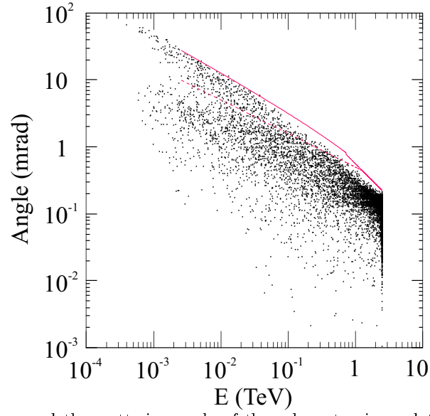
FIG. 5. Scatter plot of the energy and the scattering angle of the coherent pairs and the initial beam particles. The one dot exhibits 15000 real particles. The solid and dashed lines indicate the maximum angles of the opposite and same charge particles in Eqs.(10) and (9).
