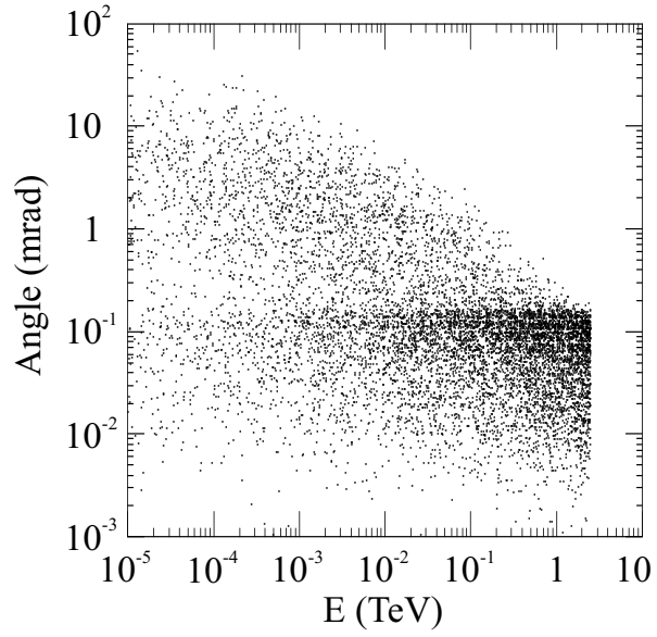
FIG. 4. Scatter plot of the energy and the scattering angle of the photons. The one dot exhibits 15000 real particles.
