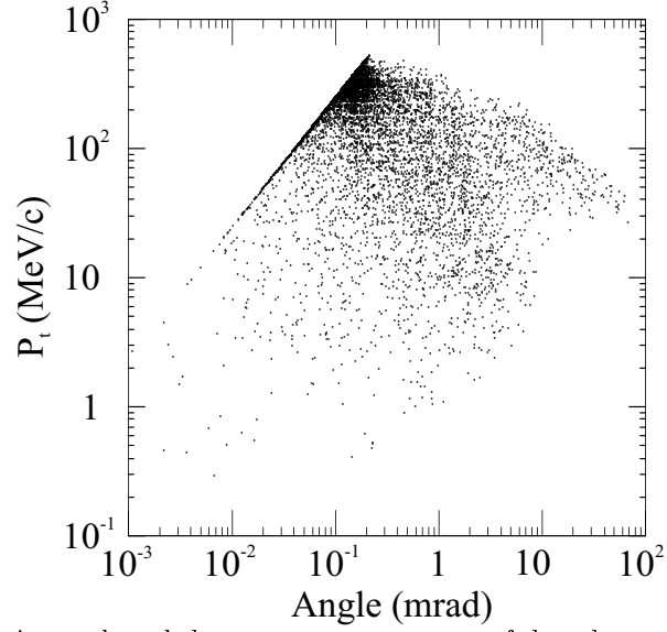
FIG. 6. Scatter plot of the scattering angle and the transverse momentum of the coherent pairs and the initial beam particles. The one dot exhibits 15000 real particles.
