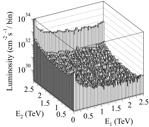
FIG. 12. The e\gamma luminosity distribution of a 5 TeV e^+e^- linear collider with \Upsilon = 631 . The energies of the photon and the electron are E_1 and E_2 , respectively. The vertical axis is d^2 L_{e\gamma}/dE_1 dE_2 in units of \text{cm}^{-2}\text{s}^{-1}/\text{bin} . The bin size is 50 \text{ GeV} \times 50 \text{ GeV} .
