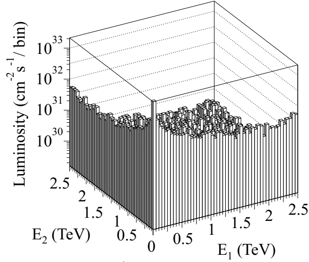
FIG. 14. The \gamma\gamma luminosity distribution of a 5 TeV e^+e^- linear collider with \Upsilon = 631 . The vertical axis is d^2L_{\gamma\gamma}/dE_1dE_2 in units of \text{cm}^{-2}\text{s}^{-1}/\text{bin} . The bin size is 50 \text{ GeV} \times 50 \text{ GeV} .
