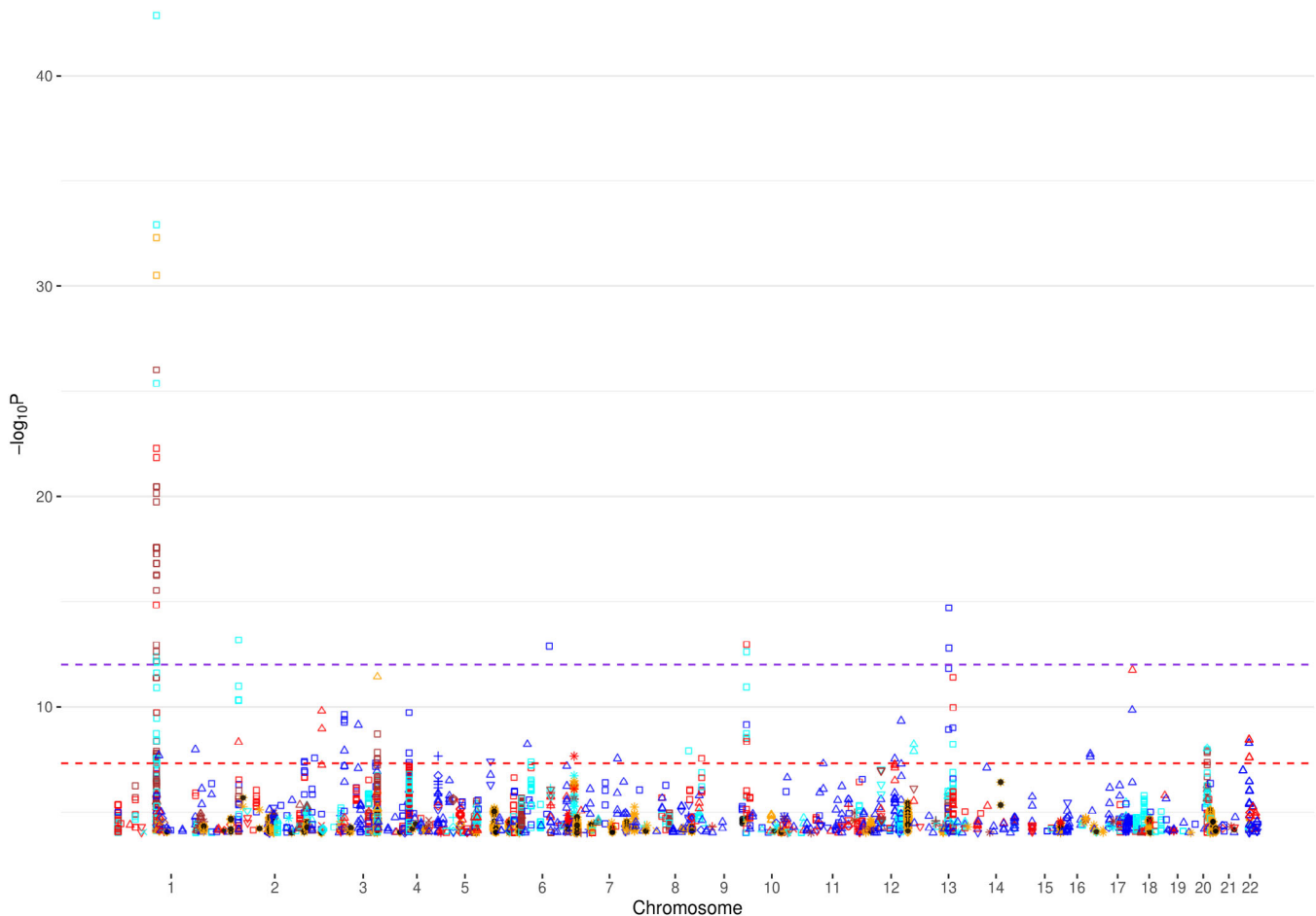
FIGURE 1 Manhattan plot for chromosomes 1–22 for PTSD. ● denotes reported signals from the original GWAS and the remain symbols and colors denote DISTMIX2 imputed signals. Among imputed signals blue denotes \text{info} < 0.2 , red denotes 0.2 < \text{info} < 0.4 , cyan denotes 0.4 < \text{info} < 0.6 , brown denotes 0.6 < \text{info} < 0.8 , orange denotes \text{info} > 0.8 , □ denotes \text{MAF} < 0.05\% , △ denotes 0.05\% < \text{MAF} < 0.5\% , ▽ denotes 0.5\% < \text{MAF} < 1\% , + denotes 1\% < \text{MAF} < 2\% , ◇ denotes 2\% < \text{MAF} < 5\% , x denotes 5\% < \text{MAF} < 10\% and * denotes 10\% < \text{MAF} < 50\% . The red line is the default genome-wide threshold of p = 5 * 10^{-8} , which is applicable common SNPs with moderate to large Info values. The purple line at p = 10^{-12} is the threshold to be used for rare and/or low Info variants. GWAS, genome-wide association studies; MAF, minor-allele frequency; PTSD, post-traumatic stress disorder; SNPs, single nucleotide polymorphisms [Color figure can be viewed at wileyonlinelibrary.com ]
