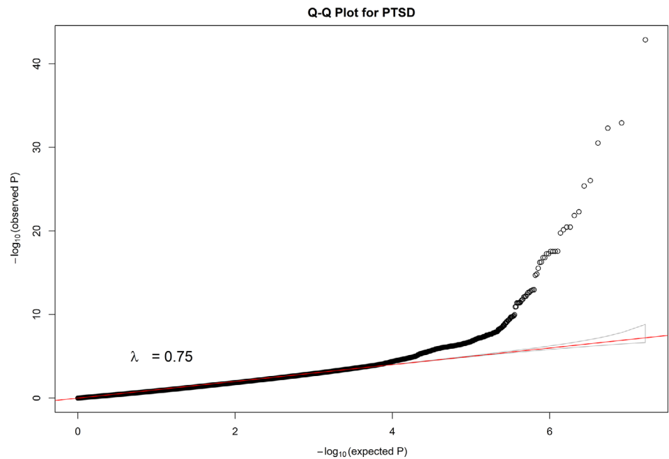
FIGURE 3 Q-Q plot for all SNPs of imputed PTSD GWAS. GWAS, genome-wide association studies; PTSD, post-traumatic stress disorder; SNPs, single nucleotide polymorphisms [Color figure can be viewed at wileyonlinelibrary.com ]
