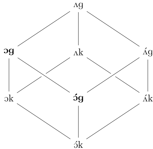
Figure 2.1: Hasse diagram of composite and concrete URs for the paradigm containing ɔk and ʌg-á. The composite URs that can support the observed alternations are bolded.
