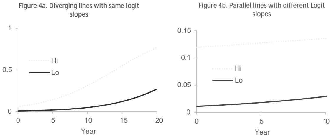
Figure 4. Examples of inconsistency between divergence in linear and log-odds space
