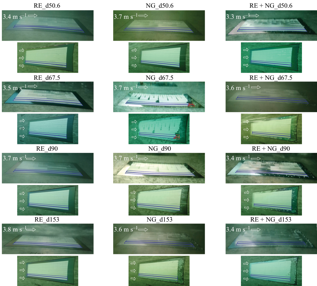
Figure 10. Sample images at speeds in the range 3.3–3.8 m s -1 . Blue indicates a pinned or slightly depinned interface (i.e. h/w \leq 0.17 ); yellow indicates a depinned interface (i.e. 0.17 < h/w < d/w ); and red indicates a no interface (i.e. h/w = d/w ).
