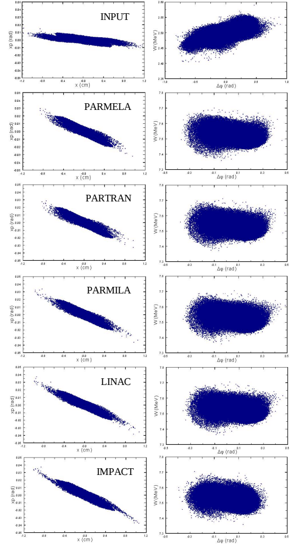
Figure 2. Transverse ( x - x' ) and longitudinal ( w - \phi ) phase space plots at the input and output from different codes.
