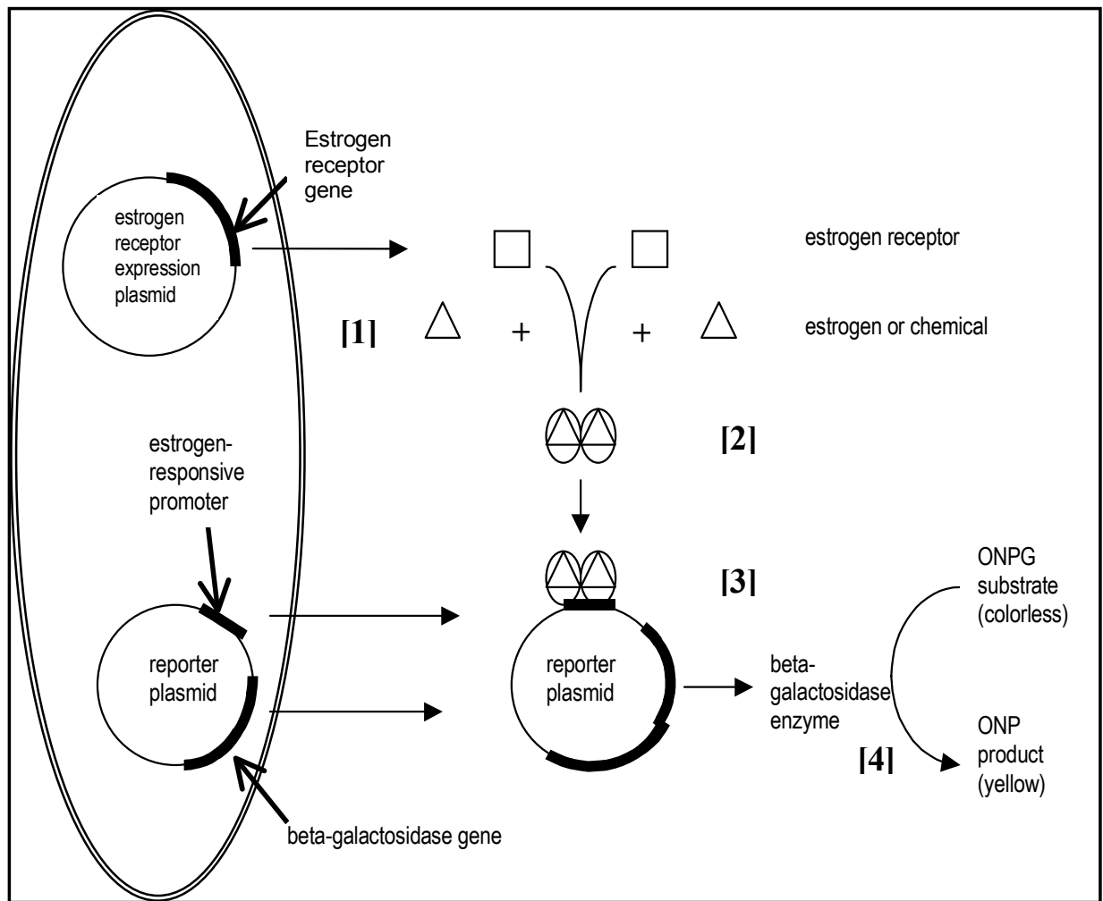
Fig. 1: Yeast-based estrogen receptor assay (Adapted from Activities Feb 1997)
