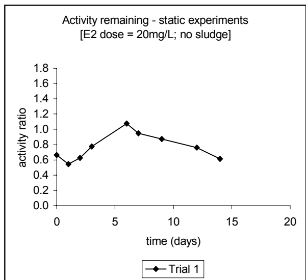
Fig. 3: Removal of total estrogenic activity over time with a 20mgE2/L dose. Note that samples with activated sludge (AS) showed some reduction of measured activity with time after 7-8 days although measured activity remains high.
