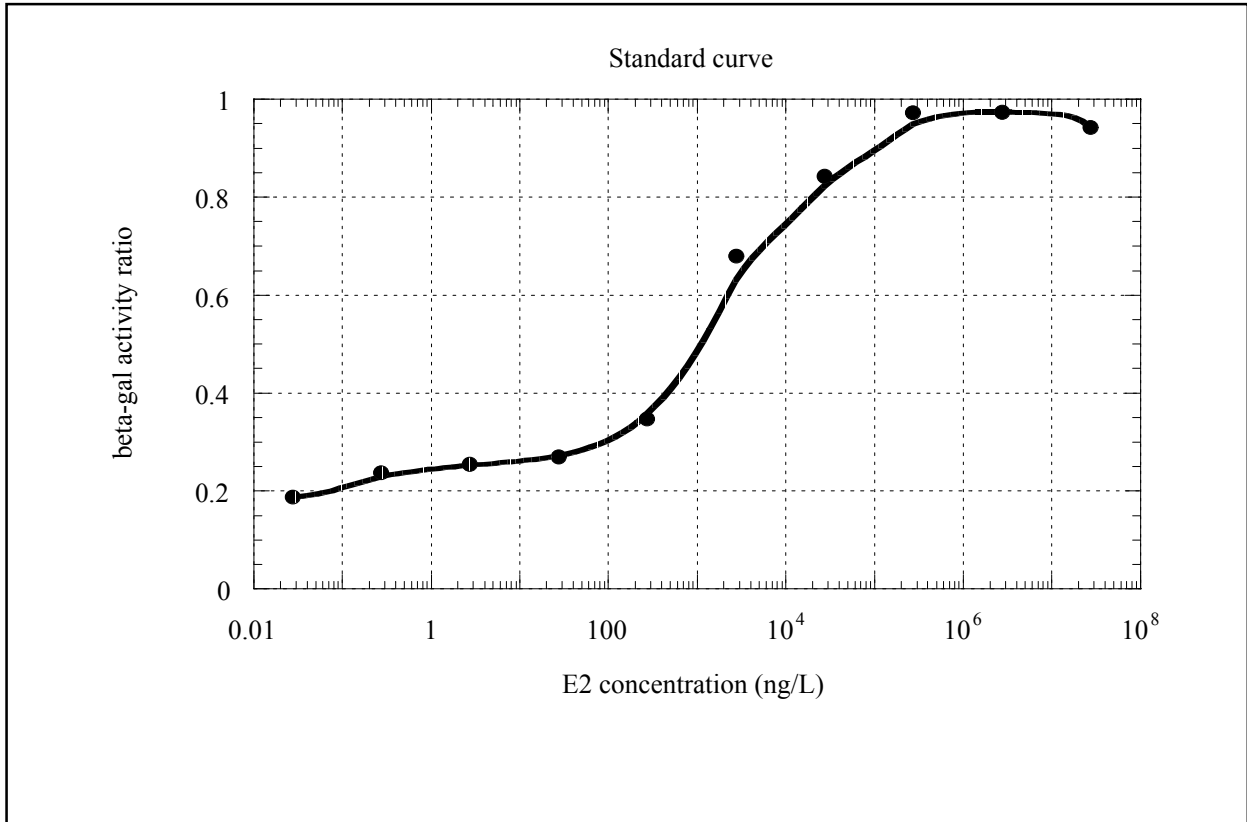
Fig. 2: Standard dose-response curve.
