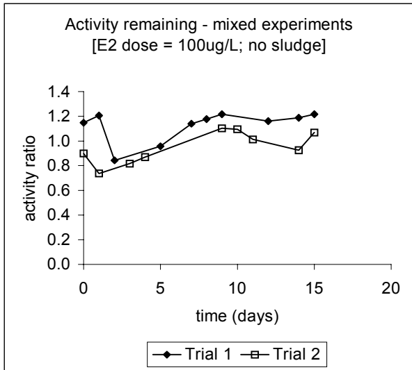
Fig. 4: Removal of total estrogenic activity over time with a 100µgE2/L (0.1mg/L) dose. Note that samples with activated sludge (AS) showed some reduction of measured activity with time after 8-10days, while experiments with no sludge showed little removal over time. Re-spiked sludge did not show maximum activity, implying more ready removal.
