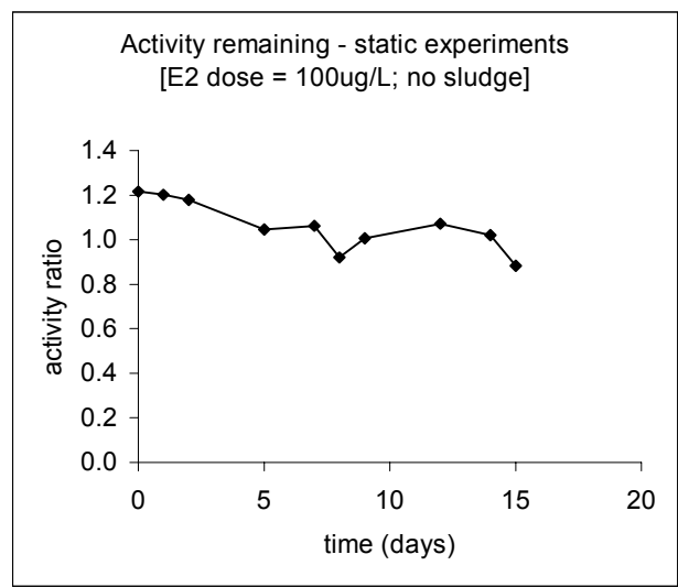
Fig. 4: Removal of total estrogenic activity over time with a 100µgE2/L (0.1mg/L) dose. Note that samples with activated sludge (AS) showed some reduction of measured activity with time after 8-10days, while experiments with no sludge showed little removal over time. Re-spiked sludge did not show maximum activity, implying more ready removal.
