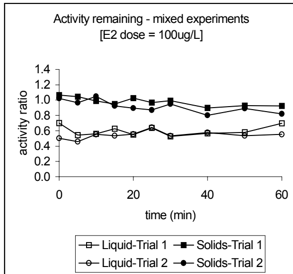
Fig. 5: Estrogenic activity associated with activated sludge solids.
