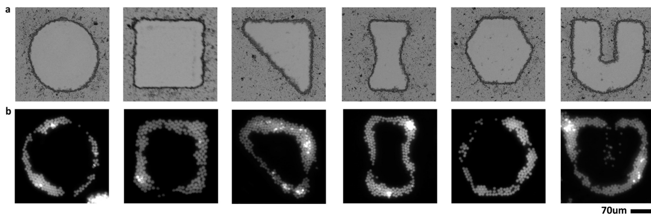
Fig. 3. (a) Arbitrary patterns with a PDMS membrane on top, which were cut within 200 \times 200 \mu\text{m}^2 area. (b) Fluorescence images of patterned 10 \mu\text{m} microparticles in water using CNT-PDMS structures for corresponding shapes. Scale bar, 70 \mu\text{m} .
