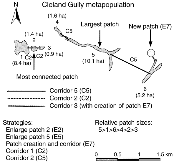
FIG. 2. The Cleland Gully Southern Emu-wren metapopulation, showing size and location of patches and corridors.
