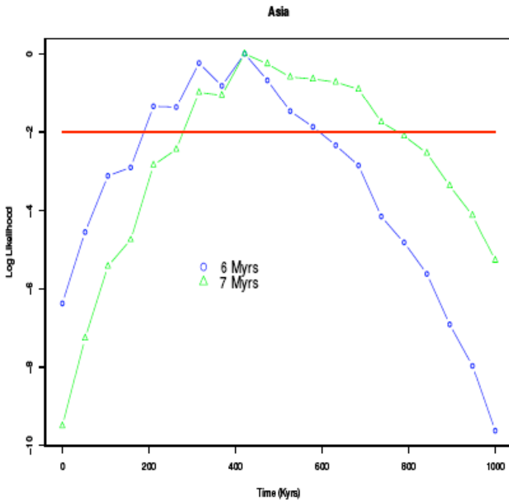
Figure S5. Log likelihood surface for the split time between the ASN population and Neanderthal, assuming two different average TMRCA between human and chimpanzee.
