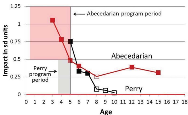
Figure 1. IQ impacts in Perry and Abecedarian.
