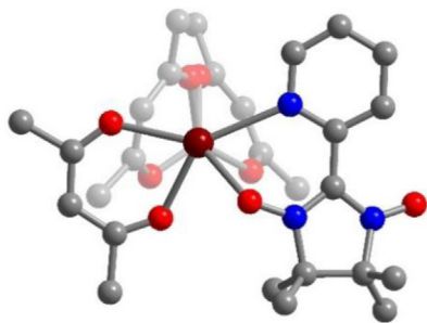
Fig. 20. Structure of \text{Tb}(\text{hfac})_3(\text{NIT2Py}) \cdot \text{C}_6\text{H}_{17} ( 23 ) with dark red, blue, red and gray spheres representing Tb, N, O and C atoms, respectively; H, F atoms, and \text{C}_6\text{H}_{17} are omitted and selected C and O atoms are faded for clarity.
