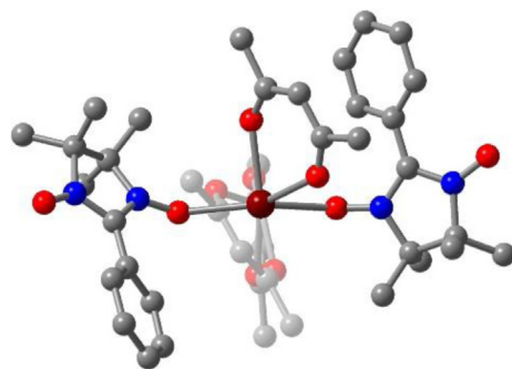
Fig. 21. Structure of \text{Tb}(\text{hfac})_3(\text{NITPhOEt})_2 ( 24 ) with dark red, blue, red and gray spheres representing Tb, N, O and C atoms, respectively; H and F atoms are omitted and selected C and O atoms are faded for clarity.
