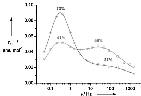
Fig. 15. Out-of-phase susceptibility ( \chi_M'' ) for 16_cr and 16_dis at 258 \text{ K} . The solid lines represent fits.
