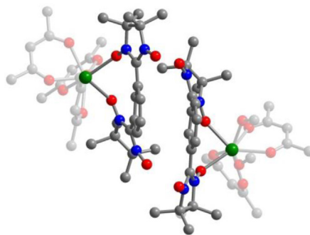
Fig. 22. Structure of \text{Dy}(\text{hfac})_3(\text{NITmbis}) ( 25 ), with green, blue, red and gray spheres representing Dy, N, O and C atoms, respectively; H and F atoms are omitted and selected C atoms are faded for clarity.
