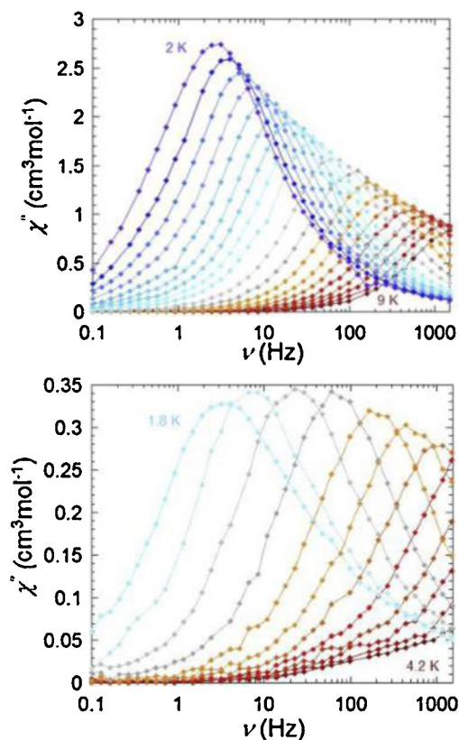
Fig. 8. Variable-frequency ac susceptibility data for [(dmp 2 Nin)Co 2 (N(SiMe 3 ) 2 ) 2 ] - ( 8 ) (top) and [(dmp 2 Nin)Co 2 (N(SiMe 3 ) 2 ) 2 (Et 2 O) 2 ] + ( 10 ) (bottom) collected under a 1200 Oe dc field.
