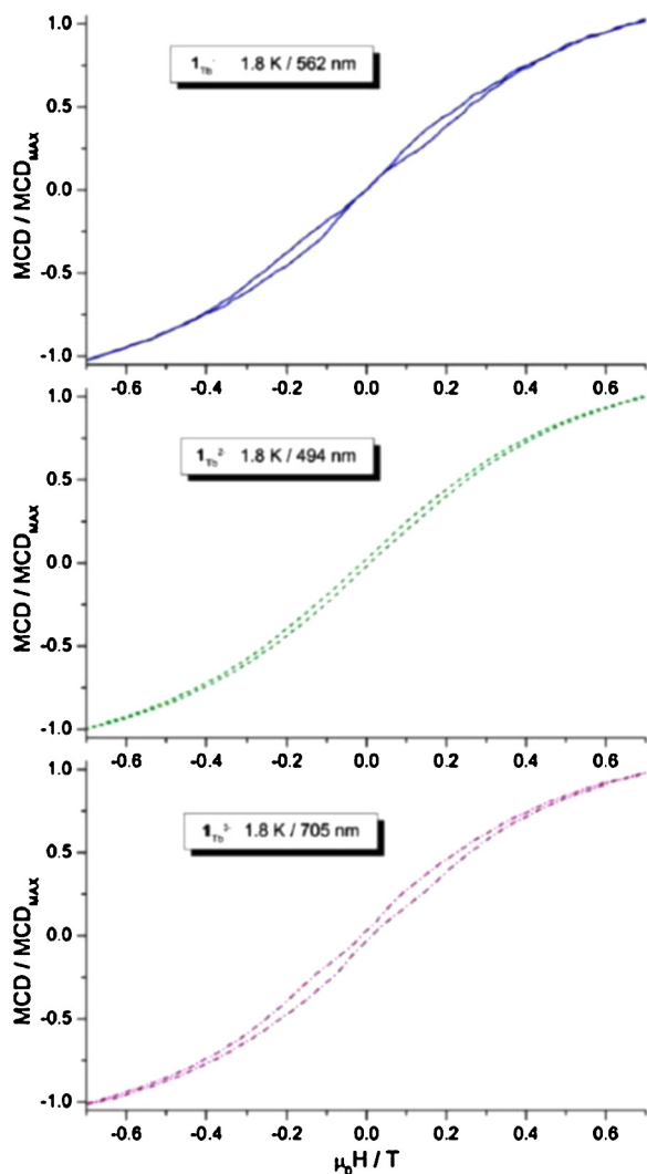
Fig. 14. Hysteresis curves of the normalized MCD intensity recorded at 1.8–1.9 K and at a sweep rate of 1 \text{ T min}^{-1} for 16-1 (top), 16-2 (middle), and 16-3 (bottom). Source: Figure was reproduced from Ref. [229], with permission of the copyright holders.
