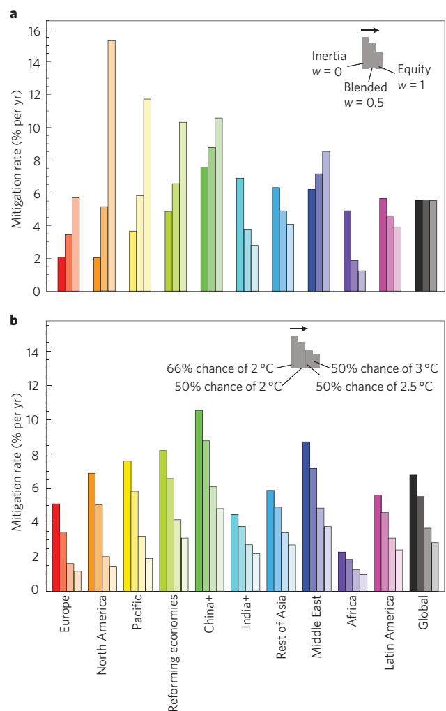
Figure 3 | Dependence of the regional mitigation challenge on the sharing index ( w ) and the warming limit. a , Mitigation rates for 10 regions and the world at w = 0, 0.5 and 1. Available global fossil-fuel combustion and industrial processes (FFI) carbon quota from 2013 is Q_{\text{avail}} = 1,400 Gt CO 2 , corresponding to a 2 °C warming limit with 50% success probability. b , Mitigation rates under a blended sharing principle ( w = 0.5 ) in four cases with warming limit and success probability, respectively, equal to 2 °C and 50%; 2.5 °C and 50%; 3 °C and 50%; and 2 °C and 66%. The available global FFI carbon quotas for these four cases are Q_{\text{avail}} = 1,400, 2,300, 3,200 and 1,100 Gt CO 2 , respectively 10 .
