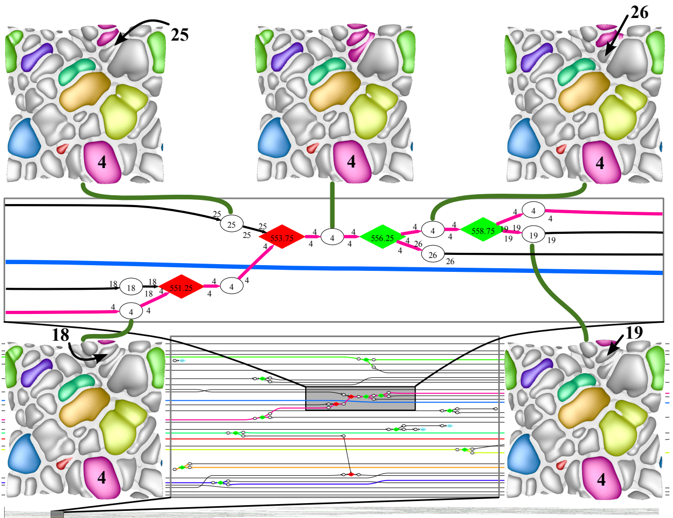
Fig. 11. Subsection of the tracking graph in the turbulence free case compressed to only show the colored arcs together with several corresponding segmentations. Round nodes correspond to cells explicitly segmented by the Morse complex, diamonds to topological events between time steps. Red signifies a merge, green a split, and turquoise a birth/death event.
