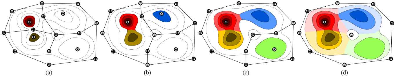
Fig. 3. Using a highest-saddle-first hierarchy to encode all possible cell segmentations: Consider the Morse complex of Fig. 1(a) together with the partial areas shown in Fig. 4(b). The sequence (a)-(d) shows how the burning cell segmentation can be constructed for all thresholds in a single top-to-bottom sweep. Colored portions of the complex are considered above the threshold, white regions below. (a) The segmentation at some initial threshold with two burning cells whose area is given by the sum of the pre-computed areas above the threshold; (b) Lowering the threshold it passes a maximum and a new cell appears (colored blue). Furthermore, the threshold has passed a saddle which is immediately canceled with its lower neighboring maxima (the yellow one). This causes the red and yellow cells to merge restoring the correct cell count for this threshold. The area of the merged cell is computed by simply summing the areas in the corresponding function ranges; (c) Further lowering the function value causes the green cell to appear and the blue one to merge with the red/yellow one. The combined area as before is given as the sum of the pre-computed areas; (d) Finally, lowering the threshold to the lowest contour shown merges the green cell with the rest.
