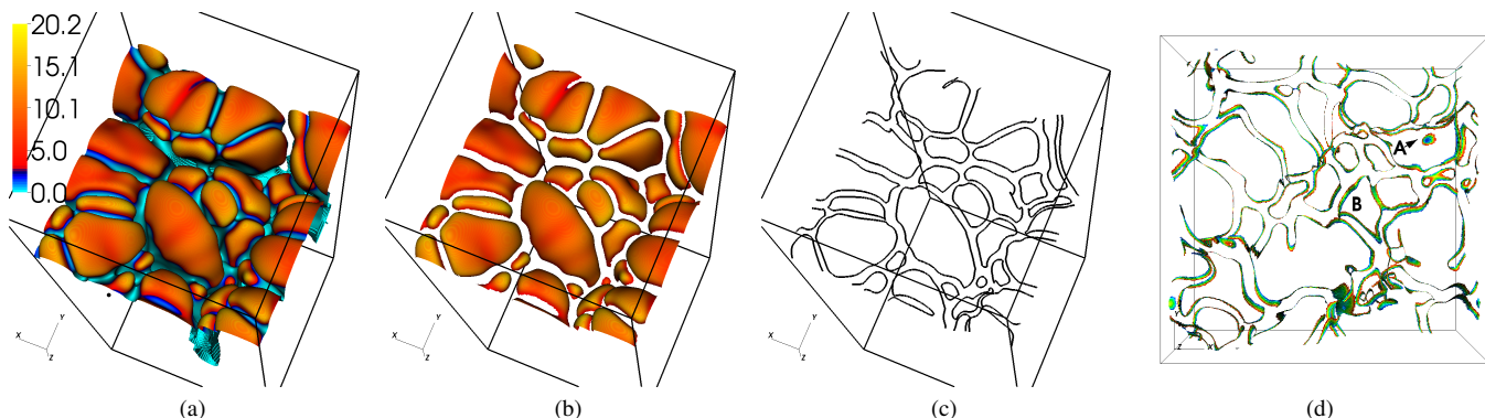
Fig. 5. Tracking burning regions. Like in the cumulative analysis, we restrict our considerations to a particular isotherm (a), on which fuel consumption is mapped as a scalar field. Thresholding triangles of the isotherm by fuel consumption allows identification of individual burning regions (b). We track these individual burning regions by considering their boundaries, which can be obtained in a second contouring operation (c). Traced over time, these boundaries sweep surfaces in 4D space (the figure shows their path in 3D space) (d). The Reeb graph of this time surface is the desired tracking graph.
