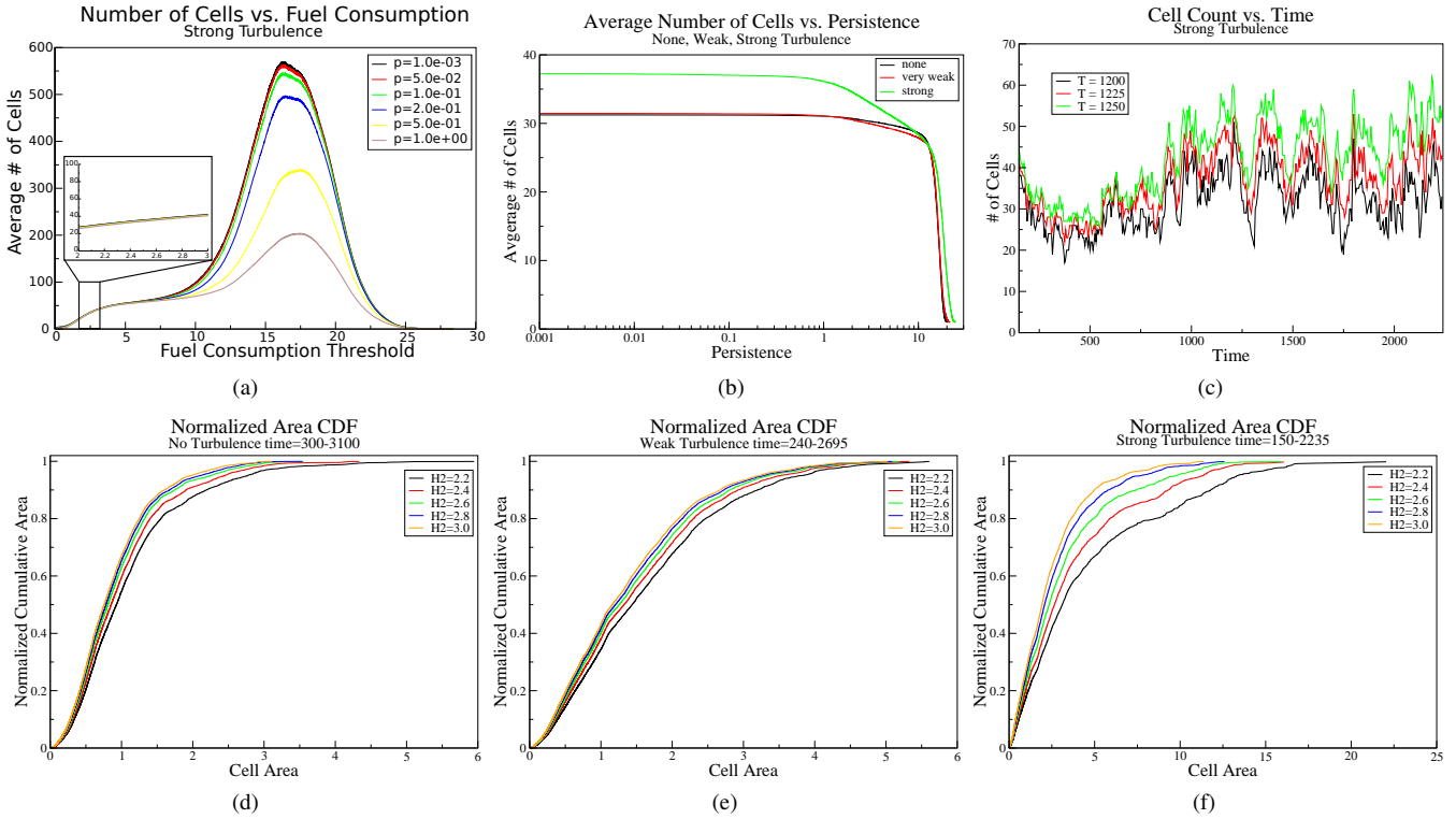
Fig. 9. Parameter study: (a) Average number of cells per time steps depending on the fuel consumption threshold for various persistences; (b) Average number of cells depending on persistence; (c) Number of cells over time for three different temperature value in the strong turbulence case; (d)-(f) Cumulative density function of cell area weighted by overall burning area for various fuel consumption thresholds in the none, weak, and strong turbulence case respectively.
