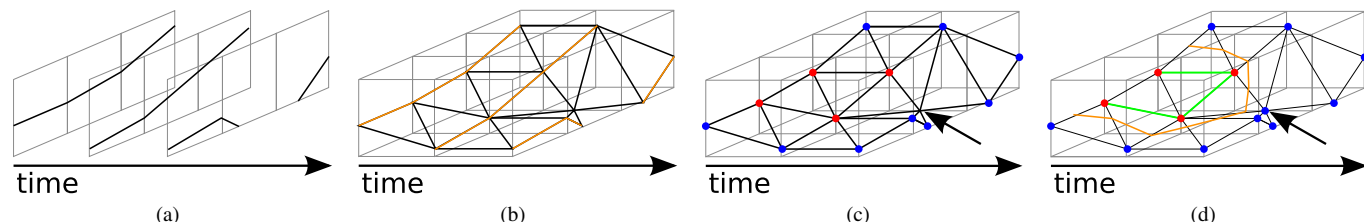
Fig. 6. Tracing the evolution of 2D burning regions and extinction pockets by tracking their boundaries. (a) Input data comes as a set of discrete time slices. (b) Treating time as additional, third dimension we extract a space-time surface correlating isotherms from different time steps. The isotherms (contour lines in 2D) for all original time steps area extracted by selecting all lines that have only vertices in the time step of interest (orange lines). (c) Isotherm vertices at original time steps classified as either burning (red) or non-burning (blue) based on the local fuel consumption rate. Note that vertices between time steps (arrowed vertex) are not classified, yet. (d) Classify vertices between time steps (arrowed vertex) by thresholding and extract boundaries separating burning regions and extinction pockets (orange lines).
