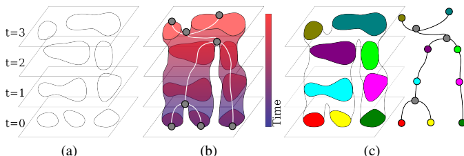
Fig. 7. Using the Reeb graph to compute a tracking graph. (a) Several time steps of a 2D data set with the boundaries of several cells indicated; (b) The space-time boundary created by the boundaries of the cells in (a) as they are interpolated over time. The surface is colored coded using time as function and its Reeb graph is shown in white and gray; (c) Each cell within a time step is assigned a unique identifier which we use to augment the Reeb graph. Note that the final tracking graph still contains nodes between time steps without identifier (shown in gray).
