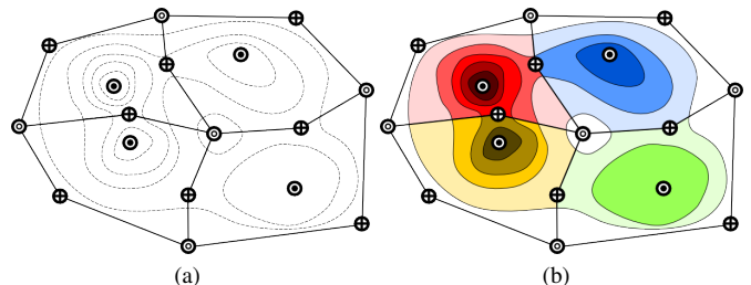
Fig. 4. (a) The Morse complex of Fig. 1(a) with several contours, drawn as dotted lines, indicating the subdivision of the stable manifolds into sub-regions based on function range; (b) The Morse complex of (a) with the partial areas color-coded wrt. their stable manifolds.
