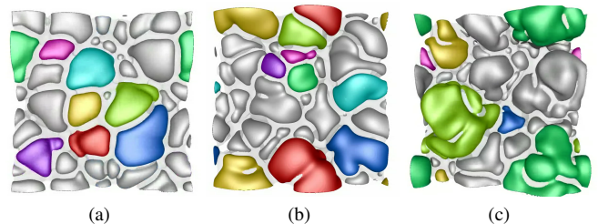
Fig. 13. Snapshots of early time steps in the turbulence free (a), weak (b), and strong turbulence (c) case. Selected burning cells are shown in color, non-selected cells in grey. The non-burning portions of the flame surfaces are drawn translucent. As the turbulence level increases cells become less convex and develop a higher genus.
