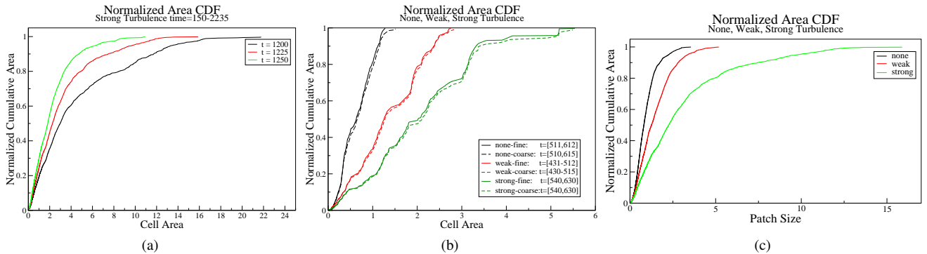
Fig. 12. Parameter study and results: (a) Cumulative density functions of the cell areas weighted by overall burning area for three temperature values in the strong turbulence case; (b) Comparison of the NCDF functions on fine and coarse resolution for all three cases. (c) NCDF function of the cell area distribution. As turbulence increases the distributions skews towards larger cells.
