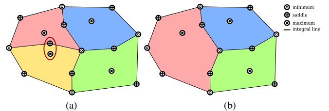
Fig. 1. (a) Example Morse complex with the stable manifolds highlighted; (b) Morse complex of (a) after the cancellation of the marked saddle maximum pair. The two critical point plus their incident integral lines are deleted and two stable manifolds merge.
