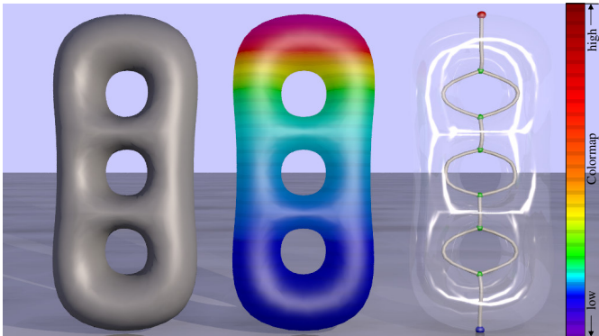
Fig. 2. Reeb graph of the height function on the triple torus. The three loops in the graph correspond to the three tunnels of the model.
