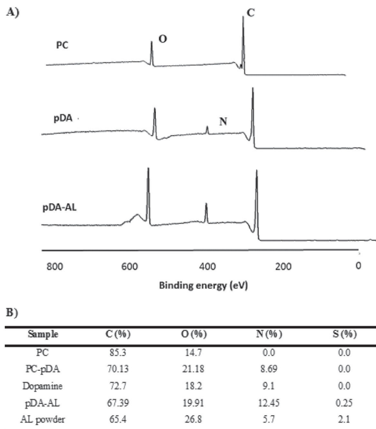
Figure 2. XPS analysis of the polymer surfaces. A) XPS peaks of the unmodified poly carbonate surfaces (PC), polydopamine-coated PC surfaces (PC-pDA), and pDA-coated PC surfaces with immobilized alginate lyase (PC-pDA-AL). B) Quantification of atomic compositions on the polymer surfaces, alginate lyase in powder (AL), and the theoretical composition of dopamine based on its molecular composition.
