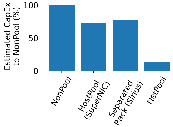
Figure 4.14. The CapEx of different SmartNIC deployment methods.
