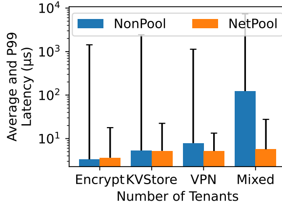
Figure 4.12. Overall Application Latency.
