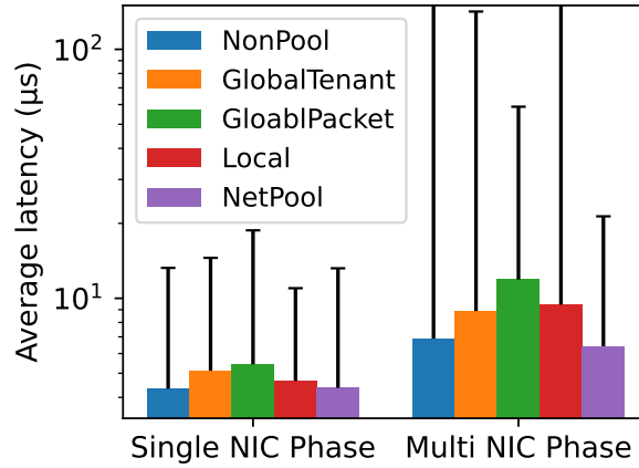
Figure 4.15. Average latency on L7 encryption application.
