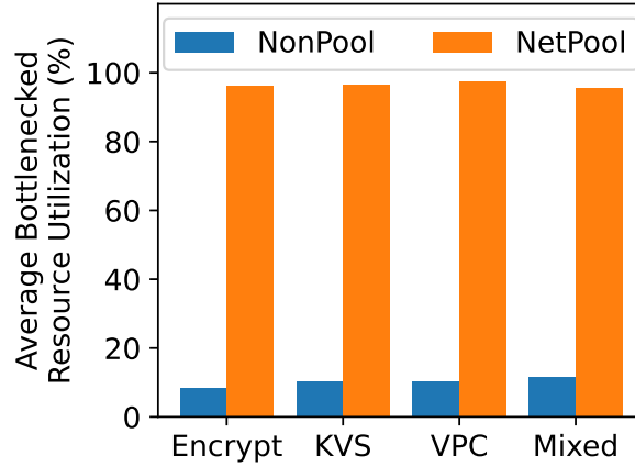
Figure 4.13. The utilization with different applications.
