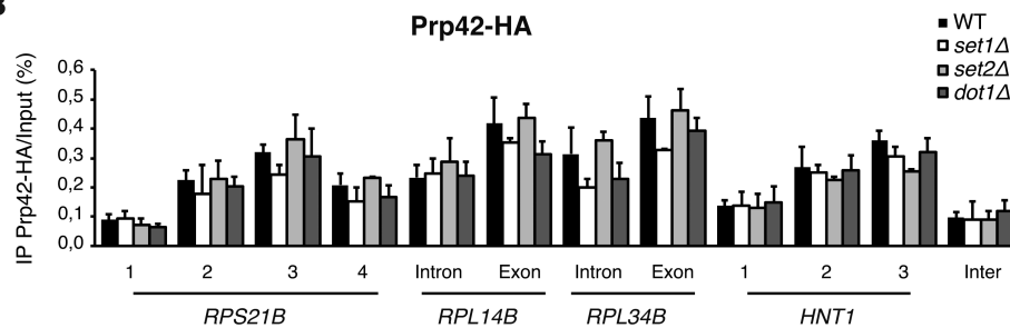
Figure 5. Loss of H2B ubiquitylation, but not Set1-, Set2- or Dot1- dependent methylation of H3, impairs recruitment of early splicing factors to transcribing genes
