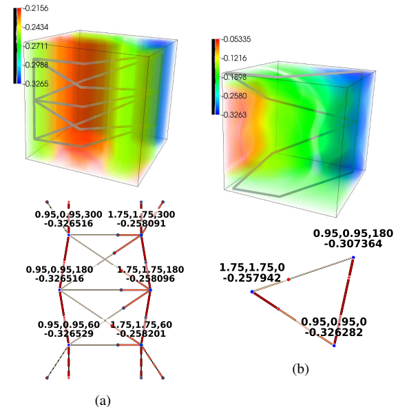
Figure 5: Three-dimensional energy function volume renderings of DFA and corresponding graphs: (a) F_{123} - M_{123} (b) F_{124} - M_{124} . As the number of dimensions grows, direct visualization becomes complicated.
