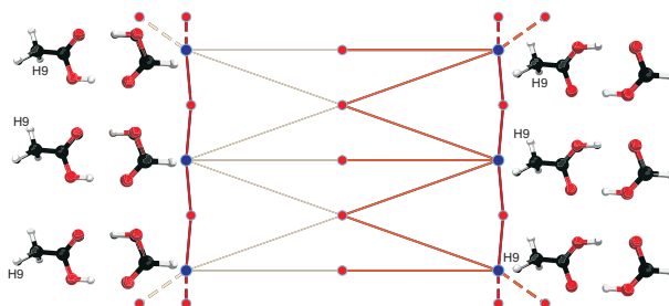
Figure 1: A 2D graph showing the topology of the 3D potential energy function of a complex of formic and acetic acids, which depends on the positions of constituting atoms. Blue and red dots represent minimum energy configurations and lowest barriers connecting neighboring minima, respectively. Edges represent the energy cost of a particular transformation, with darker and wider edges corresponding to transformations through lower barriers (more likely transformations). Two vertical branches corresponding to different positions of protons are visible on the left and right side of the graph. Energy barriers for transforming the right branch into left one are lower than for the reverse transformation.
