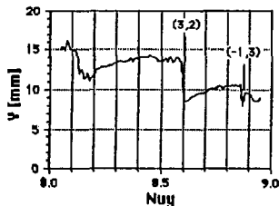
Figure 2. Vertical Tune Dependence of the Vertical Aperture
