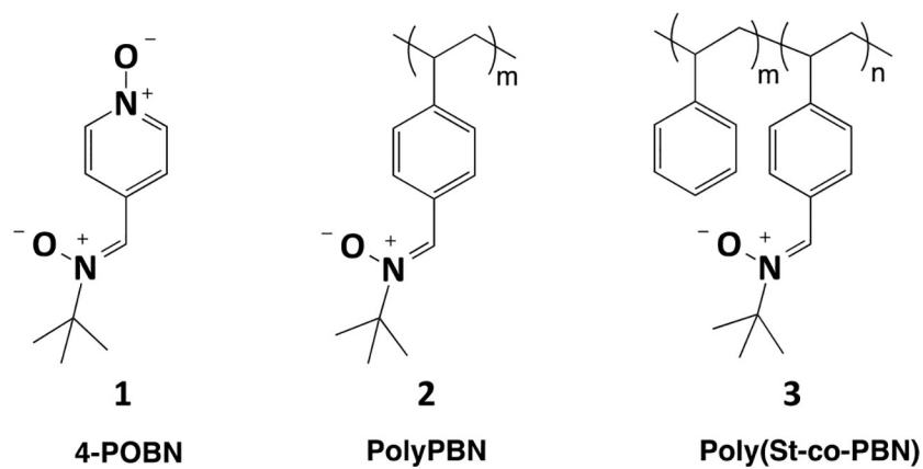
Figure 1. Spin trap 4-POBN (Watanabe) [28] and polymeric spin traps PolyPBN and Poly(St-co-PBN) (Sakakibara) [29]
