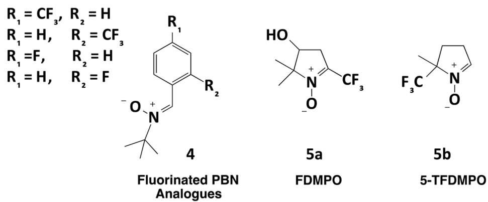
Figure 2. Fluorinated PBN spin traps 4 (Motten) [33], trifluoromethylated FDMPO 5a (Clanton) [34] and 5-TFDMPO 5b (Tordo) [36] spin traps
