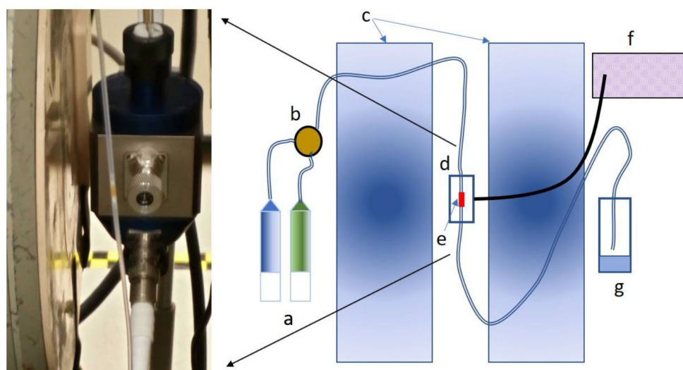
Figure 3. Generalized scheme for Flow Spin-trapping Experiments. Left side, photograph of spin trap column in front of EPR resonator. Right, instrument setup: a) Double syringe pump, b) mixer, c) EPR electromagnet, d) EPR resonator, e) spin trap column, f) UV lamp connected to resonator with flexible light pipe, g) solvent waste.
