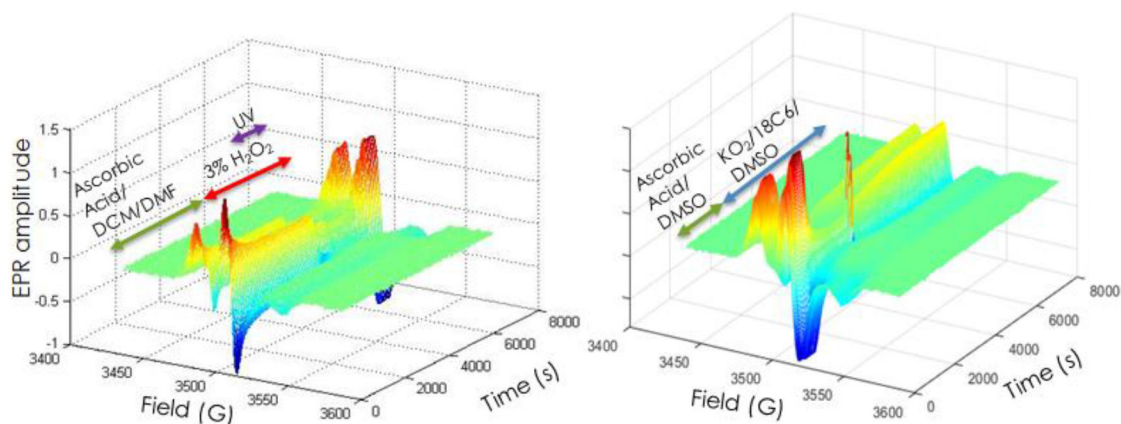
Figure 6. Flow experiments with Resin-2-HFDMPO-OH.
