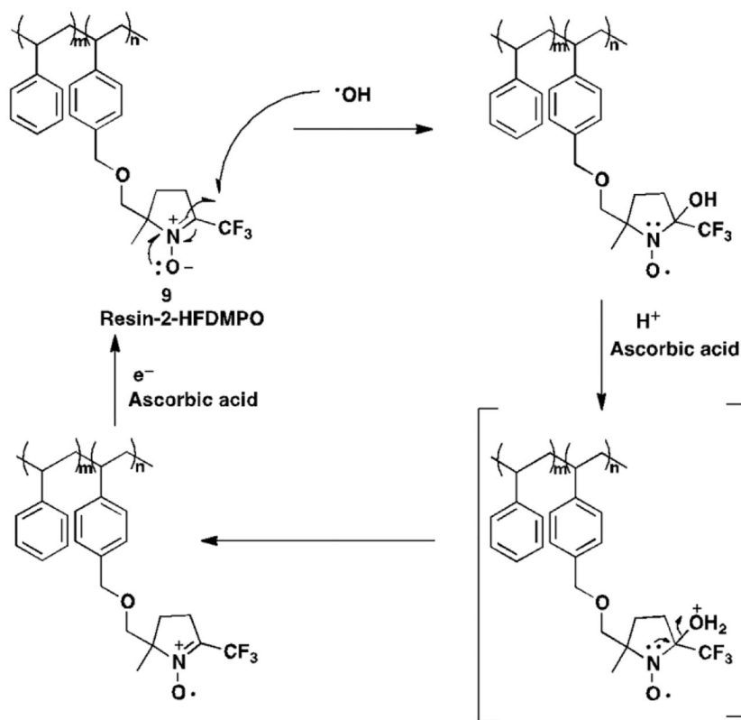
Scheme 5. Rejuvenation of Resin-2-HFDMPO 9
