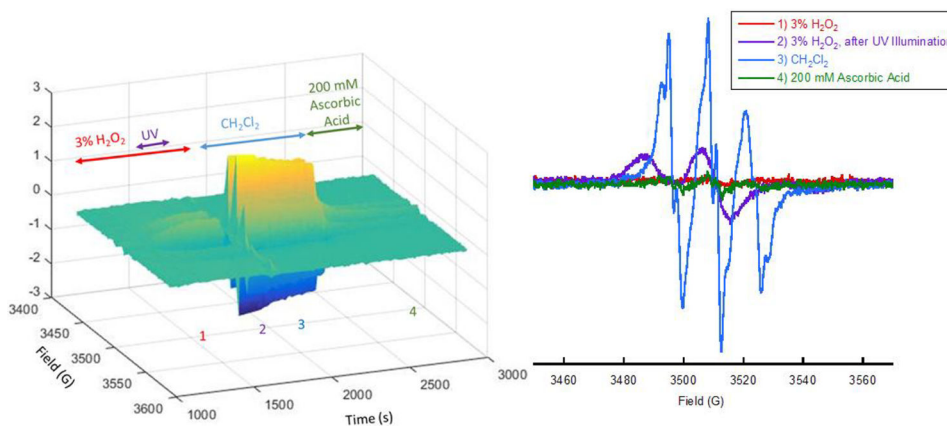
Figure 7. Flow experiments with Resin-2-PFDMPO-OH.
