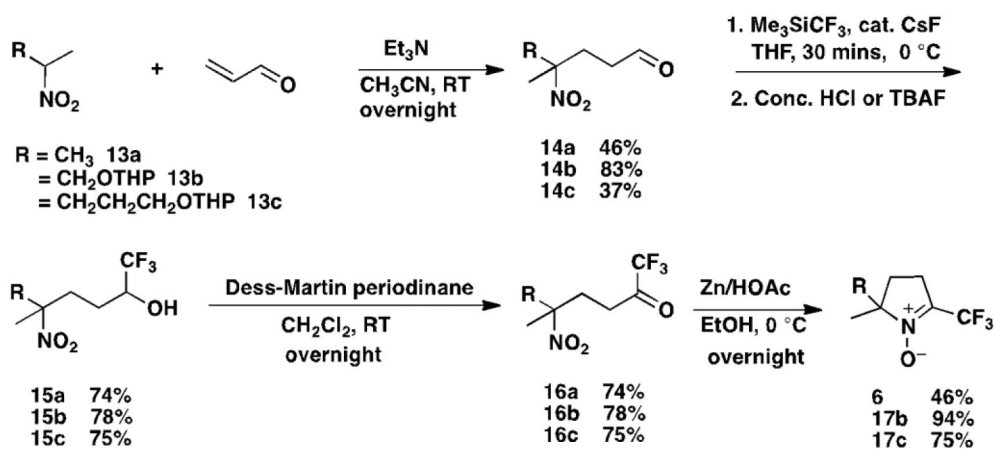
Scheme 2. Preparation of trifluoromethylated nitrones
