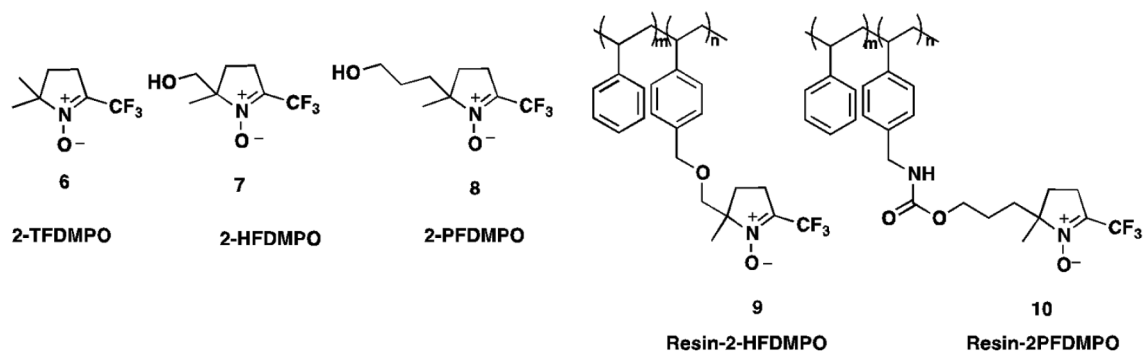
Figure 4. Monomeric and polymer-supported cyclic fluorinated nitrones investigated in this work
