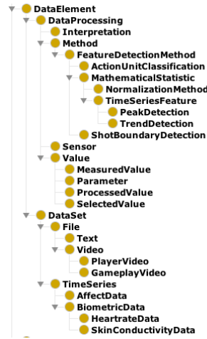
Figure 4.8: DataElement Hierarchy
