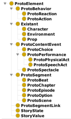
Figure 4.7: ProtoElement Hierarchy
