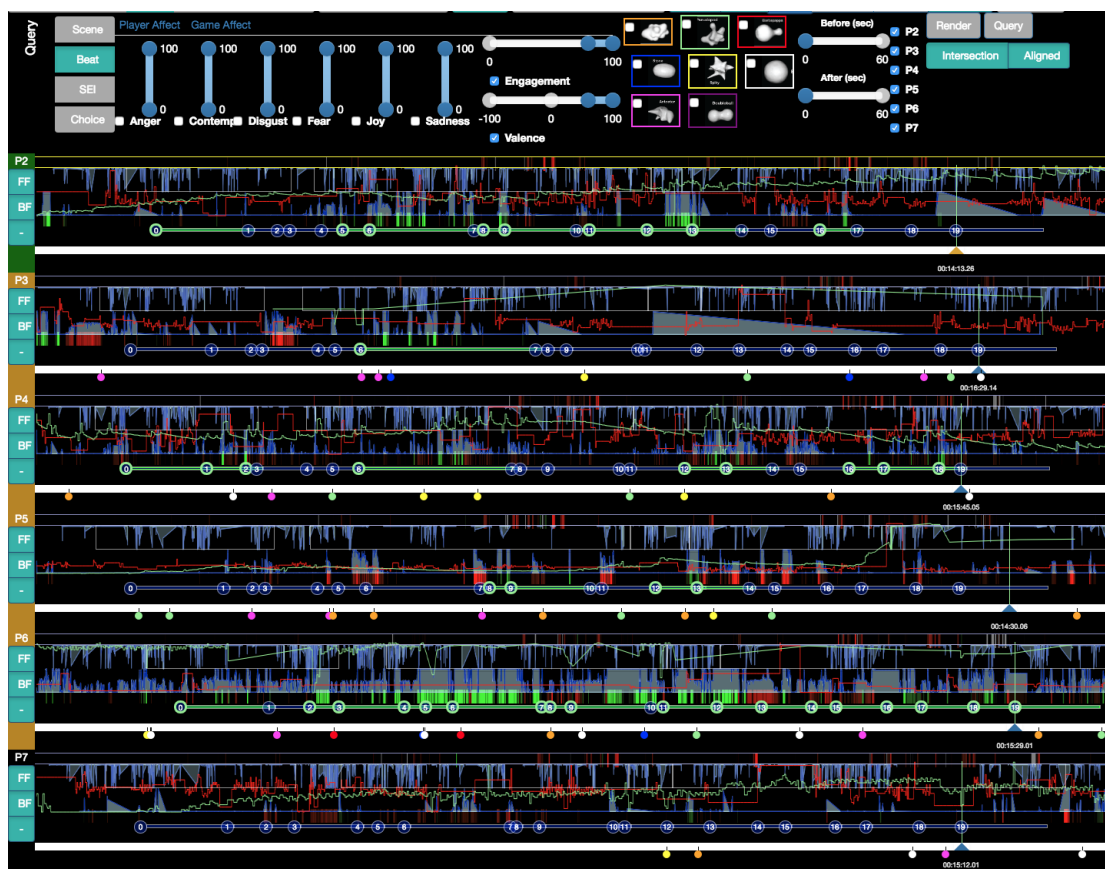
Figure 6.16: Query panel
