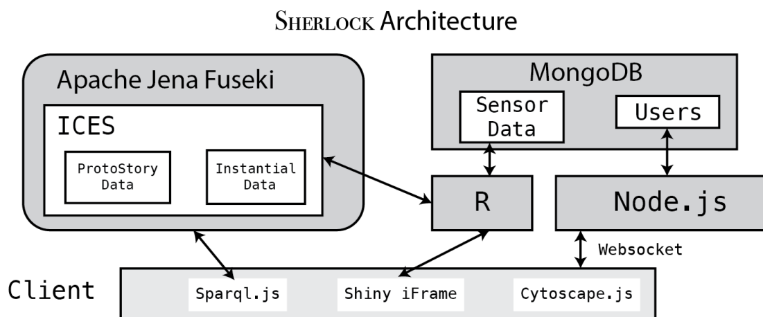
Figure 6.3: SHERLOCK architecture
