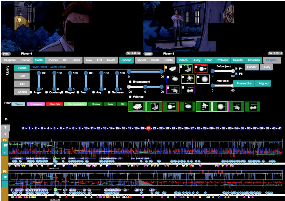
Figure 6.1: SHERLOCK user interface, v2
