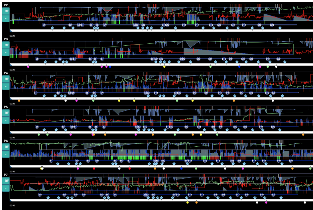
Figure 6.20: Current timelines
