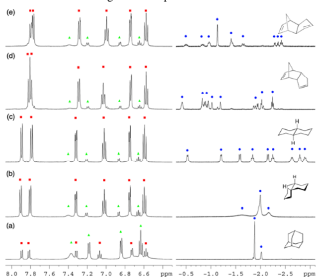
Figure 4. Aromatic (host) and upfield (bound guest) portions of the 1 H NMR spectra (500 MHz, D 2 O, pD ≈ 12) of a series of cyclodecanes bound to [Ga 4 L 6 ] 12- host 1 ; (u) bound guest; (%) bound host; ( ) free (empty) host.
