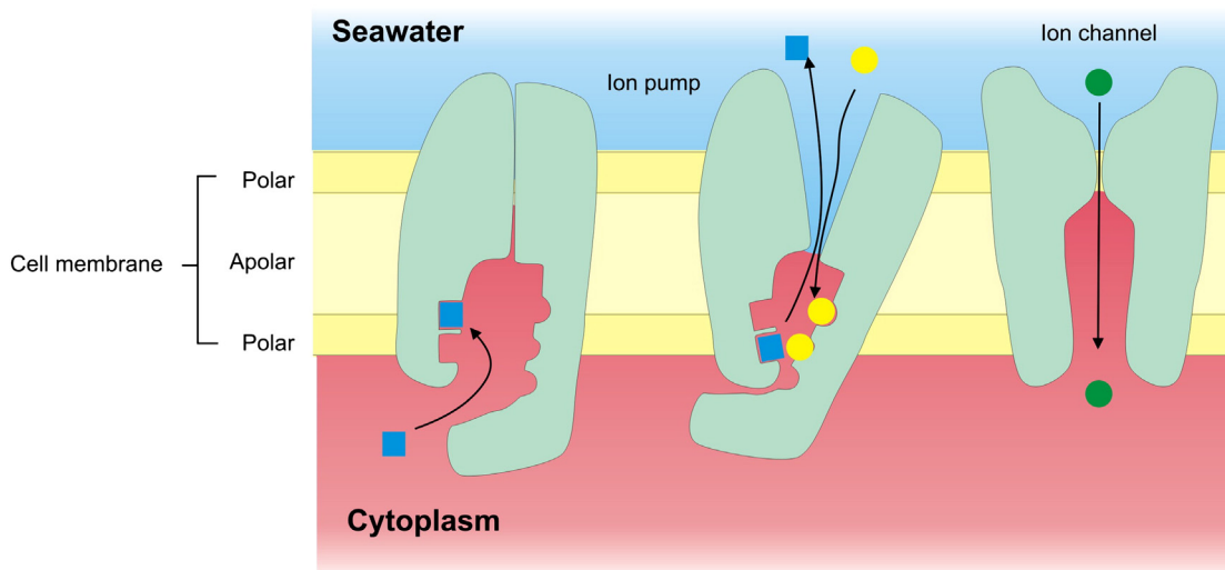
Fig. 4. Selective ion transporters. Ion pumps (left and middle) undergo structural changes that allow passage of ions from and to the binding sites. The example shown here is a simplified Na + /K + exchanger that specifically binds to Na-ions (blue squares) when in the first configurational state (left). After the structural change, affinity of the Na-binding sites decreases so that the Na-ions are released (middle). At the same time, K-ions (yellow circles) bind to their binding sites after which the pump returns to state one and releases the K + to the cytosol. Ion channels (draw after the KcsA K + channel; right) consist usually of a narrow pore allowing certain ions to pass a cell membrane down the electro-chemical gradient. Another feature of some pumps and channels is the relatively large cavity that is created by the transmembrane protein-complex (here present in the cytosol-side of the channel). This can greatly reduce the distance that the ions have to be transported. The type of Ca 2+ -transporters that are used by foraminifera are unknown, but determining their molecular structure is necessary to 1) know the extent of de-hydration during transport, 2) determine the rate of ion transport and 3) explain the selectivity for Ca 2+ against other ions (e.g. Mg 2+ ) and their fractionation (e.g. Gussone et al., 2003). (For interpretation of the references to color in this figure legend, the reader is referred to the web version of this article.)
