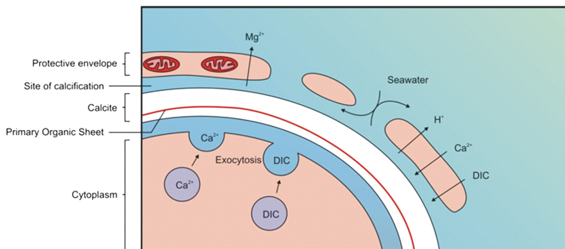
Fig. 6. Summary of the most important parts of the calcification mechanism in foraminifera, including Ca-ion transport, active Mg-removal and contribution from internal reservoirs. See text for description of the individual processes.
