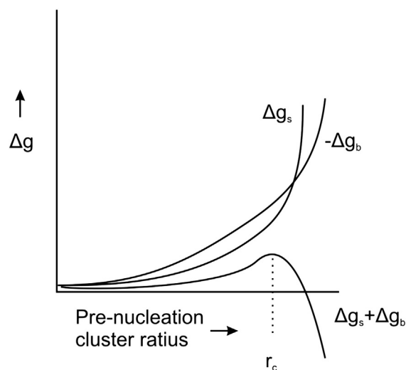
Fig. 5. Relation between free energy changes ( \Delta g ) as a function of pre-nucleation sphere ( r ), where \Delta g_s is the surface term and \Delta g_b is the bulk term. The sum of \Delta g_s and \Delta g_b is the free energy barrier that can only be overcome by the formation of a nucleation sphere with a critical size ( r_c ). Biological control over crystal nucleation is often aimed at lowering this energy barrier and can be achieved by increasing the concentrations of the solutes or the presence of an organic template.
