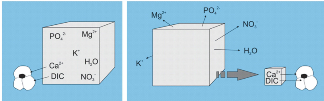
Fig. 2. Two different mechanisms to concentrate \text{Ca}^{2+} and DIC from seawater for calcification: Calcium- and bicarbonate-ions are specifically taken up from seawater (left panel), or the other ions are selectively removed, thereby increasing Ca and DIC concentrations (right panel).
