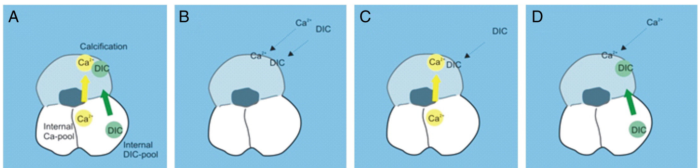
Fig. 3. Examples of possible involvement of internal reservoirs versus externally derived ions for calcification. A: \text{Ca}^{2+} and DIC are derived from internal reservoirs. B: \text{Ca}^{2+} and DIC are transported to the site of calcification without uptake and storage into reservoirs. C: DIC is taken up directly and \text{Ca}^{2+} comes from an internal reservoir. D: \text{Ca}^{2+} is taken up during chamber formation and DIC is derived from an intracellular reservoir.
