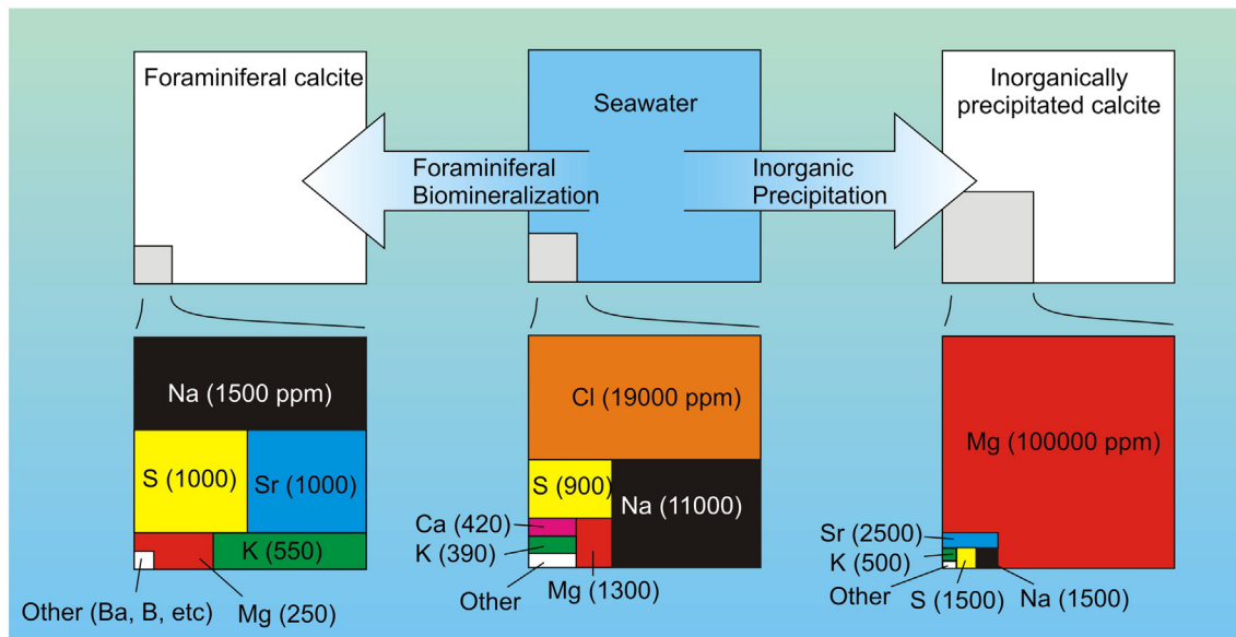
Fig. 1. Minor and trace element compositions of foraminiferal (left) and inorganically precipitated (right) calcite precipitated from seawater (middle). Concentrations are qualitative as they differ between foraminiferal species and depend on environmental conditions. Precipitation rates, ionic strength of the medium and presence of organic compounds are also known to affect partition coefficients. All values are in parts per million (ppm) and based on data in Kitano et al. (1975), Ishikawa and Ichikuni (1984), Rimstidt et al. (1998), Marriott et al. (2004), Morse et al. (2007), Tang et al. (2012) He et al. (2013) for inorganically precipitated calcium carbonates, and Lea and Boyle (1991), Rickaby and Elderfield (1999), Segev and Erez (2006), Terakado et al. (2010), Allen et al. (2011) for foraminiferal calcite composition.
