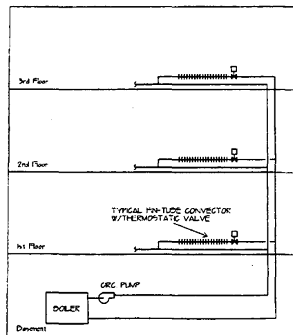
Schematic of Existing Heating System
