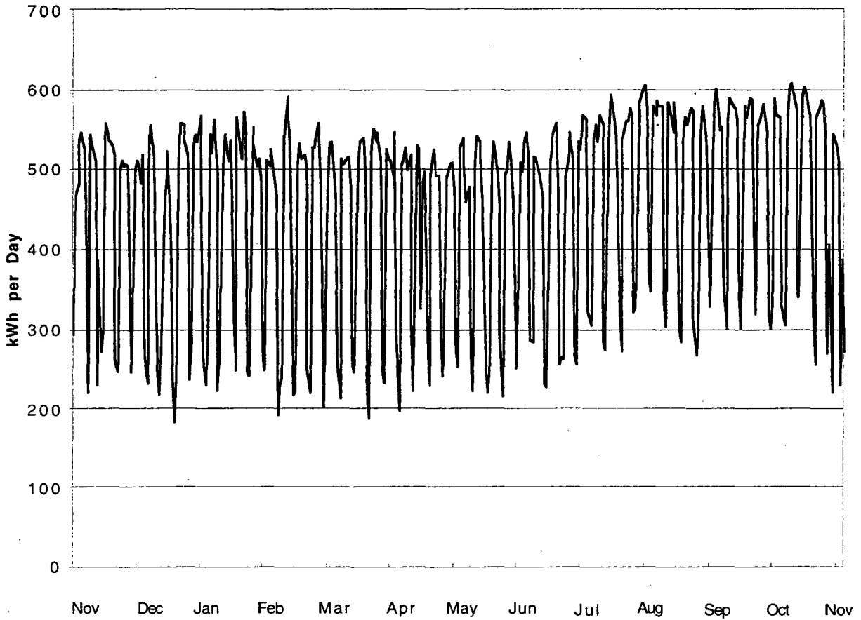
Daily Total Electricity Use for Building 102 November 1993 to November 1994
