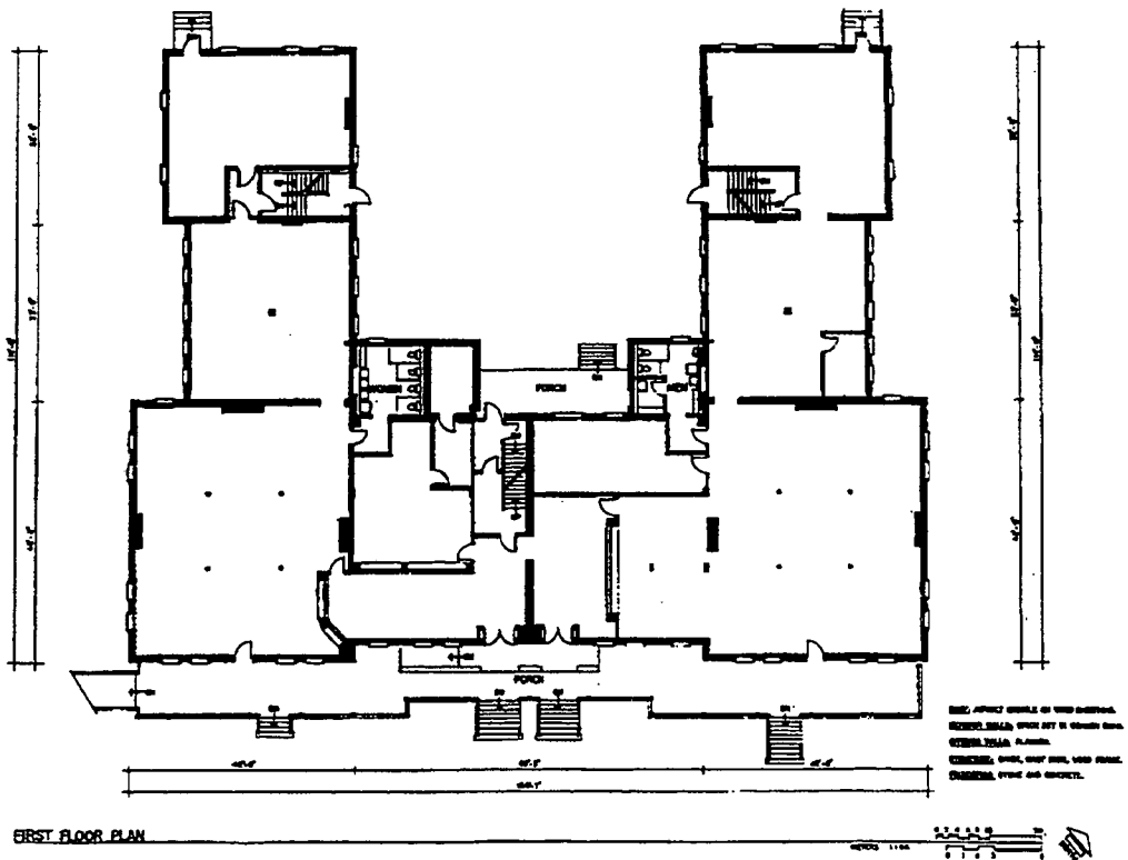
Figure 4. Building 102--First Floor Plan
