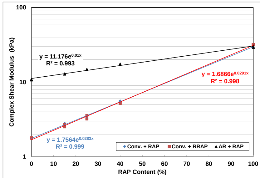
Figure 5.8: Complex shear modulus of unaged binders (64°C).
