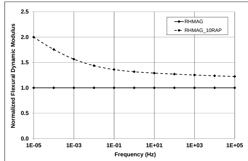
Figure 7.8: Normalized flexural modulus master curves for gap-graded RHMA mixes.
