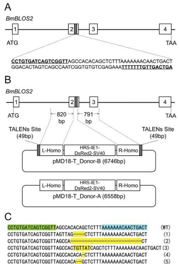
Fig. 1. Schematic representation of TALENs targeting site and donor. (A) Schematic representation of the TALENs targeting site. The thin black line represents the BmBLOS2 genome locus with the open boxes signifying the four exons. A 49bp fragment (gray box) located in exon-2 is the targeted site. The sequences in bold and underlined are the TALENs targeting sequence. A 16 bp sequence serves as a spacer between the two sites. (B) Schematic representation of the donor. A cassette expressing a DsRed2 marker (with a HR5 enhancer sequence, driven by a baculovirus IE1 promoter) was cloned into the pMD18T-simple vector. Two homologous DNA fragments (L-homo and R-homo), 820 bp and 791 bp at the 5'- and 3'-ends, respectively, of the TALEN site were cloned separately into the left and right sides of the DsRed2 cassette. The DsRed2 marker with two homologous fragments was flanked by two of the 49 bp TALENs sites (donor B). (C) Mutations detected in G 0 mutants with the oily skin phenotype (OSP). Genomic DNA was extracted from G 0 mutants with severe OSP. Fragments covering the target site were amplified and sequenced. Small deletions or insertions resulting from non-homologous end joining repair were detected. Sequences highlighted in green and blue are TALENs target sequence. Mutations are highlighted in yellow. (For interpretation of the references to colour in this figure legend, the reader is referred to the web version of this article.)
