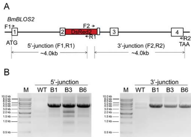
Fig. 3. Gene amplification analyses of transgene insertions in transformed silkworms. (A) Primer positions for amplification. The primer pairs F1/R1 and F2/R2 were used to amplify the 5'- and 3'-end insertion junctions, respectively. (B) The diagnostic DNA fragments for 5'- and 3'-end junctions were detected in brood-1 (B1), brood-3 (B3) and brood-6 (B6).
