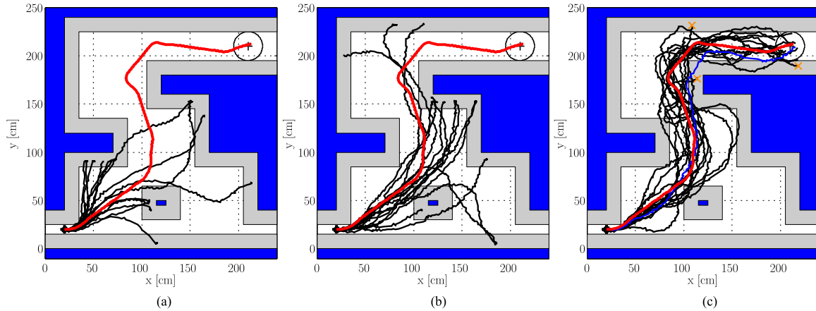
Fig. 7. Experimental results with the OctoRoACH. The desired path is marked with a thick curve in all cases. (a) Open-loop implementation of the desired path. (b) Closed-loop response of the system using the reported path tracking controller. (c) The combination of local path tracking control with the prediction phase. The path is refined every two primitives using the RRT; Fig. 9 shows this process for one sample path, highlighted here in blue (color version).
