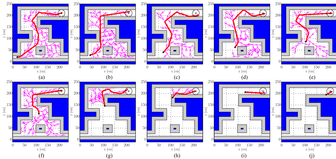
Fig. 9. Illustration of the two-stage path tracking control and prediction scheme when applied to the physical robot. (a) Initial path (thick curve) generated by the RRT (cf. Fig. 3), is updated after the first two primitives of the plan have been executed with the local path tracking controller being active. (b) Updated path (thick curve) is followed for the first two primitives, and updated again by the solver. (c)–(j) Process repeats until the desired state is reached.
