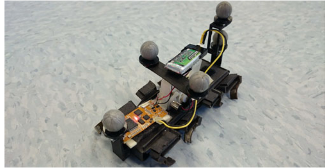
Fig. 1. The miniature eight-legged OctoRoACH robot [6].
