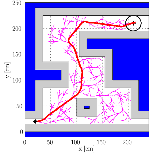
Fig. 3. RRT is outlined in thin curves, whereas the desired path is marked with a thick curve. Obstacles (shown in dark shading) are artificially augmented (lightly shaded regions) to account for platform volume.
