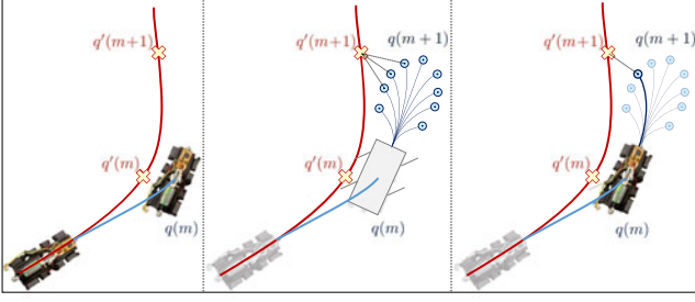
Fig. 4. Pictorial representation of the tracking controller's function. Primed and nonprimed quantities denote desired and actual states at the beginning of step m and m + 1 , respectively.
