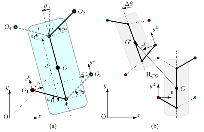
Fig. 2. (a) The SFM model. Two pairs of rigid legs become active in turns, forming two four-bar linkages, \{O_1A, AB, BO_2\} and \{O_3A, AB, BO_4\} . d is the distance between the two hip-point joints A and B , l denotes the leg length, and G is its geometric center. (b) Pictorial representation of state propagation—the active pair is marked with thick solid lines.
