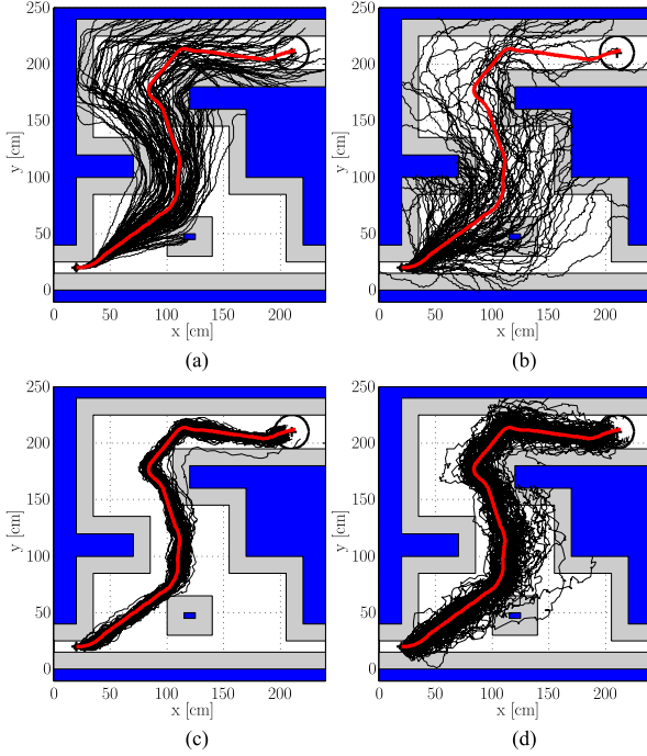
Fig. 5. Simulated response of the system commanded to follow a desired path (thick red curve), when uncertainty affects its state at the end of every step. (a) Open-loop response of the system with low magnitude of infused uncertainty scores a 10% success rate. (b) As the magnitude of the infused uncertainty grows, the success rate reduces to 2%. (c) Closed-loop response of the system using the reported path tracking controller. When the magnitude of the infused uncertainty is low, the controller enables the system to follow the desired path, scoring a 100% success rate. (d) As the magnitude of the infused uncertainty grows, the system may exit the region of attraction of the controller and lose track of the desired path; the success rate reduces to 85%. (a) \sigma_x = \sigma_y = 0.25 cm, \sigma_\theta = 2^\circ . (b) \sigma_x = \sigma_y = 0.75 cm, \sigma_\theta = 5^\circ . (c) \sigma_x = \sigma_y = 1 cm, \sigma_\theta = 5^\circ . (d) \sigma_x = \sigma_y = 2 cm, \sigma_\theta = 10^\circ .
