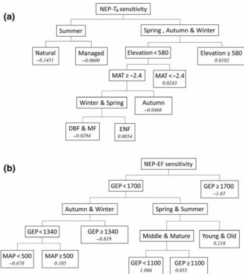
FIGURE 8 Classification and Regression Tree (CART) analysis on seasonal net ecosystem productivity (NEP) sensitivities to air temperature ( T_a , a) ( \text{g C m}^{-2} \text{ day}^{-1} \text{ }^\circ\text{C}^{-1} ) and evaporative fraction (EF, b) ( \text{g C m}^{-2} \text{ day}^{-1} ) anomalies. The CART ranks the explanatory variables based on predictive power with the variable that explains the highest amount of variance in the dependent variable on top. The explanatory variables were selected from Table 2. Minimum node size = 15. DBF, broadleaved deciduous forests; ENF, evergreen needle-leaved forests; GEP, gross ecosystem productivity; MAP, mean annual precipitation; MAT, mean annual temperature; MF, mixed forests
