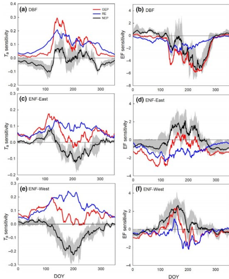
FIGURE 2 Daily sensitivities of forest carbon fluxes to air temperature ( T_a , \text{g C m}^{-2} \text{ day}^{-1} \text{ }^\circ\text{C}^{-1} ) and dryness represented by evaporative fraction (EF, \text{g C m}^{-2} \text{ day}^{-1} ) anomalies. (a) T_a sensitivity in Deciduous Broadleaf Forest (DBF), (b) EF sensitivity in DBF, (c) T_a sensitivity in evergreen needle-leaf forest (ENF) in eastern sites, (d) EF sensitivity in ENF in eastern sites, (e) T_a sensitivity in ENF in western sites, and (f) EF sensitivity in ENF in western sites. Curves show the mean sensitivity in the 15 day moving-windows. The shaded area shows the 25% and 75% percentile of the net ecosystem productivity sensitivities among sites
