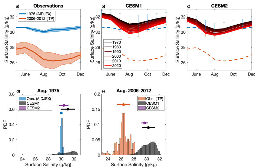
Figure 2. (a) Surface salinity from 1975 AIDJEX data (blue) and 2006-2012 ITP data (red). Solid line indicates May-December average and shading indicates standard deviation. Blue and red error bars indicate one standard deviation over all grid points and simulations in 1975 and 2006-2012, respectively. (b-c) Simulated 1970-2020 ensemble-mean surface salinity from (b) CESM1 and (c) CESM2. Distribution of August surface salinity in (d) 1975 and (e) 2006-2012 from each observation in 1975 (blue) and 2006-2012 (red), and from each grid point of each CESM1 (black) and CESM2 (purple) simulation of 1975 and 2006-2012 (distribution for CESM2 not shown). Solid dots and lines indicate mean and one standard deviation. AIDJEX (blue) and ITP (red) observations are repeated in panels (b,c).
