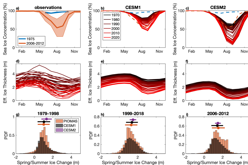
Figure 3. (a) Observed sea ice concentration co-located to 1975 AIDJEX data (blue) and 2006-2012 ITP data (red). Solid line indicates monthly mean, and shading indicates standard deviation. (b-c) Simulated 1970-2020 ensemble-mean sea ice concentration from (b) CESM1 and (c) CESM2. (d-f) Effective sea ice thickness from (d) PIOMAS and (e,f) CESM1,2 ensemble mean. (g-i) Distribution of the seasonal change of the effective sea ice thickness between May and September during (g) 1979-1998, (h) 1999-2018, and (i) 2006-2012 using all grid points from PIOMAS (red), and from each CESM1 (black) and CESM2 (purple) simulation (distribution for CESM2 not shown). Solid dots and lines indicate the mean and standard deviation. AIDJEX (blue) and ITP (red) observations are repeated in panels (b,c).
