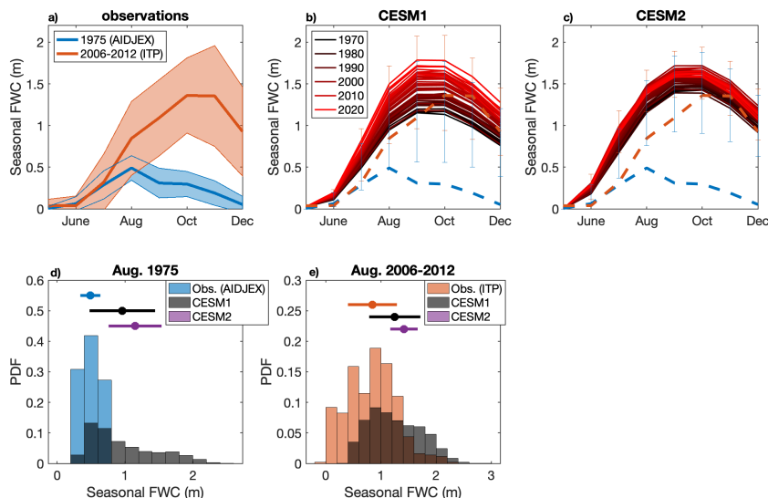
Figure 4. (a) Observed sFWC from 1975 AIDJEX data (blue) and 2006-2012 ITP data (red). Solid line indicates monthly-mean and shading indicates one standard deviation. (b-c) Simulated 1970-2020 ensemble-mean sFWC from (b) CESM1 and (c) CESM2. Blue and red error bars indicate one standard deviation over all grid points and simulations in 1975 and 2006-2012, respectively. (d-e) Distribution of August sFWC in (d) 1975 and (e) 2006-2012 from each observation in 1975 (blue) and 2006-2012 (red), and from each grid point of each CESM1 (black) and CESM2 (purple) simulation of 1975 and 2006-2012 (distribution for CESM2 not shown). Solid dots and lines indicate mean and one standard deviation. AIDJEX (blue) and ITP (red) observations are repeated in panels (b,c).
