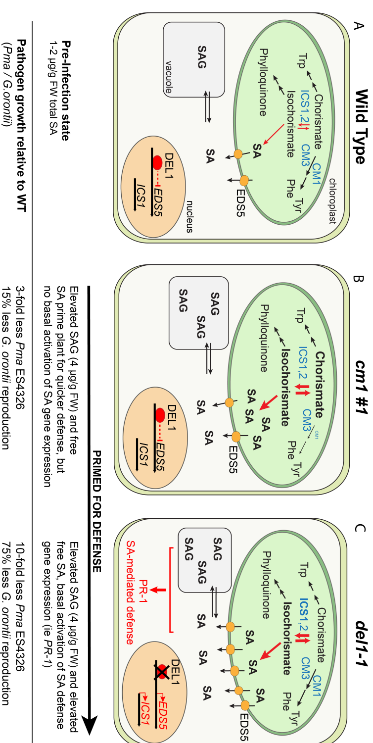
Figure 4.1 Model of basal SA accumulation and signaling in cm1 #1 and del1
